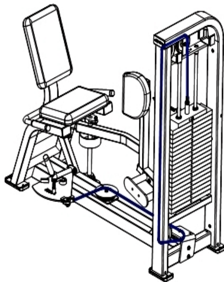
7423611 Stack cable
