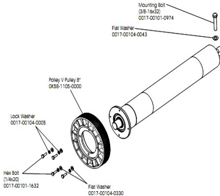
Front Roller Assembly – AK58-00066-0000
