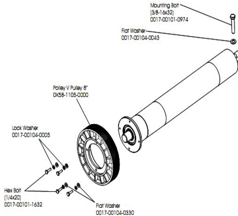
Front Roller Assembly – AK58-00067-0000
