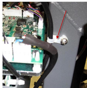
ROUTE LEFT ACTUATOR MOTOR CABLE AS SHOWN. POSITION CABLE TIE 101416-001 AS SHOWN.
