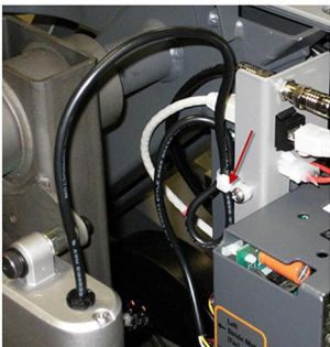
ROUTE RIGHT ACTUATOR MOTOR CABLE AS SHOWN. POSITION CABLE TIE 101416-001 AS SHOWN.
