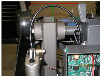
HEIGHT OF CABLE FROM ACTUATOR MOTOR SHOULD BE EVEN WITH BRACKET ON FRAME AS SHOWN IN ABOVE PICTURE
