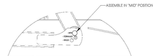
DETAIL B SCALE 1 : 2
