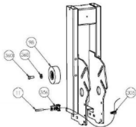
DETAIL IDLER PULLEY, SWITCH, CLAMP PLACEMENT
