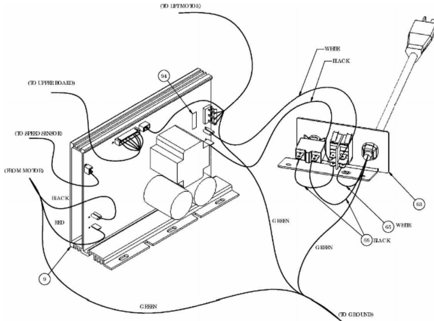
WIRING DIAGRAM
