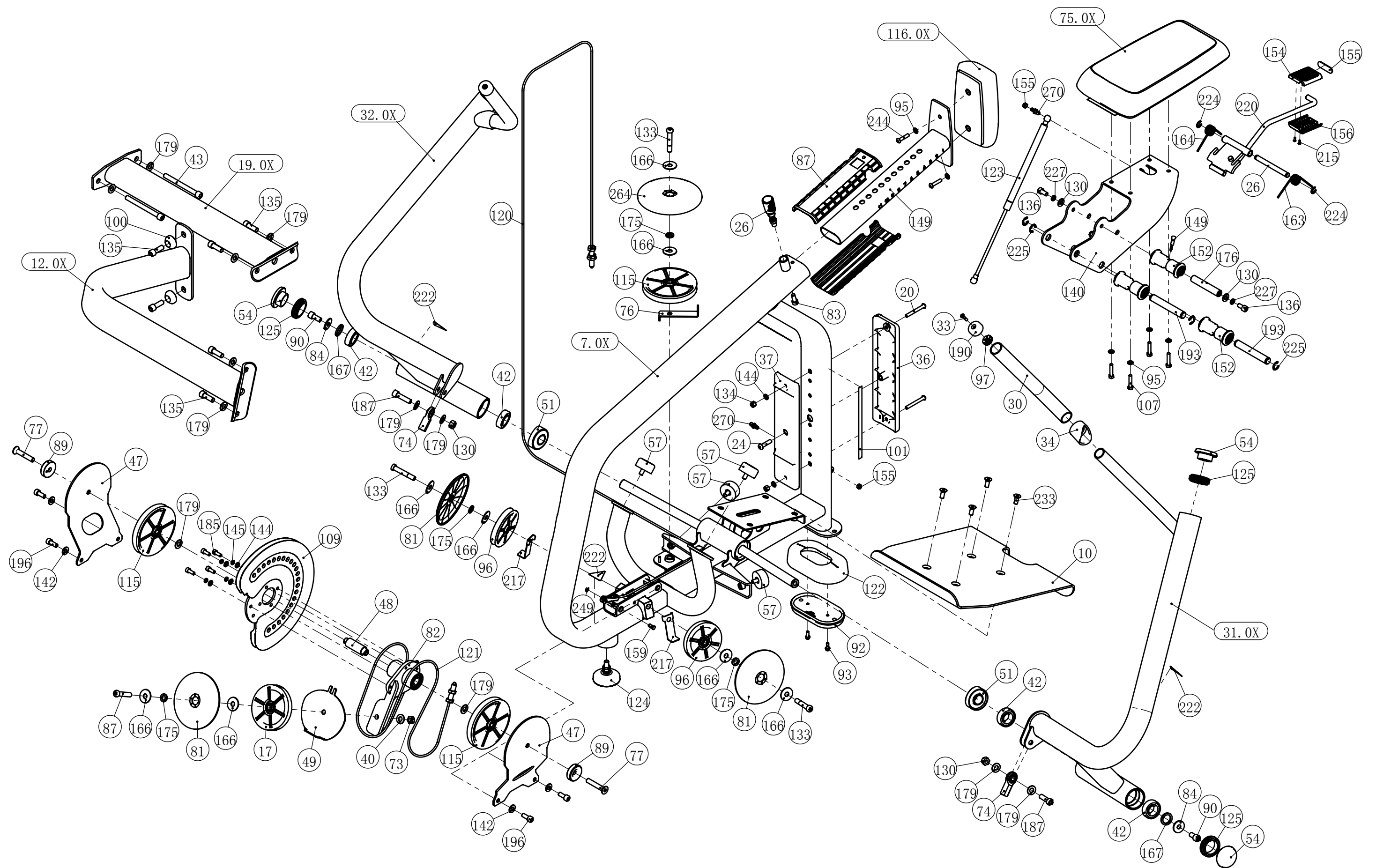
Description: Seated Row Exploded View: CW39821-101 REV C
