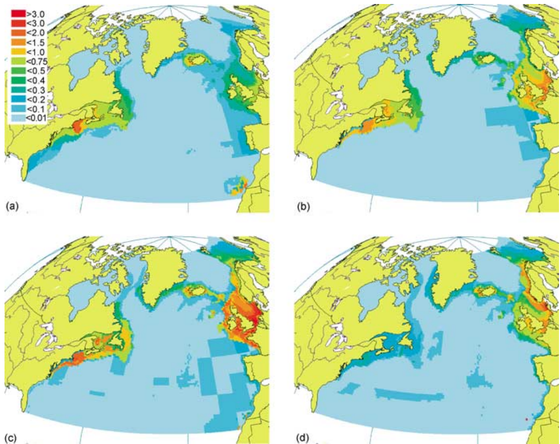
Figure 9 Predicted catch distributions of high-trophic level fishes in the North Atlantic in (a) 1900 (b) 1950 (c) 1975 and (d) 1999. The catches are based on FAO catch data information supplemented with other sources using a rule-based system for spatial allocation (Watson et al. 2001), and are here extracted for fish with trophic level \geq 3.75 (based on trophic levels in FishBase). Units for the legend are tonnes \text{km}^{-2} \text{year}^{-1} .
