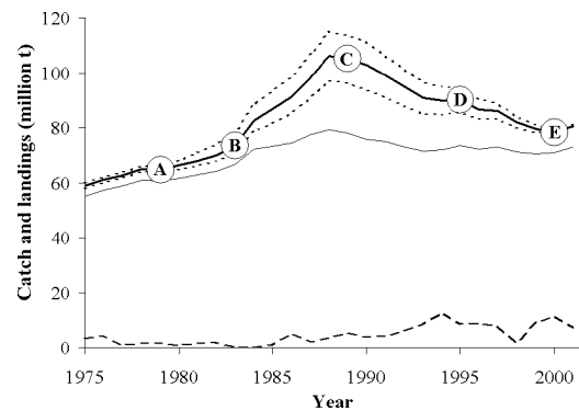
Figure 2 Landing and discarding trends in global marine fisheries. The graph shows fisheries landings for 1975 to 2001 (thin black line), as reported by FAO, but excluding catches over-reported by China (Watson and Pauly 2001), the highly variable Peruvian anchoveta ( Engraulis ringens , dashed line) and discards. These landings have been declining by about 0.4 million t per year since the late 1980s (Watson and Pauly 2001). Total catches (thick black line), i.e., catches = reported landings + estimated mean discards, suggest a much stronger decline of about 2.3 million t per year. The same summation using minimum and maximum range estimates for discards are also shown (dotted lines). Fisheries discards are interpolated between five point estimates: A 1979 (Anonymous 1982); B 1983 (Saila 1983); C 1989 (Alverson et al. 1994); D 1995 (Alverson 2005) and E 2000 (Kelleher 2004).
