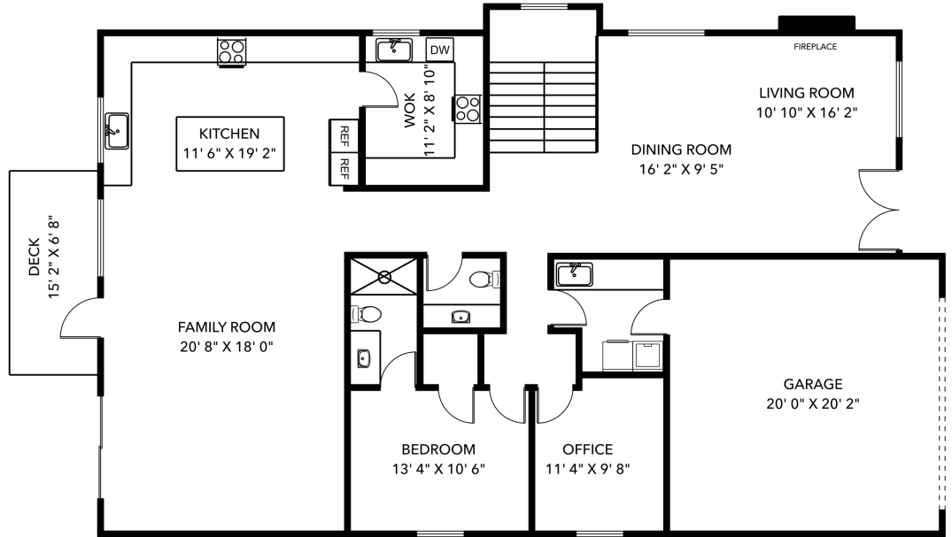
MAIN LEVEL 1936 SF
