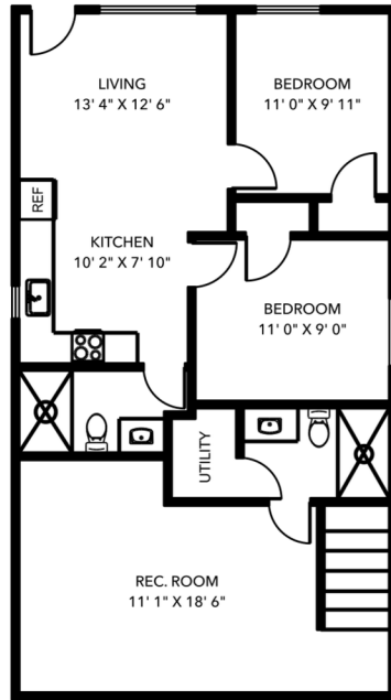
Basement 995 sq.ft.
