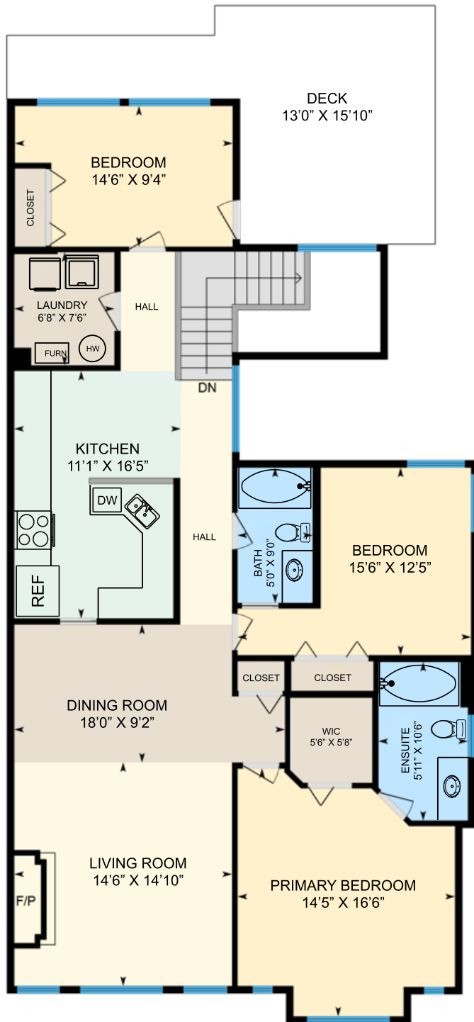
Main Level 1503 sf
