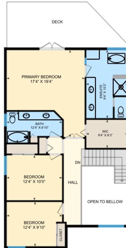
Upper Level 1061 sq.ft.
