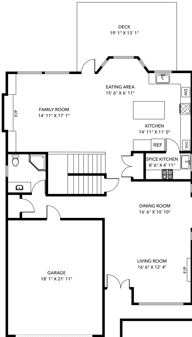
MAIN LEVEL 1331 SQ.FT.
