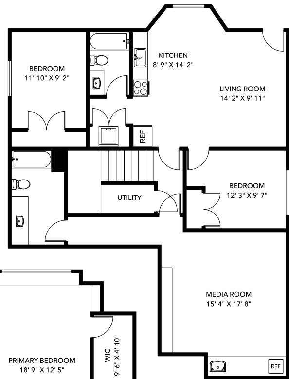
LOWER LEVEL 1312 SQ.FT.
