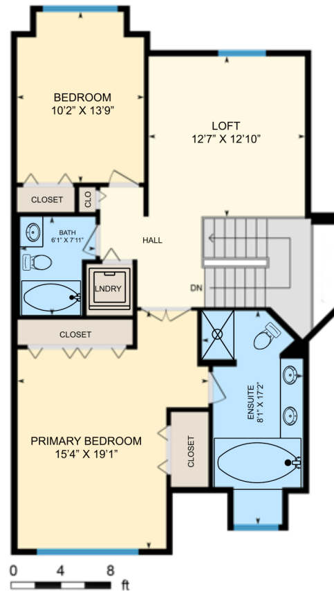
UPPER LEVEL 958 sq.ft.
