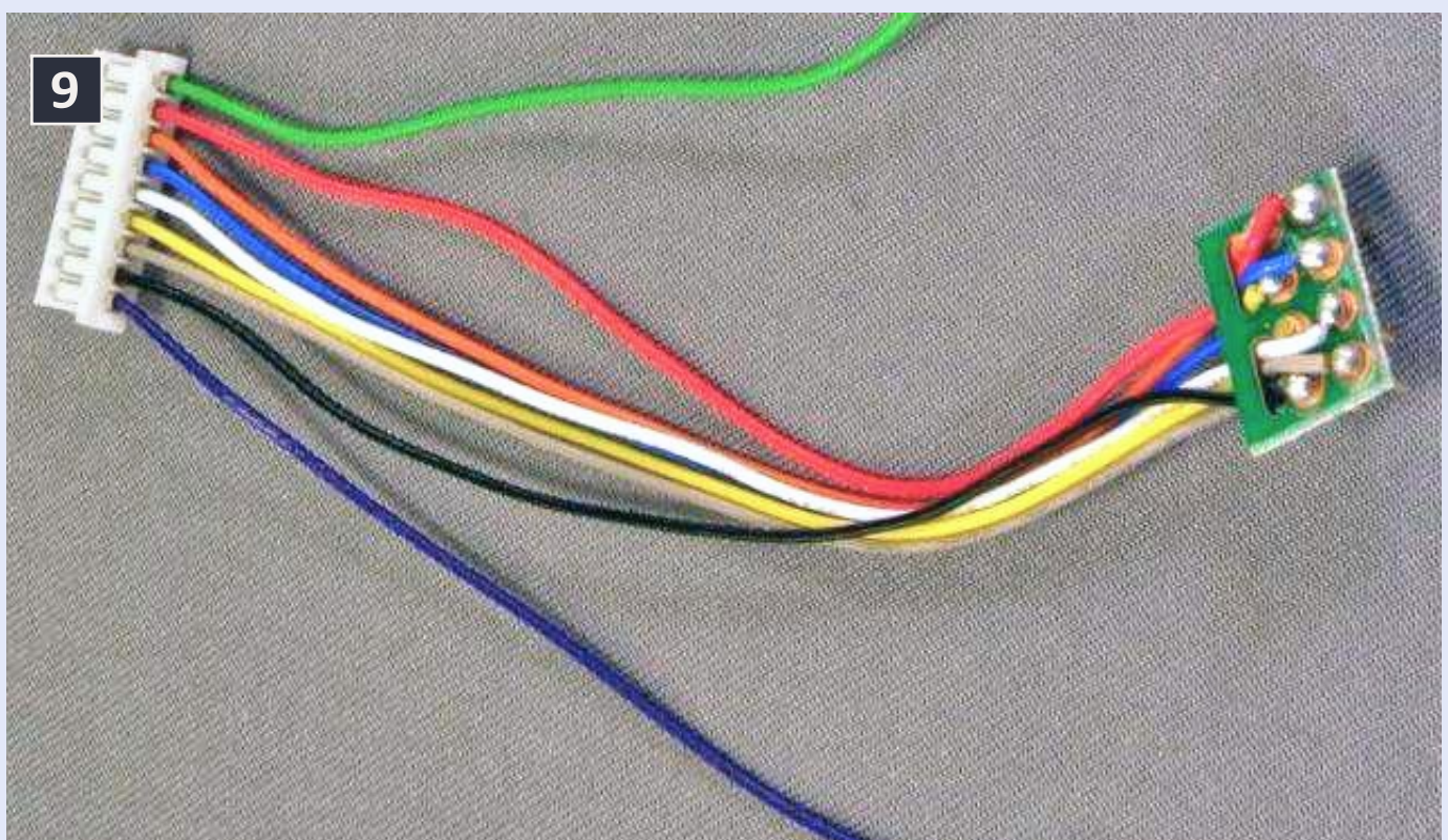
9: JST to NEM-652 conversion harness (9-pin to 8-pin).
