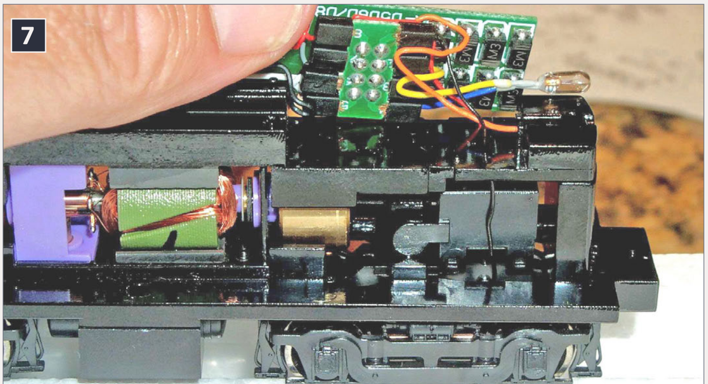
7: Life-Like Proto 2000 S1 (HO-scale) light board and DCC socket.
