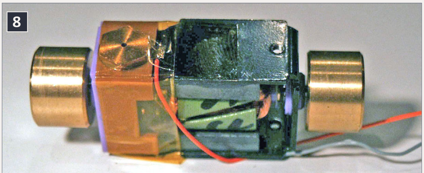
8: Life-Like Proto 2000 S1 (HO-scale) motor after insulation – bottom view.
