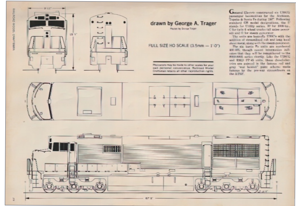
4. I used this scale drawing from the February 1970 issue of Railroad Model Craftsman as the starting point for my 3D CAD model. Copyright Railroad Model Craftsman, used with permission.
