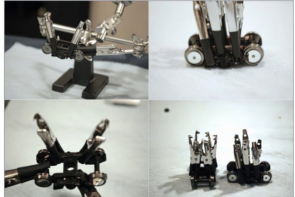
10. Gluing the electrical wipers to the trucks with the helping hands clamps.
