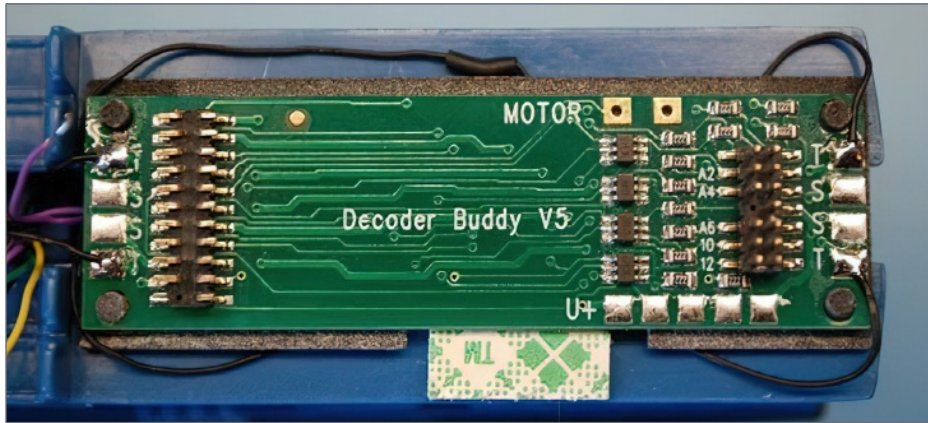
21. Decoder Buddy with soldered truck feed wires.
