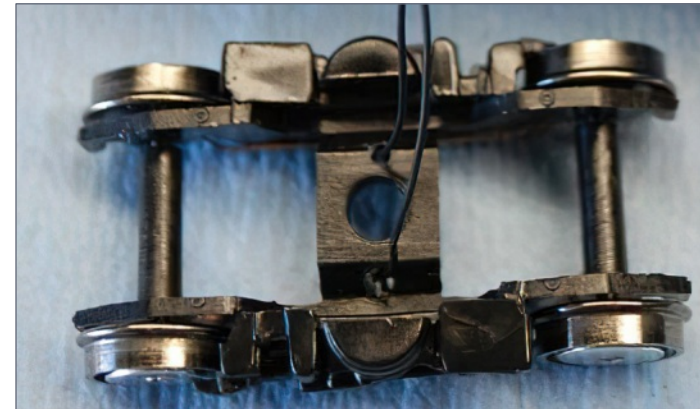
5. Truck hole positions with electrical wire pickups shown.
