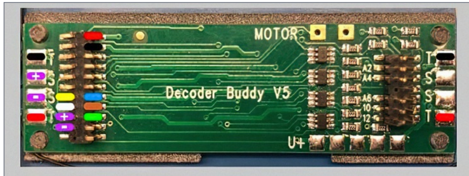
22. Solder points for the SoundCar decoder wires.
