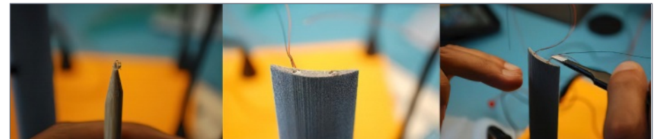
35. With the fiber optic threaded into the holes in the interior roof casting, then glue LEDs to the ends with clear Gorilla glue as shown here. Use a pencil tip to apply the glue, then attach the SMD LEDs.
