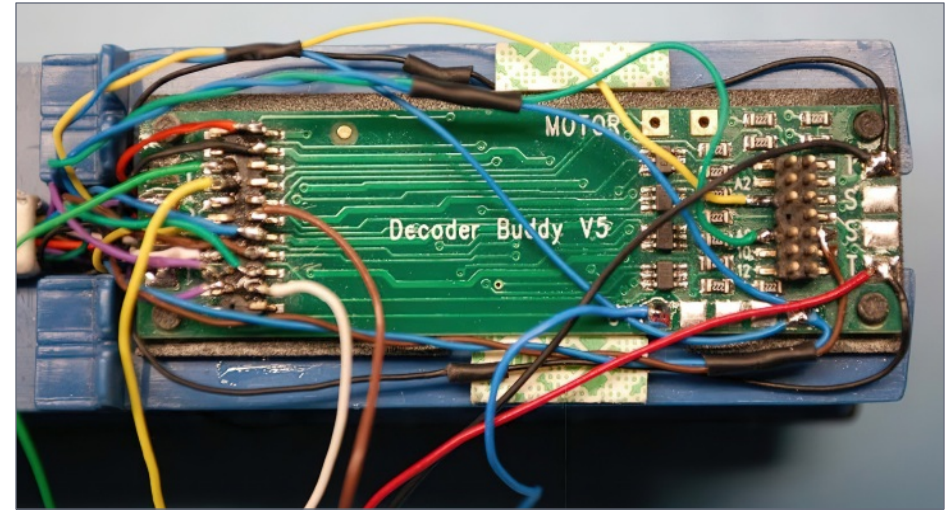
50. SoundCar #2 decoder wires soldered to Decoder Buddy main board.
