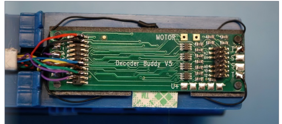
23. SoundCar wires soldered to Decoder Buddy. The jumper wires shown in [20] were not yet soldered in place. In hindsight, I recommend you add the jumper wires shown in [20] first.
