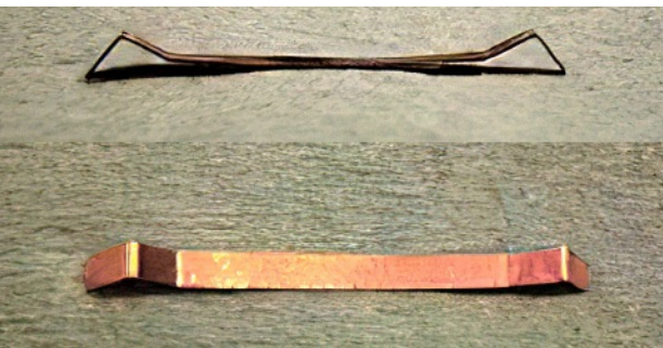
9. Electrical pickup bend geometry (I bent them before soldering in this photo).
