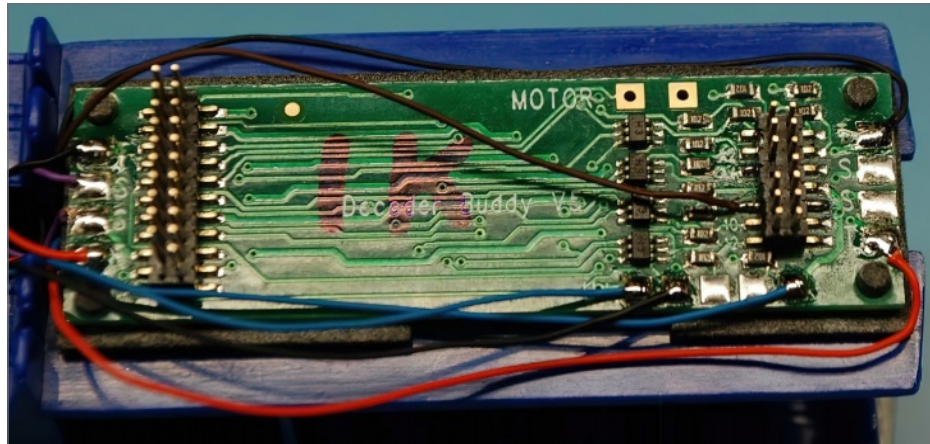
25. Decoder Buddy with wires soldered as per [24].
