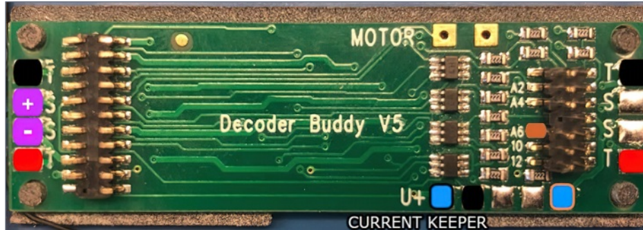
24. Soldering points when using an ESU decoder. Use A6 (AUX6) for lower-level lighting.
