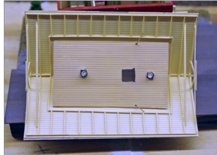
4. The removable roof includes a ceiling and LED lighting for the interior. The brass wires extending from the ceiling carry power for the lights.
