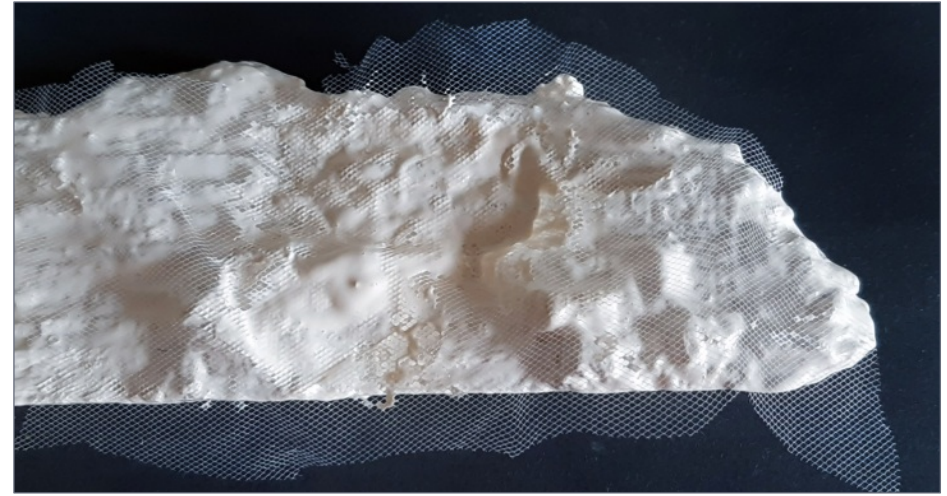
16. Tulle from a fabric store is embedded in the latex and more rubber is painted on. This makes the finished mold almost indestructible.
