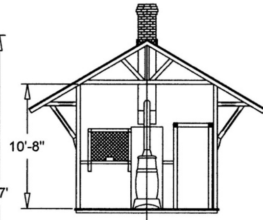
SECTION THROUGH INTERIOR
