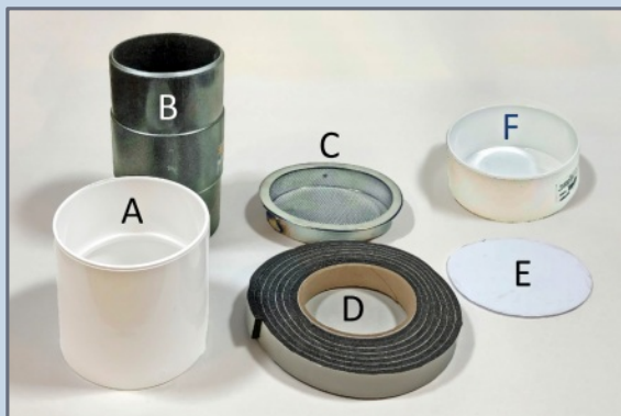
1a. Parts to make the shell for this jumbo static grass applicator in the US or Canada. See text for part descriptions.
