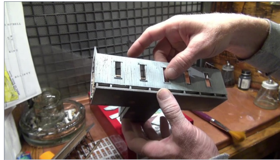
13. After spray-painting the shell over the rubber cement, Ken distresses the paint by rubbing his thumb over it, exposing the darker paint underneath for a peeling paint effect.
