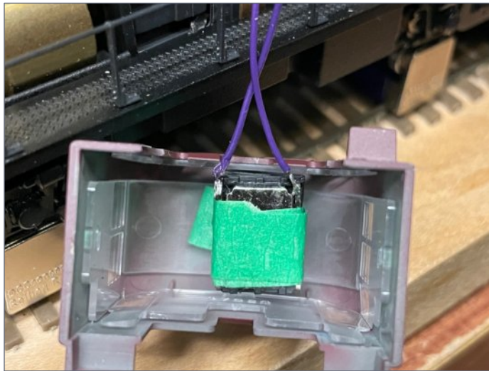
11. ESU Sugarcube speaker inside the cab roof. The green tape is temporary.
