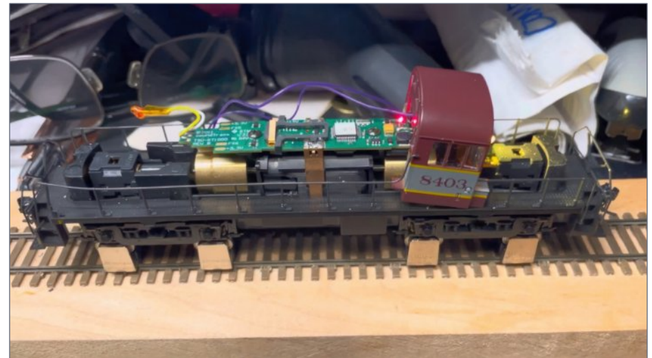
10. ESU Sugarcube 50321 speaker in the cab. To hear how this one sounds on a video recording, go here: youtu.be/Ap44BPPJf10
