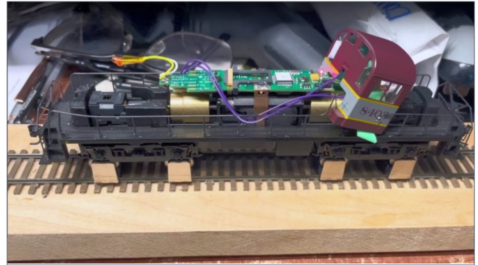
9. Two Soundtraxx Mini Cube 3 speakers in the cab. To hear how this one sounds on a video recording, go here: youtu.be/UosmdVkRj68
