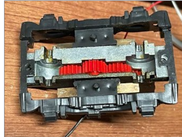
25. With the bottom cover removed, the geared wheelsets came out, and then the truck side frame piece came off. I made note of the order so I could reverse it for reassembly. The frame must go on first, since the wheel wipers will block
