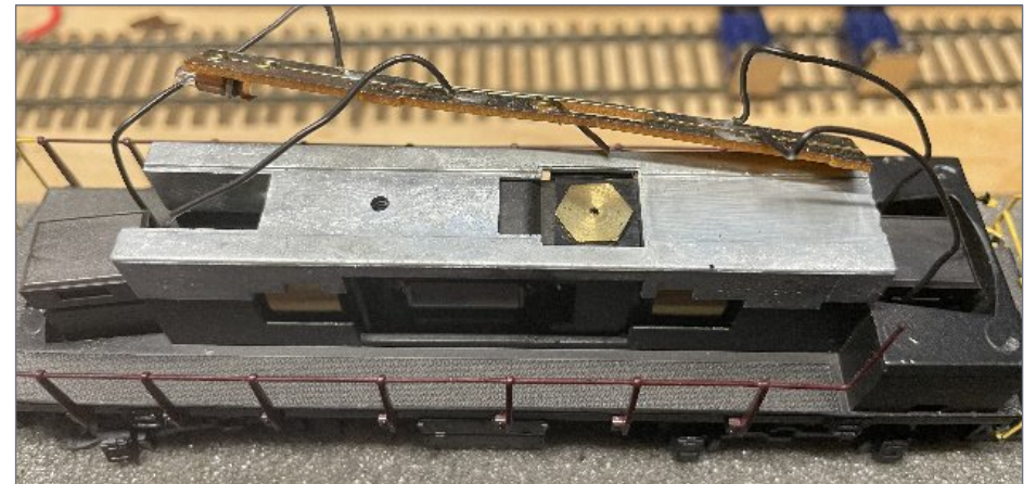
15. Circuit board removed with wiring intact.
