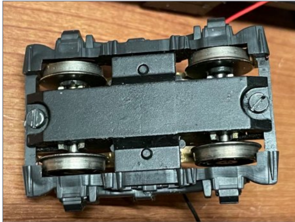
24. The two screws on the bottom of the truck hold the cover and side frames in place.
