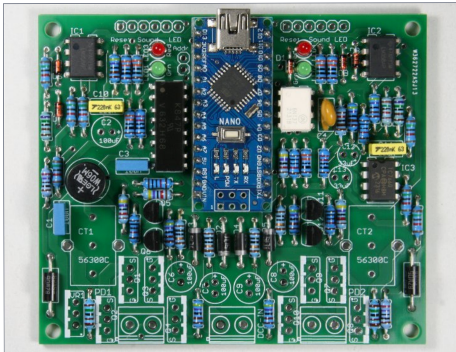
5. Second stage of Dual Power Breaker assembly.
