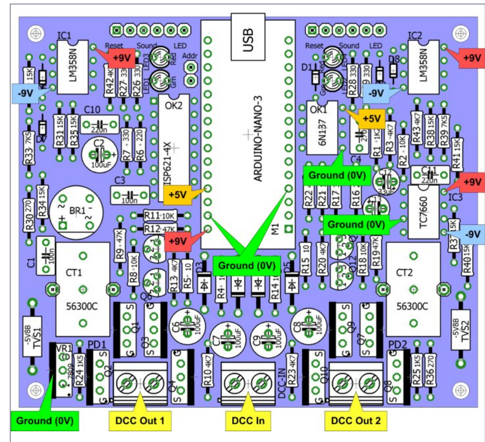
16. Check the DPB integrated circuits for correct voltages.
