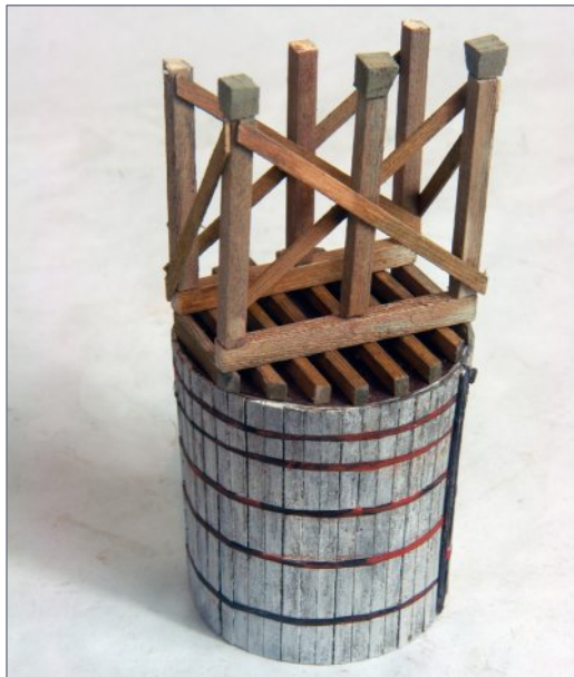
20. Finishing up the tank stand. No one will ever notice the missing concrete footings on the rear legs.
