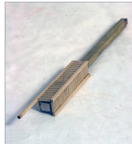
22. Installing the corner posts for the water column. I kept a short length of the core for easy attachment between the legs of the tank base.
