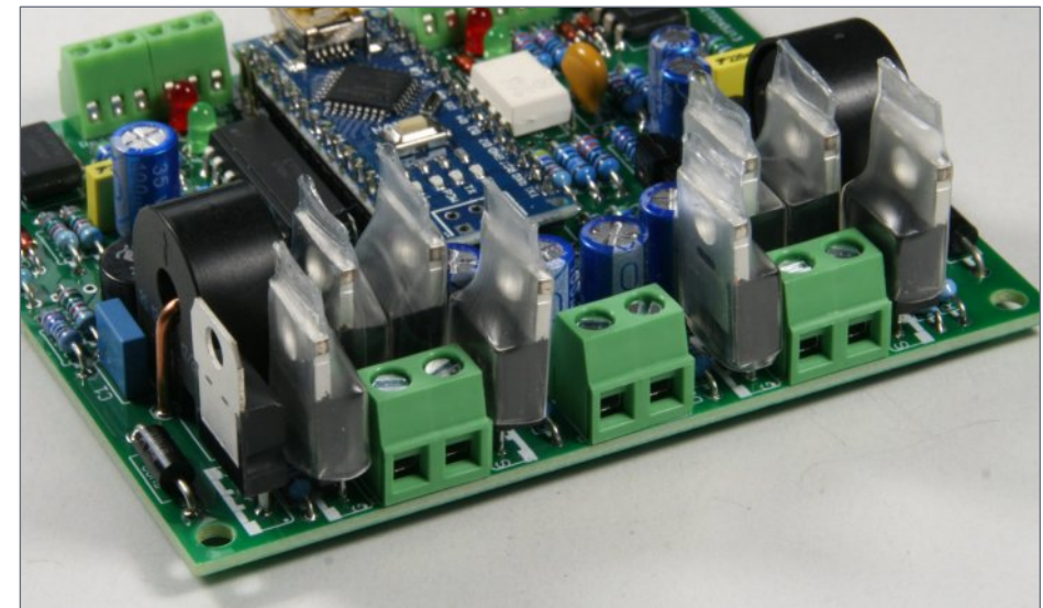
15. Insulation by adding heat-shrink tubing to the power MOSFETs. The tab of the voltage regulator (lower left) is at ground (0V), so it does not require insulation.
