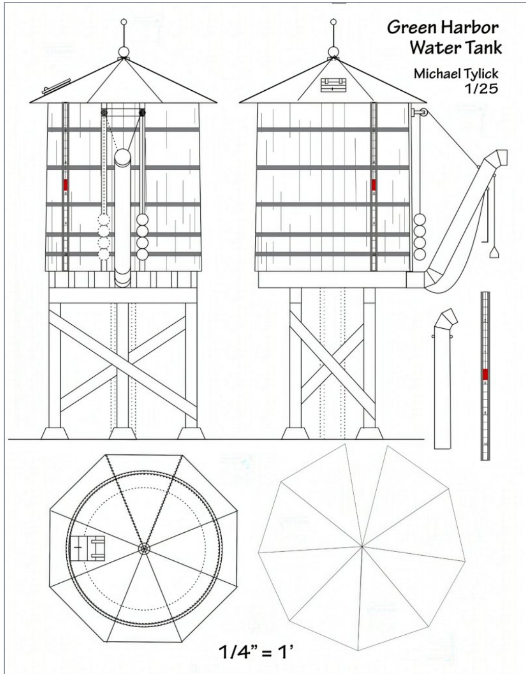
1a. Water tank plans.
