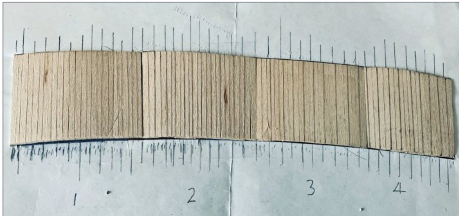
6. The four slightly trapezoidal panels are lined up on the template. Each has been scribed along the template markings.
