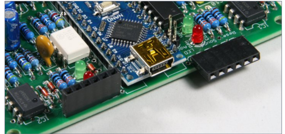
11. Female 6-pin headers for auxiliary connections (vertical or right-angle).
