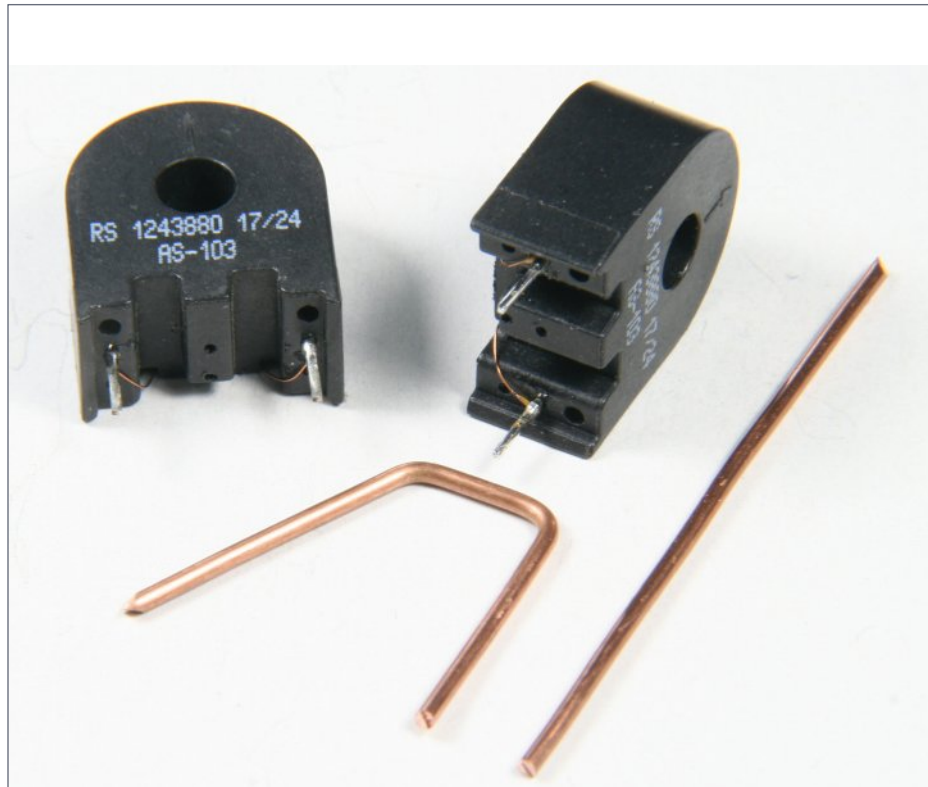
7. Preparation of the loop wire for current transformers.
