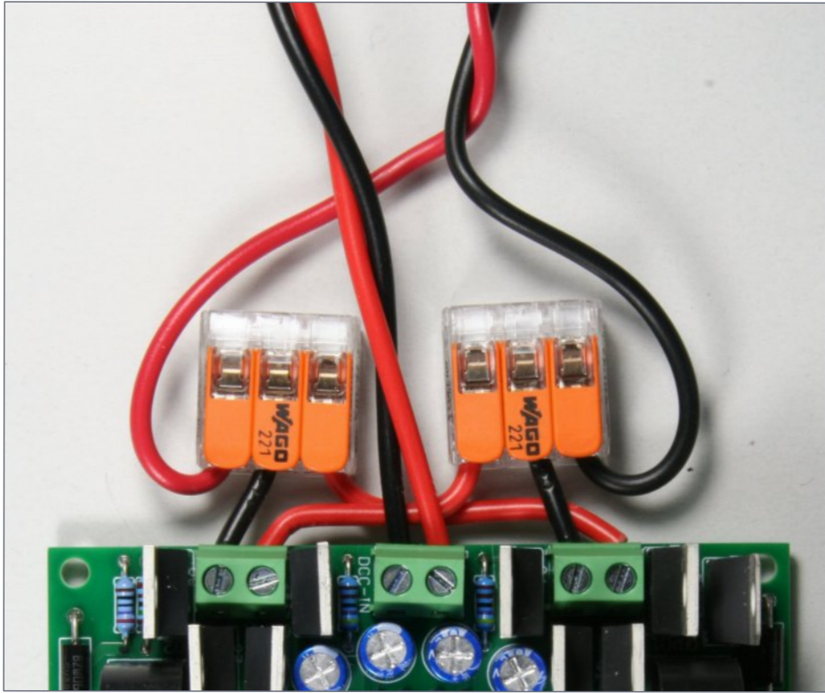
22. Dual Power Breaker connected as auto-reverser.
