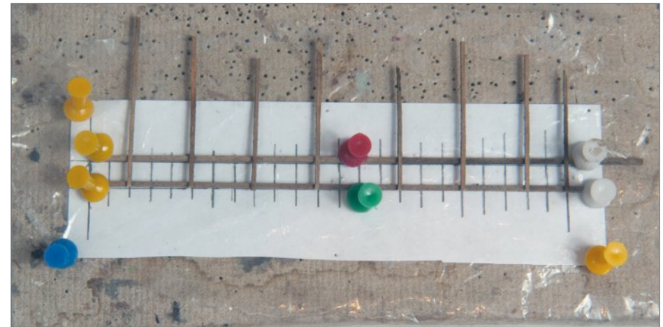
28. Every third rung is attached. I trimmed them to size after the glue dried.
