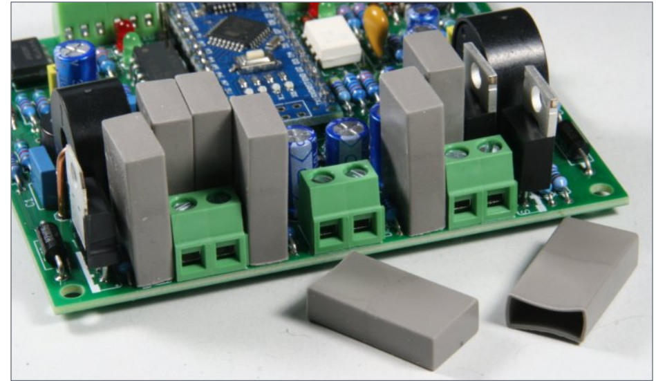
14. Insulation caps for the power MOSFETs.
