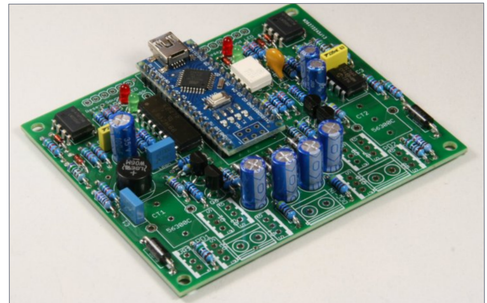
6. Fitment of electrolytic capacitors to PCB.
