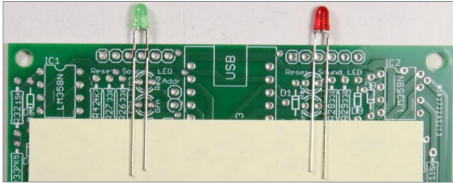
4. LEDs – correct orientation – short lead toward Nano module.
