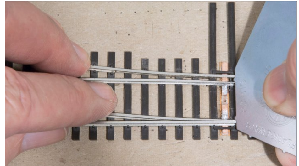
15. The points spacing on this Walthers/Shinohara turnout is now set to the correct (P) spacing. Compare to before [9].
