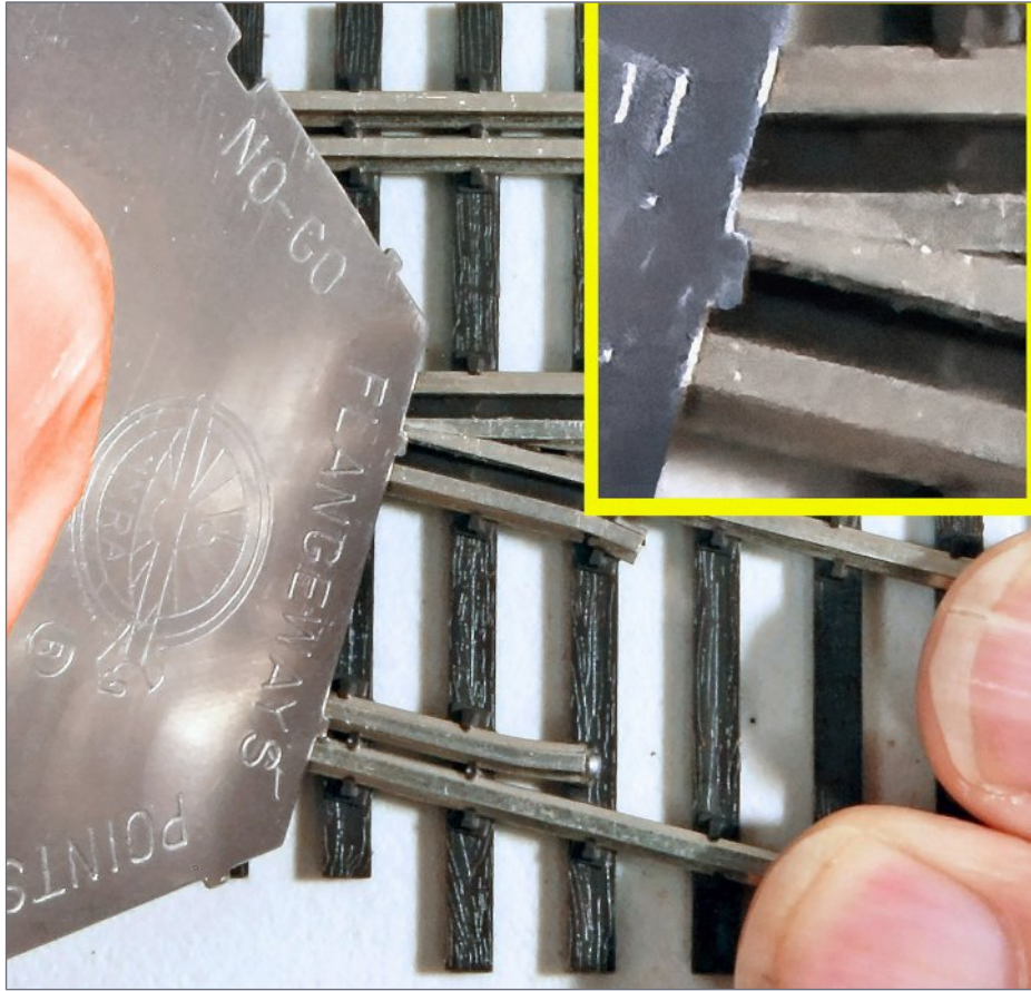
11. The NMRA check gauge is too narrow in this Walthers/Shinohara turnout, which allows properly in-gauge wheelsets to pick the frog and maybe derail. It is worth upgrading to NMRA spec [12].
