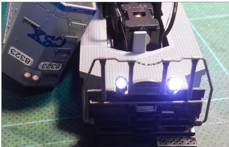
38. Testing the installed ditch lights.
