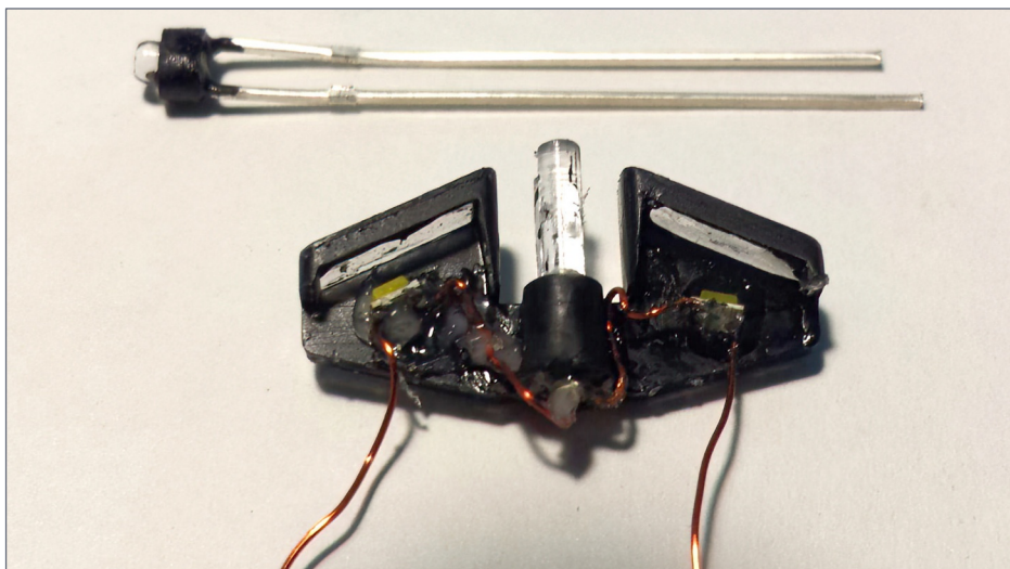
22. The cab rooftop rotating beacon (top), and the clear headlight/number board casting fitted with SMD LEDs (bottom). The black paint is to reduce light leaks.
