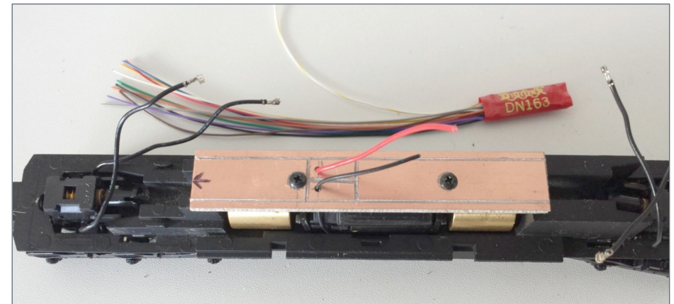
8. A scratchbuilt copper-clad 'motherboard' replaces the stock light board, providing clean mounting and wiring points for the DCC decoder. The red and black wires on the board center go to the motor – by NMRA standards, they should be orange and gray. I later fixed this [9].
