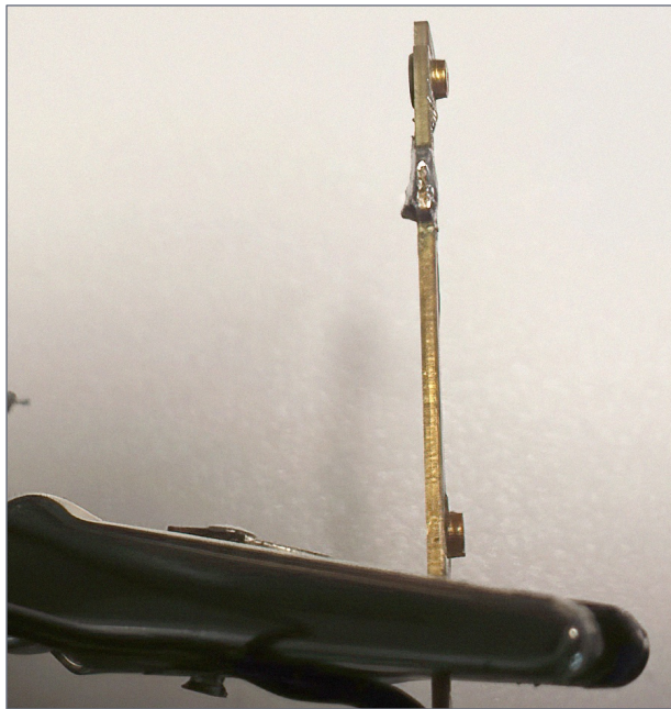
7. This pickup plate is held for soldering. The protrusions on the right side of the plate should nest into the truck side frame.
