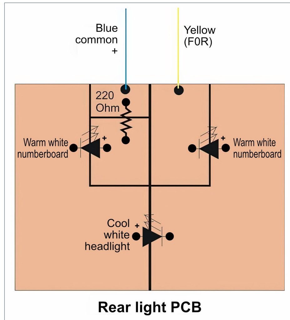
14. Using copper-clad board and cutting it into regions with a cutoff disk, I can wire it as shown here for the headlights, bridging each pad area to "wire" it. Also see [15, 16].
