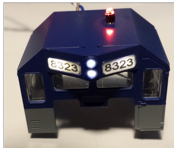
25. Finished cab assembly under power, showing the working beacon, main bright-white headlight, and warm-white boards.
