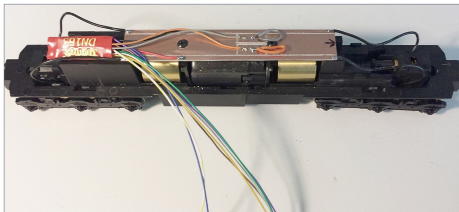
9. Digitrax DN163 decoder wired to the DIY motherboard on the chassis, with the orange and gray motor lead wire colors corrected.
