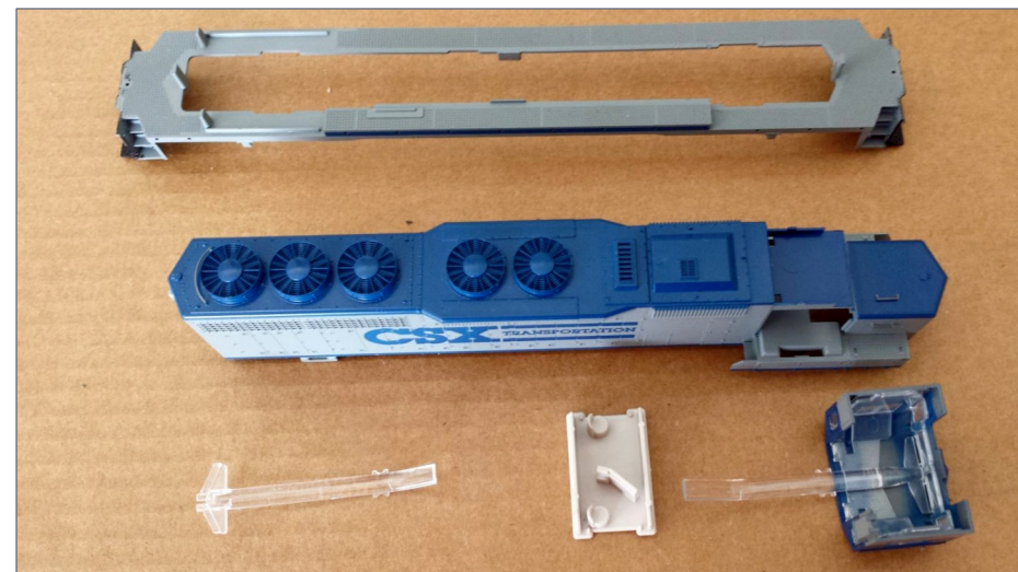
11. To begin Phase 2, I dismantled the Kato SD40 body into its major components: walkway, long hood, rear clear lighting guide, cab interior, and cab with its clear light guide.
