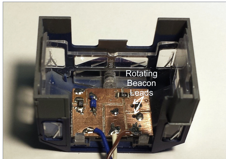
21. The DIY headlight/number board light PCB placed in the cab roof, with the blue, white, and brown decoder wires feeding the board. Headlight and number board clear plastic block not yet installed.
