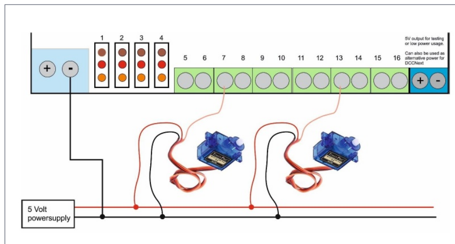
13. Servos connected to DCCNext, showing the additional connection to DCCNext ground.
