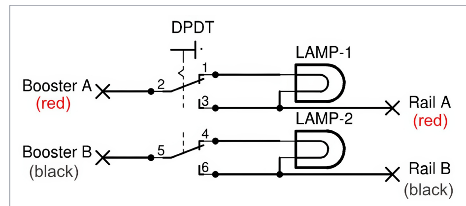
7. Wiring diagram for the #1156 current-limiting circuit.
