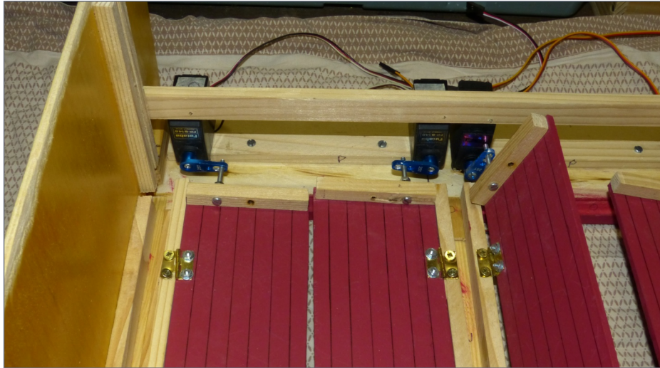
10. Everything is in place: servos connected to doors, servos fastened to support strips.
