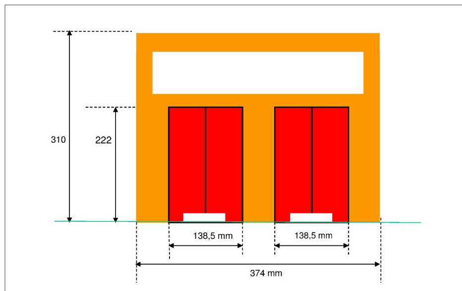
2. Draft of the new shed front with doors.
