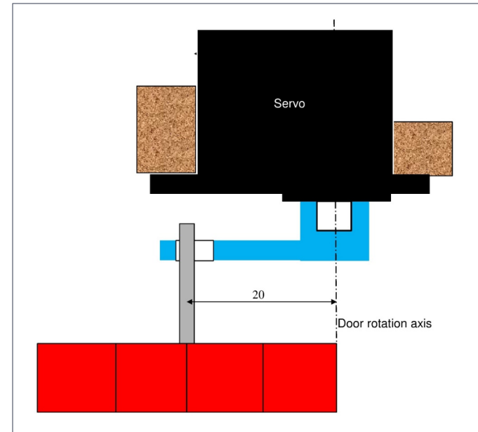
8. Servo installation drawing.
