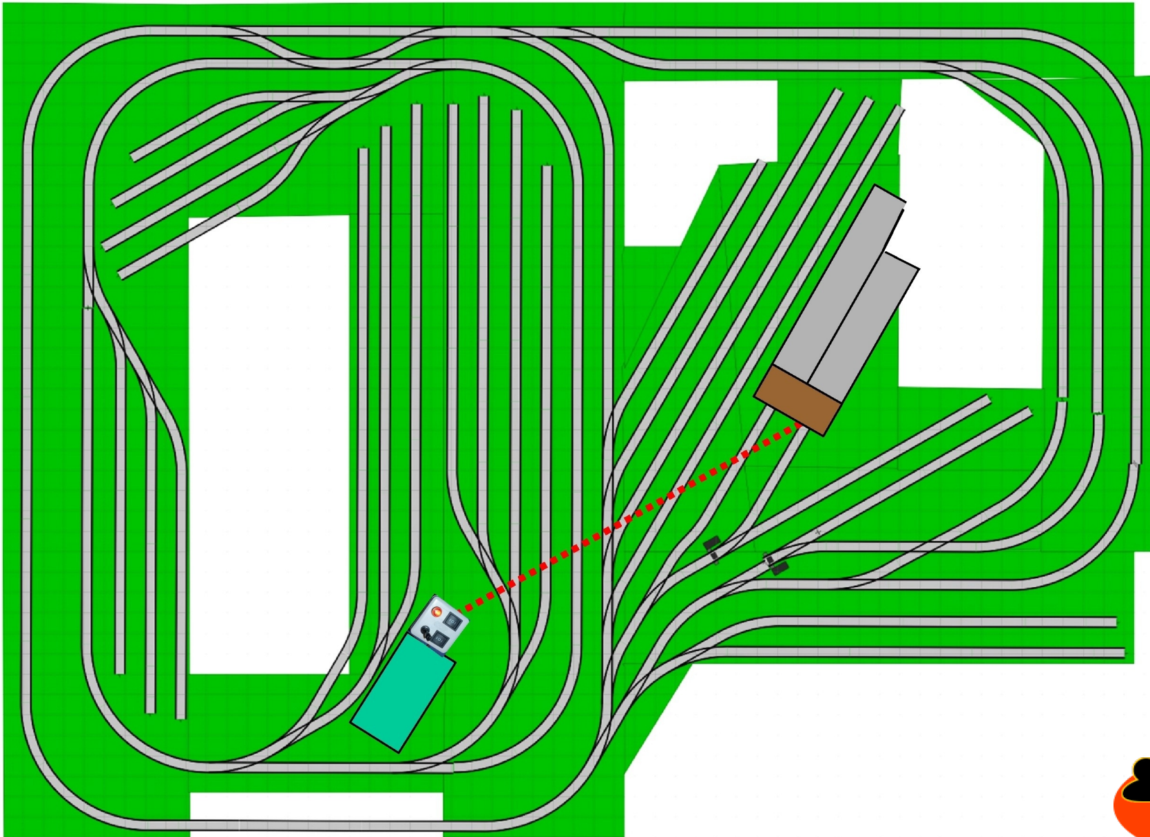
20. Layout drawing showing wiring between main control area and shed.
