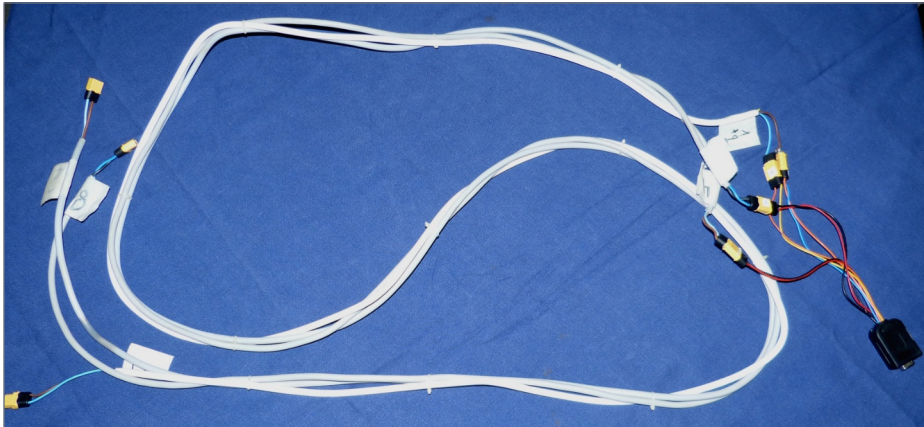
22. Wire bundle for installation underneath the layout. I have labeled the wire pairs, and everything has been fitted with two-wire connections for easy installation under the layout.
