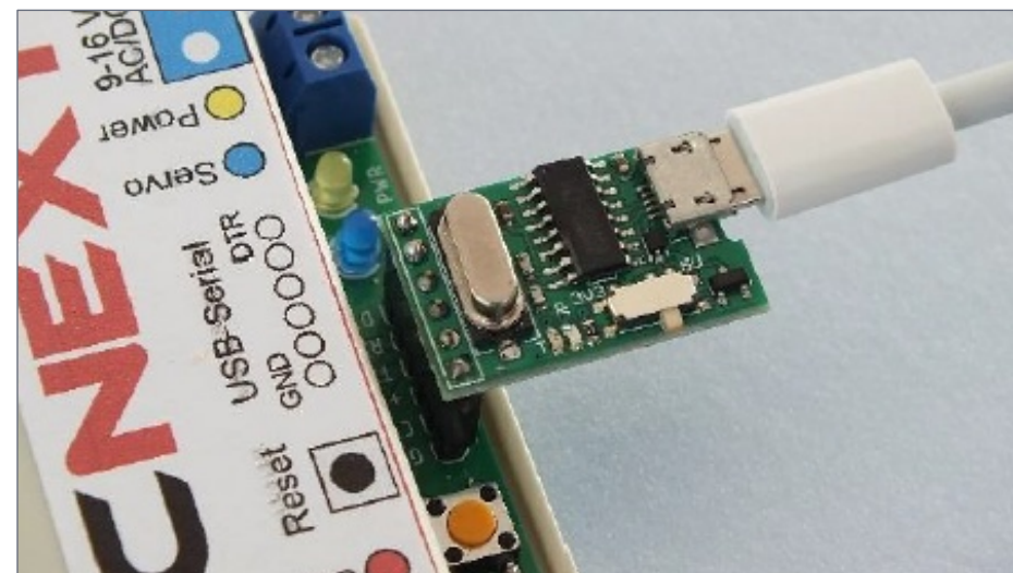
12. USB option linking DCCNext and home PC.
