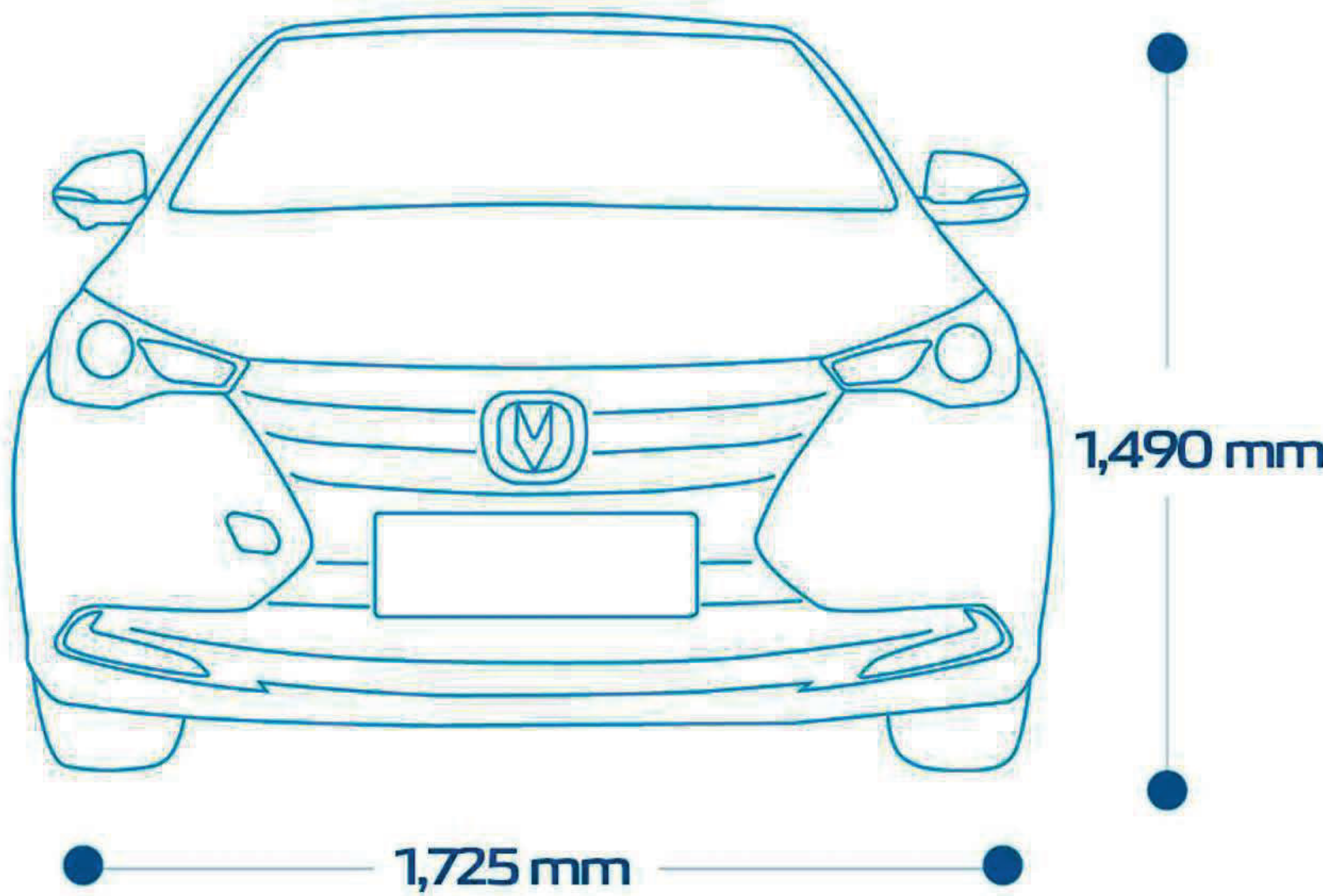
Ancho 1,725 mm
