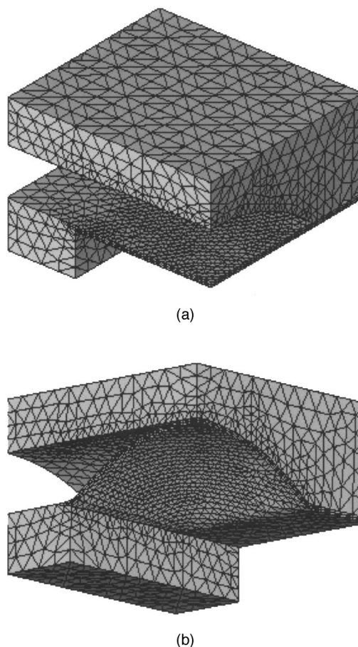
FIG. 6. Computational model of a microvalve consisting of a 300 \times 56 \mu\text{m} control channel, a 300 \times 50 \mu\text{m} fluidic channel, and a 5- \mu\text{m} -thick membrane. The mesh consists of 3365 nodes and 1622 ten node tetrahedral finite elements. (a) Undeformed configuration (b) Deformed configuration at actuation pressure.
