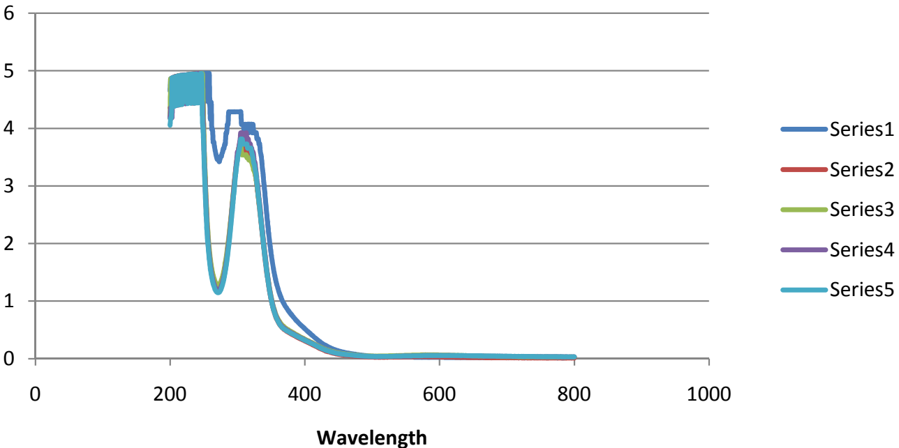
Corrected Absorbance of BSA/HAuCl4 vs. Time
