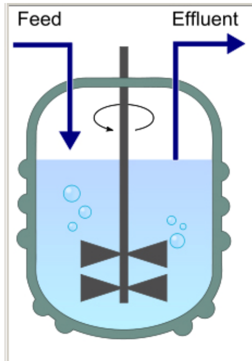
Figure 1. Chemostat cartoon from Wikipedia.
