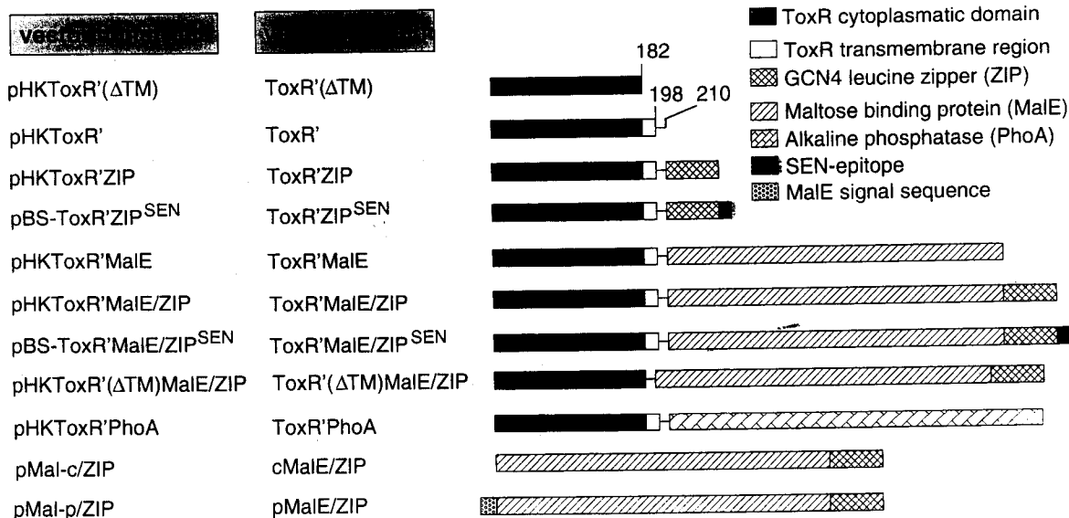
Fig. 2. Modular organization of chimeric proteins employed in this study. In the vector series pHKToxR' (Kolmar et al. , 1994), chimeric toxR' genes are under transcriptional control of V.cholerae toxR promoter. For overexpression, the respective constructs were cloned into vector pBS [pBluescript II SK(-) TM ]. Here, the fusion genes are under additional control of the lac promoter. Soluble MalE/ZIP fusion proteins were accumulated alternatively in the cytoplasmic or the periplasmic compartment of E.coli by expression of the respective genes residing in vectors pMal-c/ZIP and pMal-p/ZIP; in the latter case, an N-terminal leader sequence is provided. For details of construction of the respective fusion genes, see Materials and methods.
