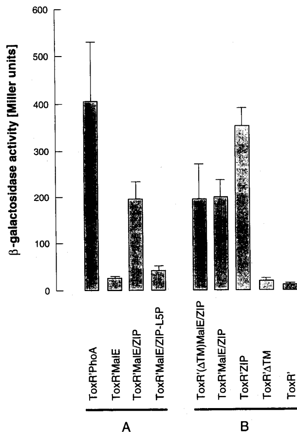
Fig. 4. (A) Transcription activation of ctx promoter mediated by ToxR' fusion proteins that have their periplasmic domain substituted by various other proteins. (B) Transcription activation of ctx promoter mediated by various cytoplasmic or membrane-bound ToxR' fusion proteins (see Figure 2). Each bar displays specific \beta -galactosidase activity in crude cell lysates obtained from overnight cultures of six individual colonies. Standard deviations are indicated by error bars.
