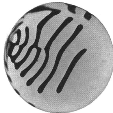
Figure 3 Morphology of precipitation induced by poly(L-Glu)
