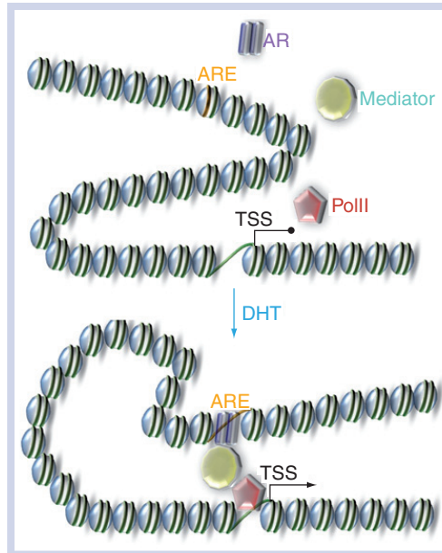
Figure 3. Androgen-induced nucleosome repositioning and chromosomal looping.
