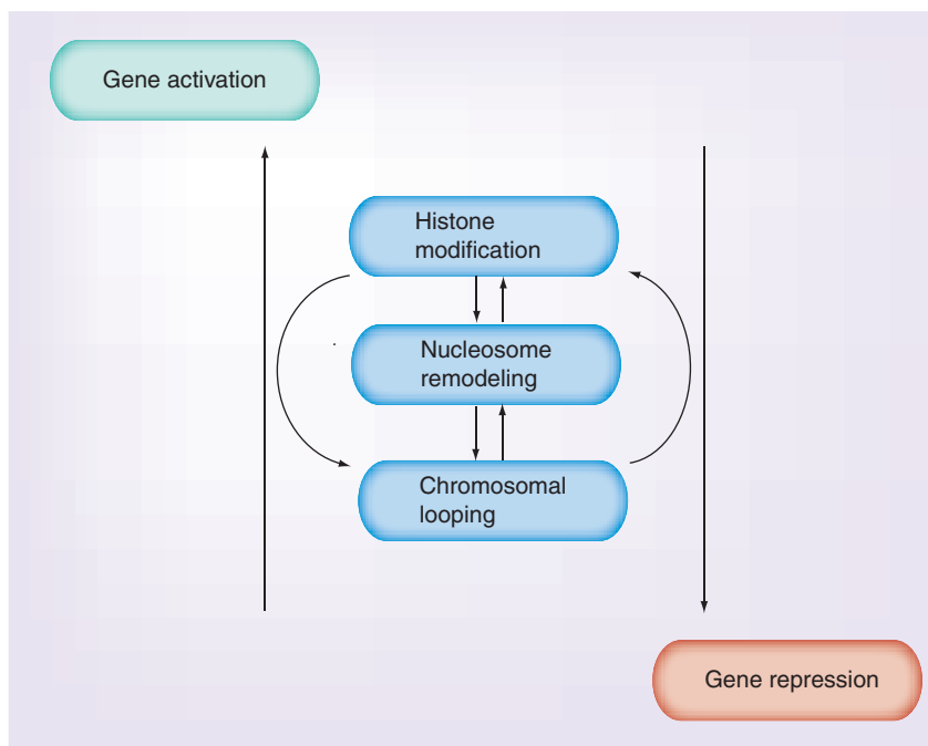
Figure 2. The interplay among histone modification, nucleosome remodeling and chromosomal looping leads to gene activation or repression in prostate cancer. For example, a histone modification may be recognized by a chromatin remodeler that causes nucleosome ejection. This may lead to a transcription factor binding, chromosomal looping and gene activation (see FIGURE 3).
