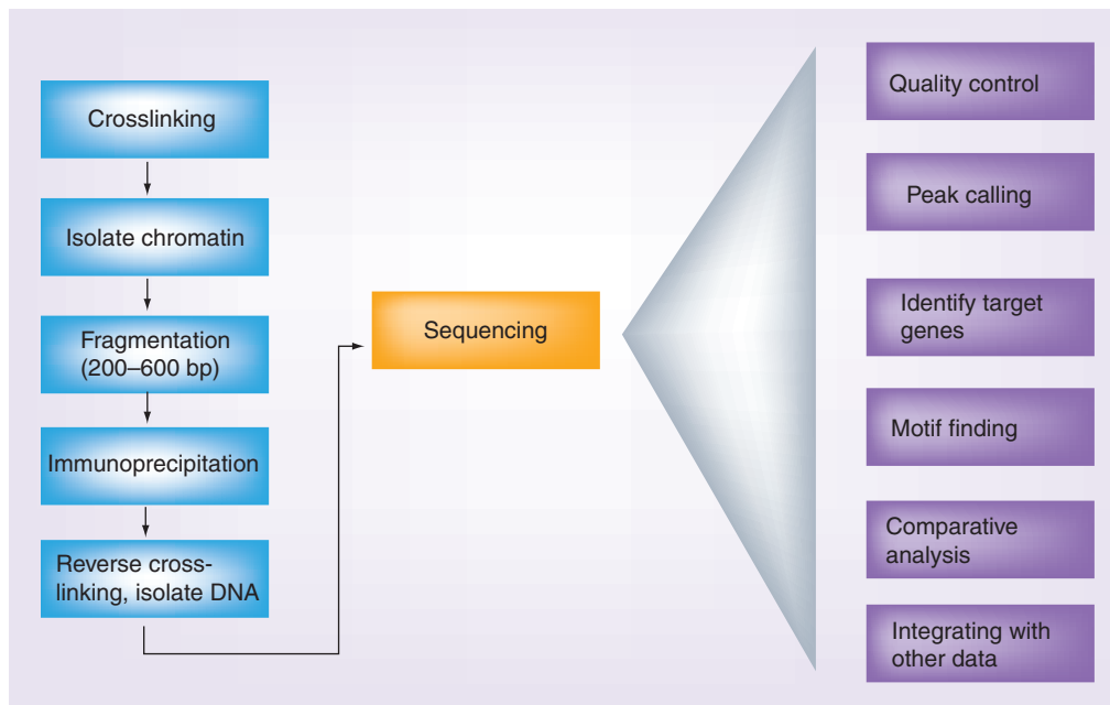
Figure 1. A typical workflow for chromatin immunoprecipitation combined with high-throughput sequencing. Experimental procedures are presented in the boxes on the left; sequencing step is indicated in the middle box and is not fully explained; the bioinformatics analysis parts are presented in the boxes on the right
