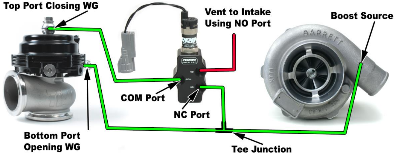
PERRIN EBCS solenoid shown connecting to External Wastegate. NOTE: Intake Manifold can be uses as boost source.
