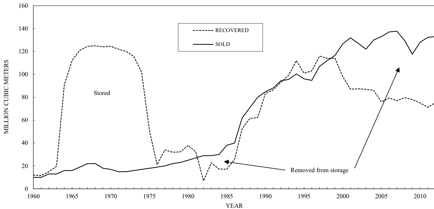
FIGURE 2 HELIUM RECOVERY IN THE UNITED STATES, 1960–2012
