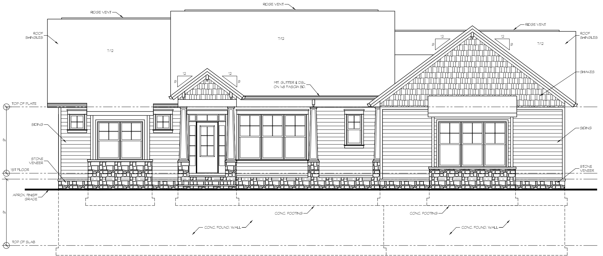
FRONT ELEVATION 1/8"=1'-0"
