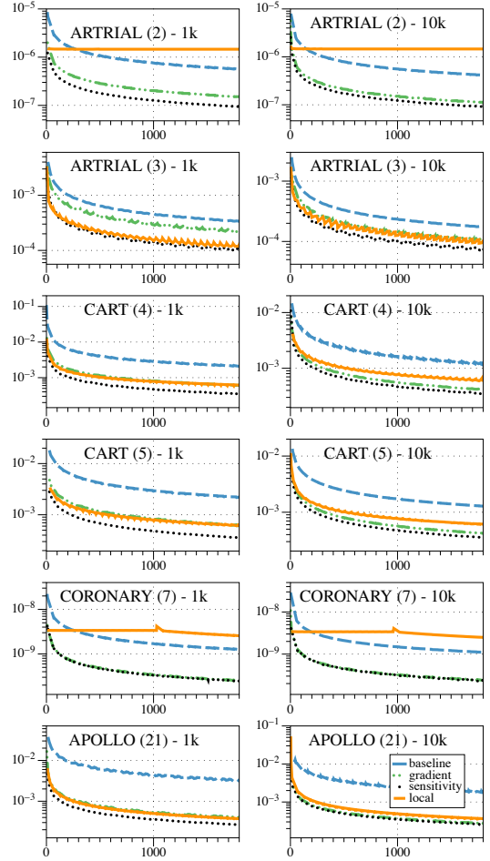
Figure 5: Convergence rate of iterative sampling and the baseline approach on selected subjects (y-axis in logarithmic scale).
