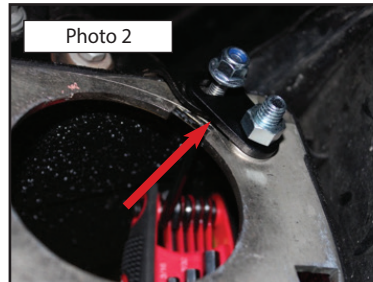
Use mounting tab tied into factory bucket mount to reinforce bracket attachment to bucket.
