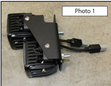
Dually/D2 lights mounted to bracket. Insert bracket mount bolts first.
