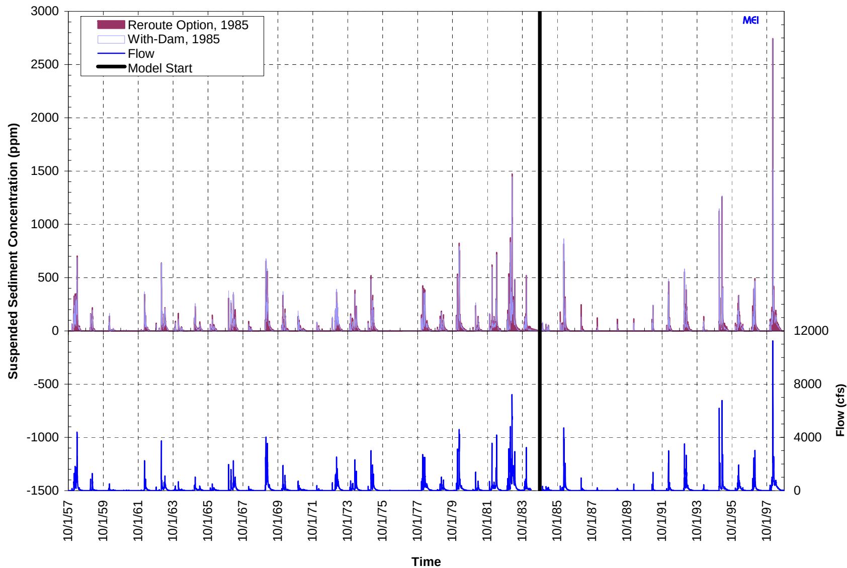
Figure C.1.20. Computed daily suspended sediment concentrations for with-dam conditions and the Reroute and Removal Option in Subreach 9 (1985 start date).
