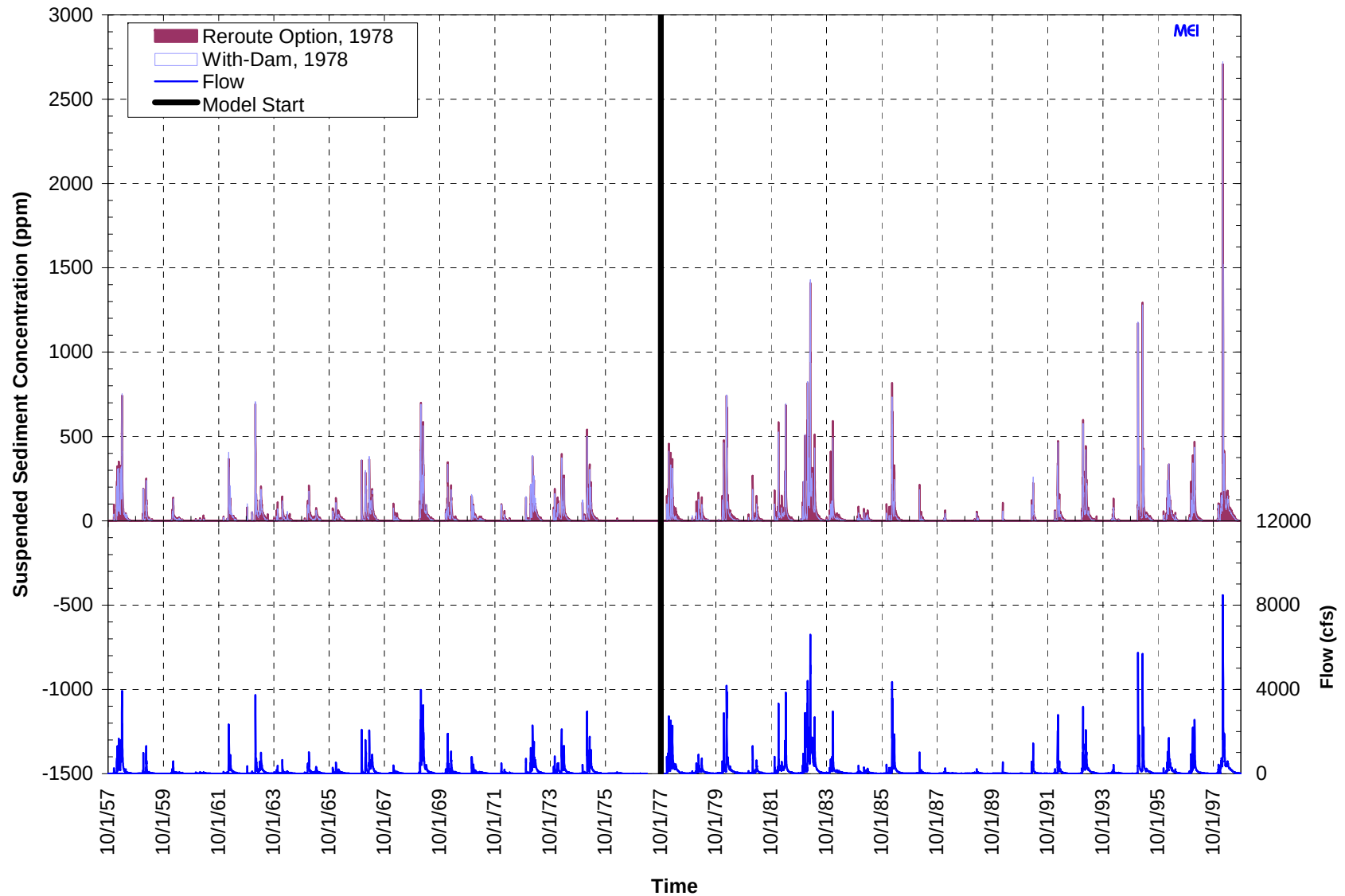
Figure C.1.9. Computed daily suspended sediment concentrations for with-dam conditions and the Reroute and Removal Option in Subreach 8.7 (1978 start date).
