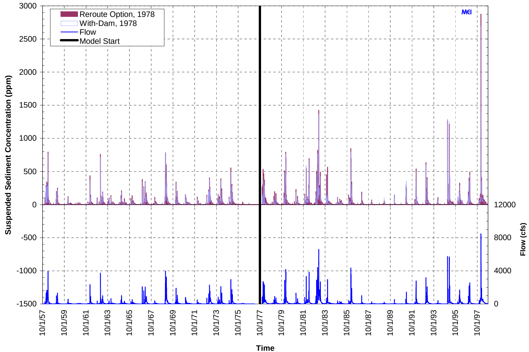
Figure C.1.6. Computed daily suspended sediment concentrations for with-dam conditions and the Reroute and Removal Option in Subreach 7.3 (1978 start date).
