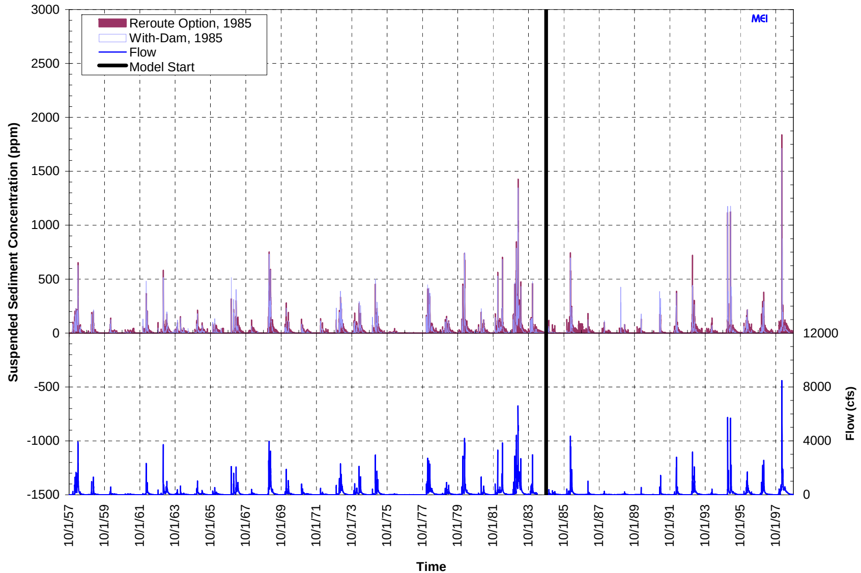
Figure C.1.11. Computed daily suspended sediment concentrations for with-dam conditions and the Reroute and Removal Option in Subreach 4.3 (1985 start date).
