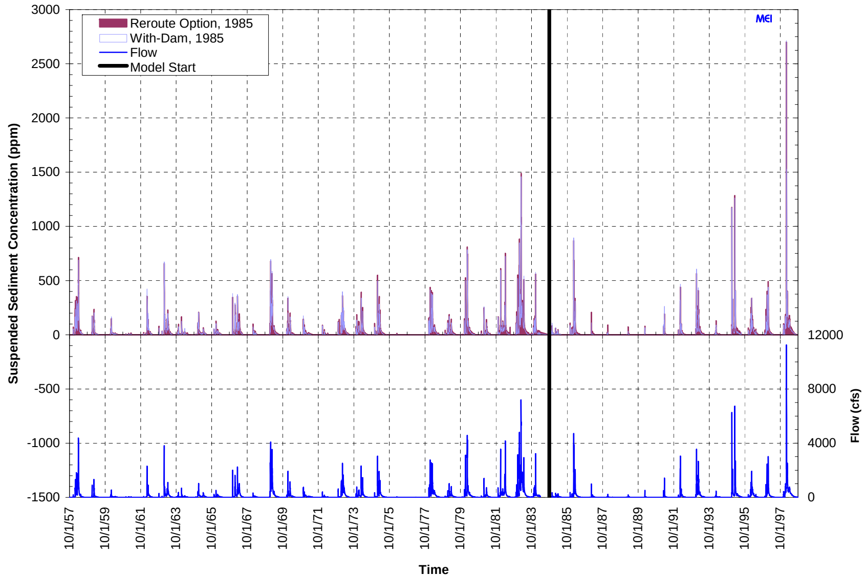
Figure C.1.19. Computed daily suspended sediment concentrations for with-dam conditions and the Reroute and Removal Option in Subreach 8.7 (1985 start date).
