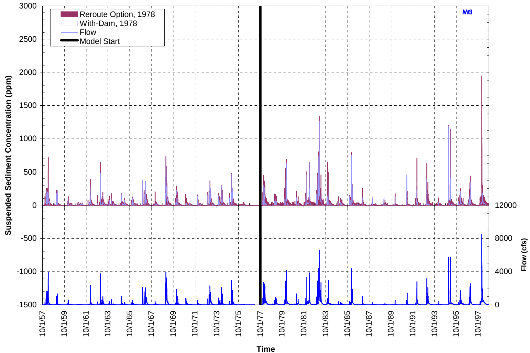
Figure C.1.1. Computed daily suspended sediment concentrations for with-dam conditions and the Reroute and Removal Option in Subreach 4.3 (1978 start date).
