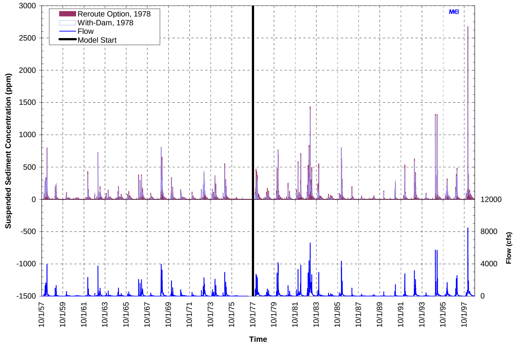
Figure C.1.7. Computed daily suspended sediment concentrations for with-dam conditions and the Reroute and Removal Option in Subreach 7.7 (1978 start date).
