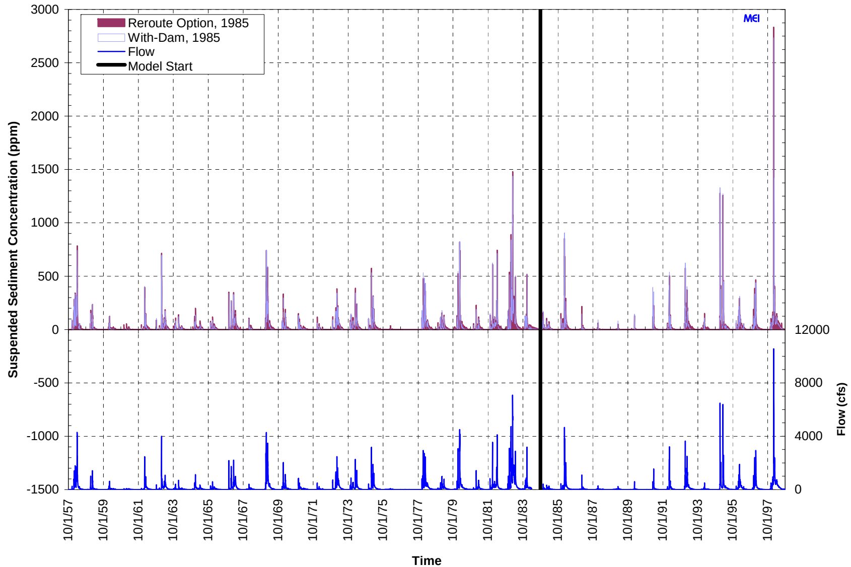
Figure C.1.16. Computed daily suspended sediment concentrations for with-dam conditions and the Reroute and Removal Option in Subreach 7.3 (1985 start date).
