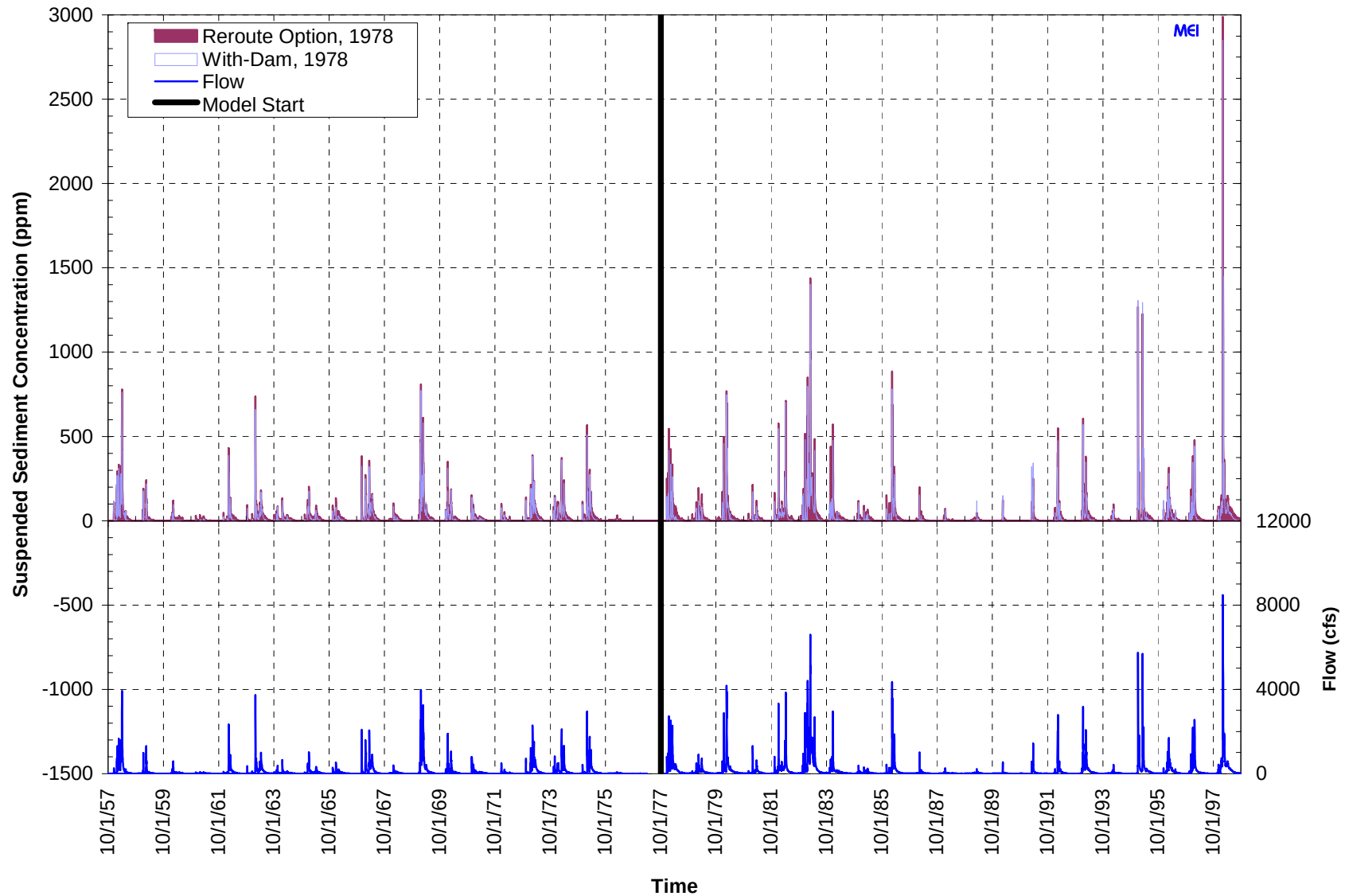
Figure C.1.5. Computed daily suspended sediment concentrations for with-dam conditions and the Reroute and Removal Option in Subreach 6.7 (1978 start date).
