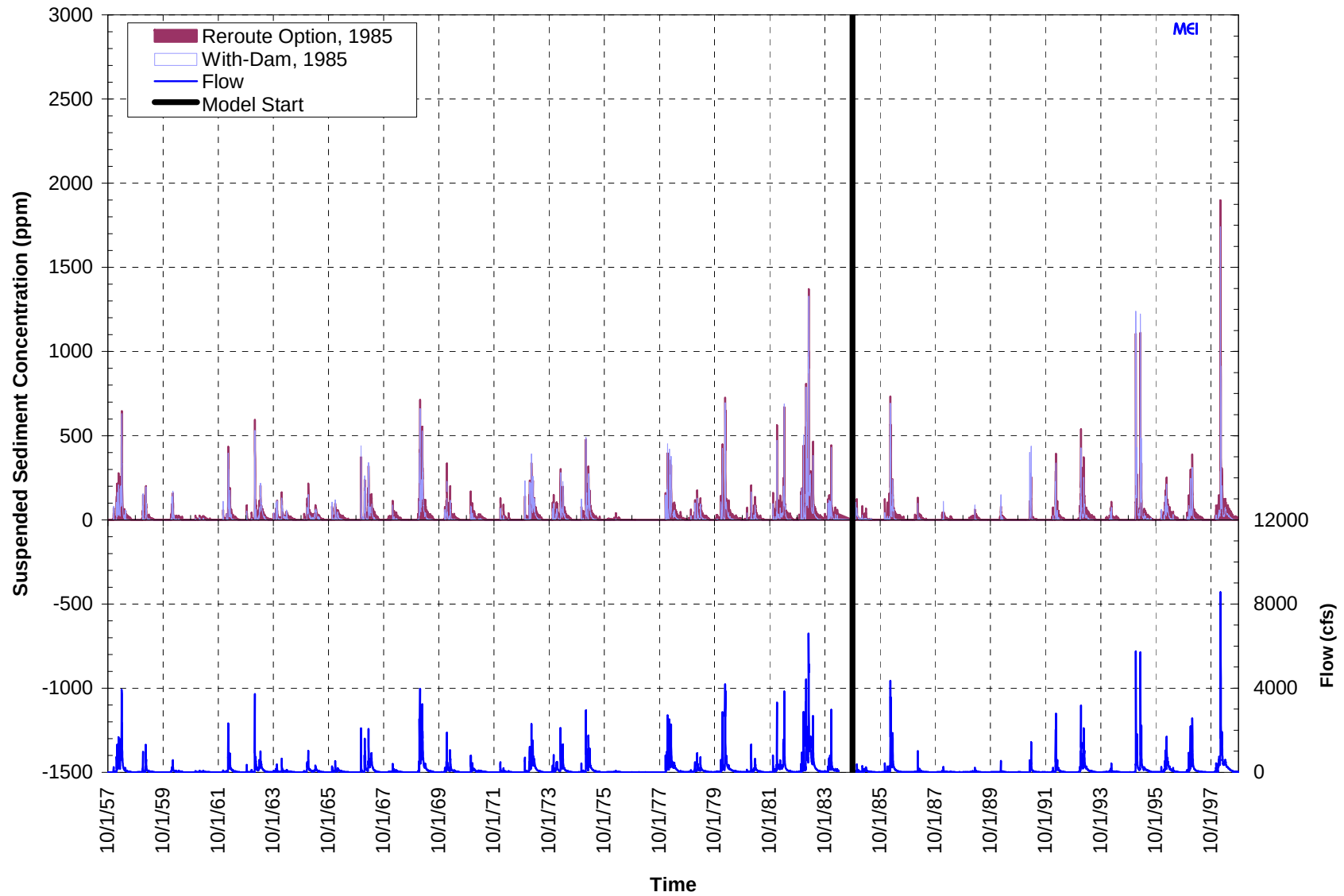
Figure C.1.12. Computed daily suspended sediment concentrations for with-dam conditions and the Reroute and Removal Option in Subreach 4.7 (1985 start date).
