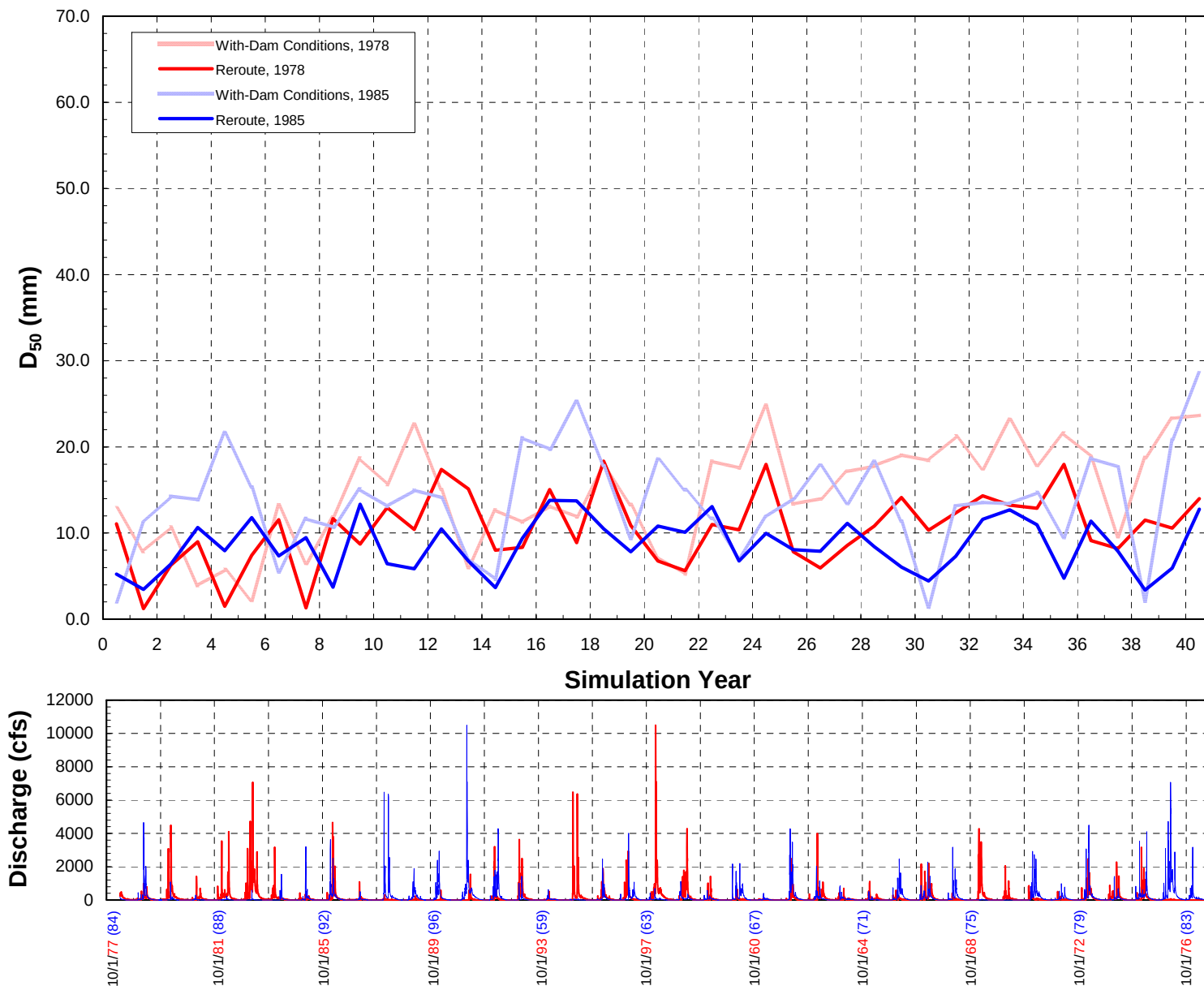
Figure D.5. Temporal change in median grain size in Subreach 6.7 for with-dam conditions and the Reroute and Removal Option, 1978 and 1985 start dates.
