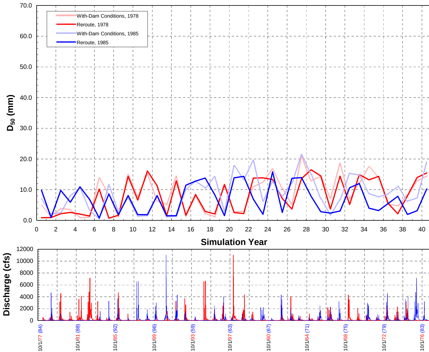
Figure D.8. Temporal change in median grain size in Subreach 8.3 for with-dam conditions and the Reroute and Removal Option, 1978 and 1985 start dates.
