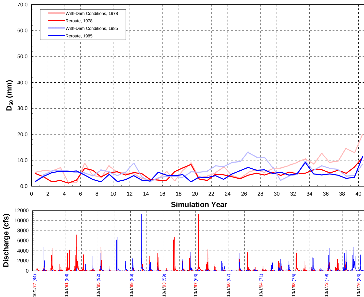
Figure D.10. Temporal change in median grain size in Subreach 9 for with-dam conditions and the Reroute and Removal Option, 1978 and 1985 start dates.
