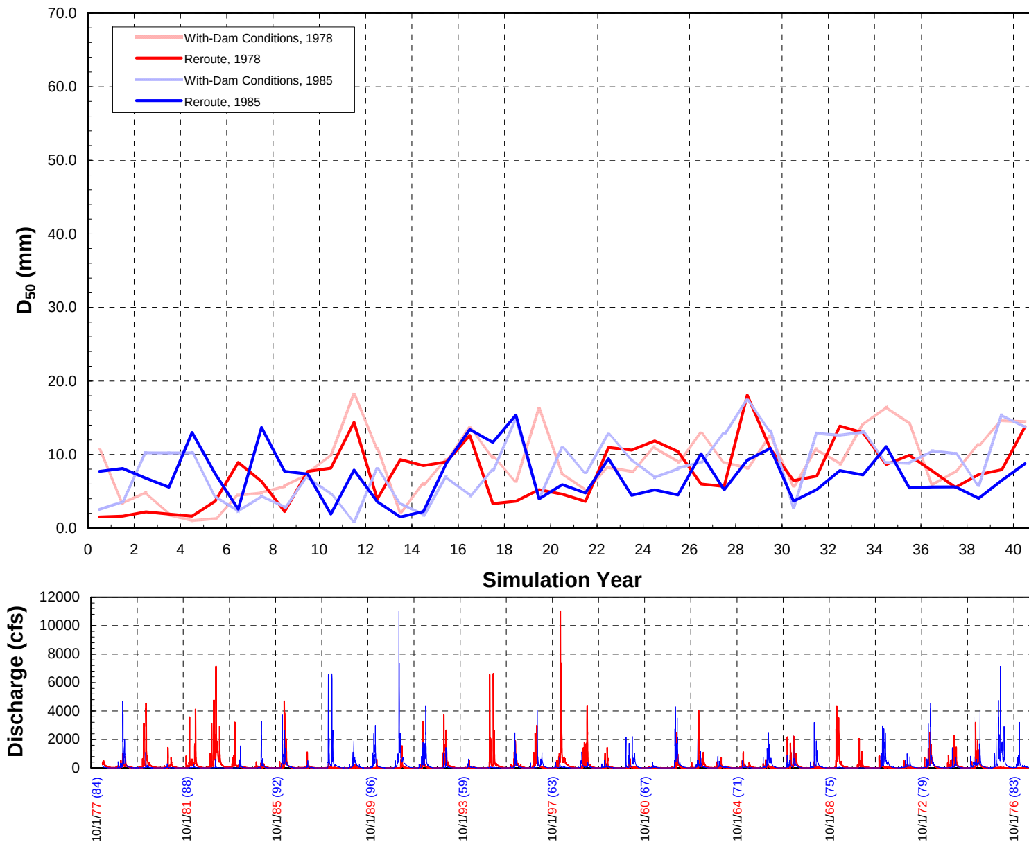
Figure D.7. Temporal change in median grain size in Subreach 7.7 for with-dam conditions and the Reroute and Removal Option, 1978 and 1985 start dates.
