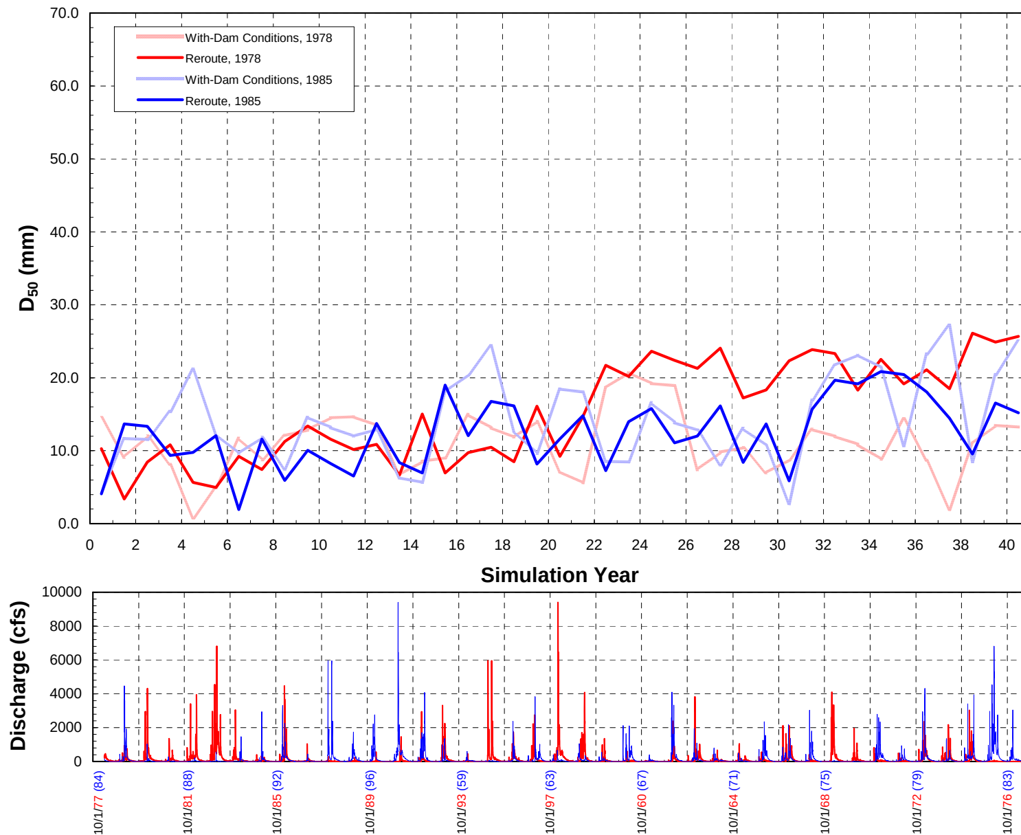
Figure D.4. Temporal change in median grain size in Subreach 6.3 for with-dam conditions and the Reroute and Removal Option, 1978 and 1985 start dates.
