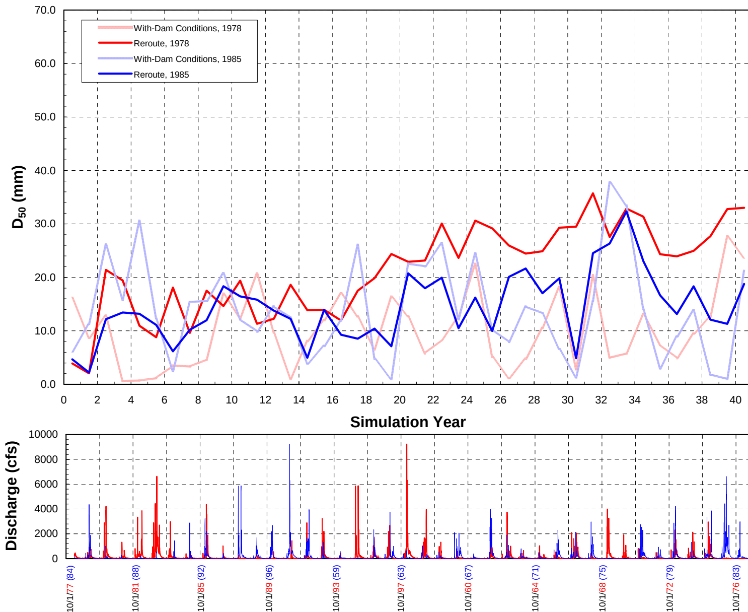
Figure D.3. Temporal change in median grain size in Subreach 5 for with-dam conditions and the Reroute and Removal Option, 1978 and 1985 start dates.
