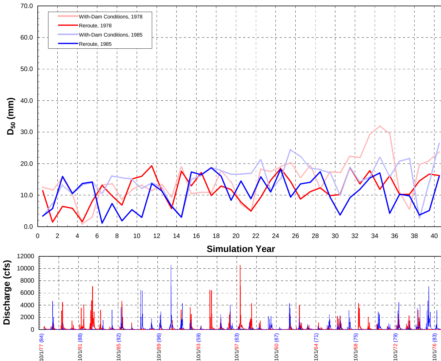
Figure D.6. Temporal change in median grain size in Subreach 7.3 for with-dam conditions and the Reroute and Removal Option, 1978 and 1985 start dates.
