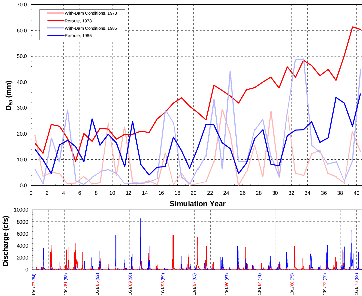
Figure D.2. Temporal change in median grain size in Subreach 4.7 for with-dam conditions and the Reroute and Removal Option, 1978 and 1985 start dates.
