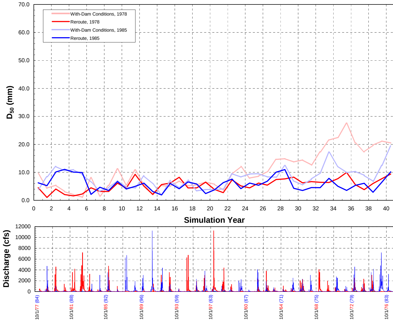
Figure D.9. Temporal change in median grain size in Subreach 8.7 for with-dam conditions and the Reroute and Removal Option, 1978 and 1985 start dates.
