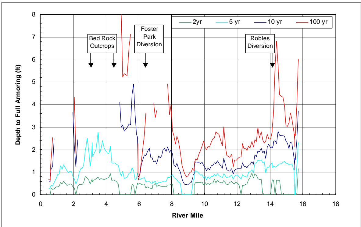
Figure 5.27. Estimated Depth to Full Armoring.
