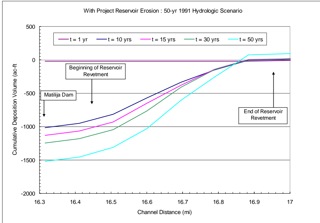
Figure 11.8. Erosion of Sediment from Matilija Reservoir under With-Project Conditions and 50-yr 1991 Hydrologic Scenario
