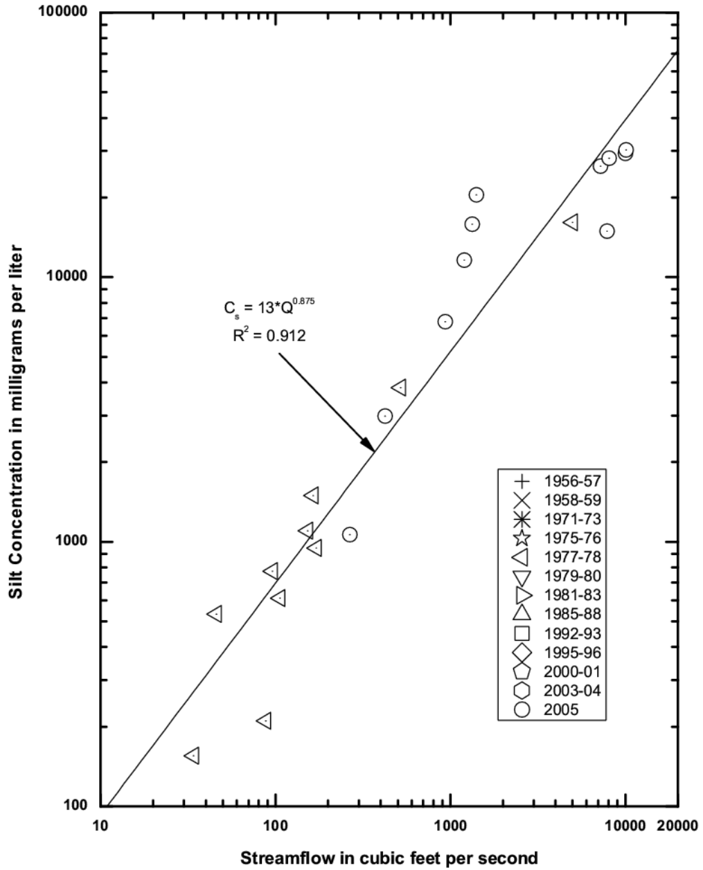
Figure 5.19. Silt Concentration on San Antonio Creek.
