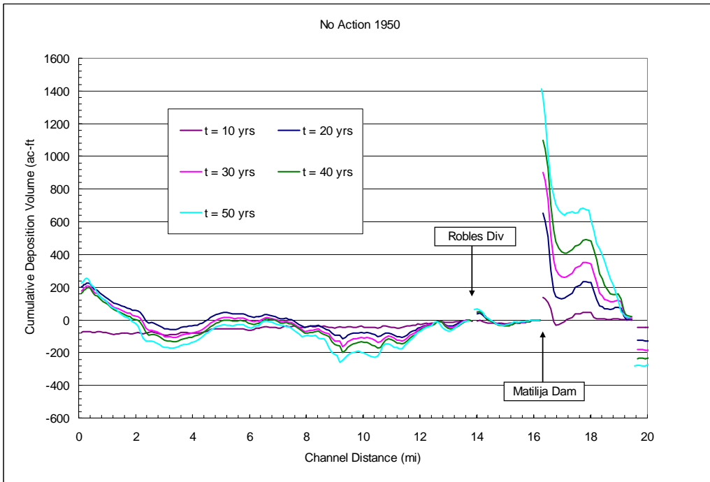
Figure 11.10. Cumulative Deposition for 1950 historical 50-yr hydrograph for Without Project Conditions.
