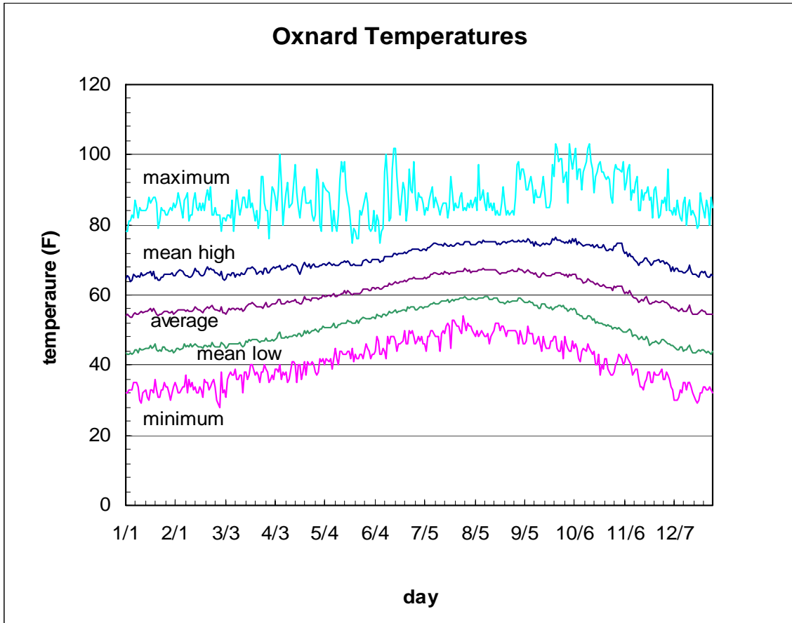
Figure 1.7. Temperatures at Oxnard (34° 11' 00" N 119° 10' 00"W, El. 49 ft) for the period of 1948 to 2000.
