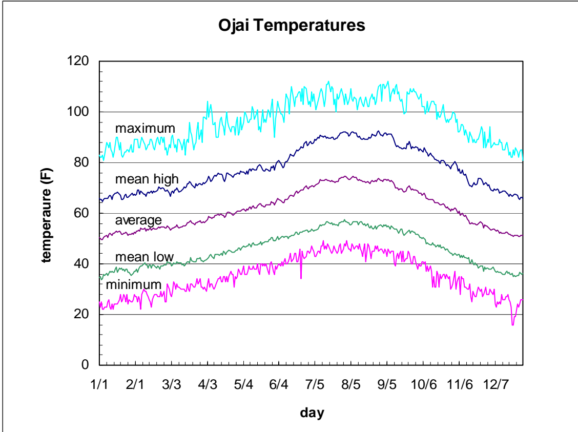
Figure 1.8. Temperatures at Ojai (34° 26' 00"N, 119° 13' 00"W, El. 750 ft) for the period 1948 to 2000.
