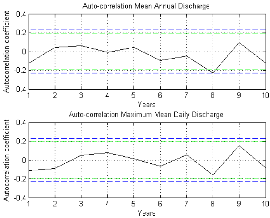
Figure 6.3. Gage 11116000 autocorrelation structure.
