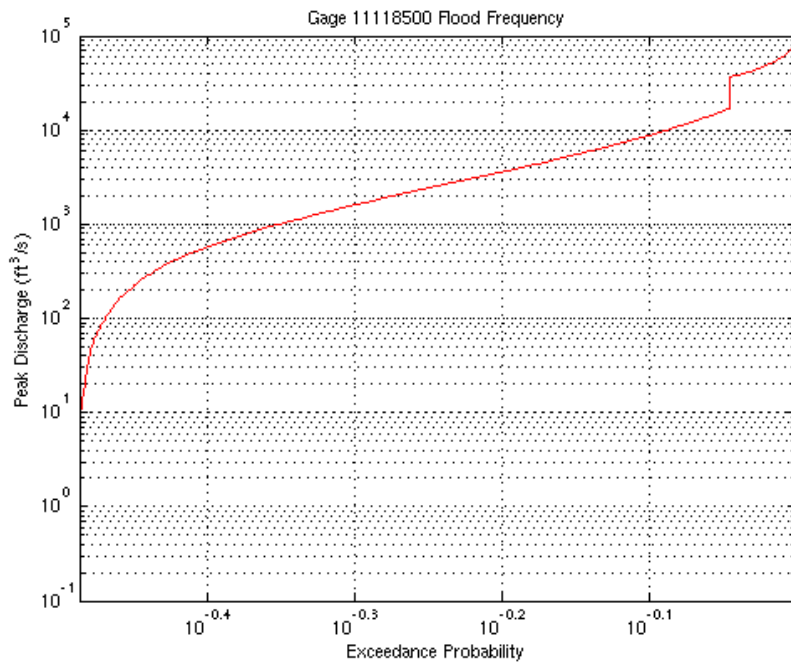
Figure 6.7. Flood Frequency curve for gage 11118500 used in stochastic simulations.
