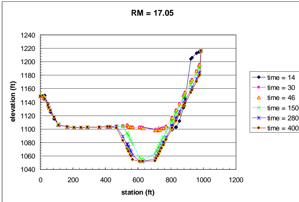
Figure 6.15. Example of Cross Section at Reservoir Delta for Alternative 2a for Two 100-yr Floods in Succession.
