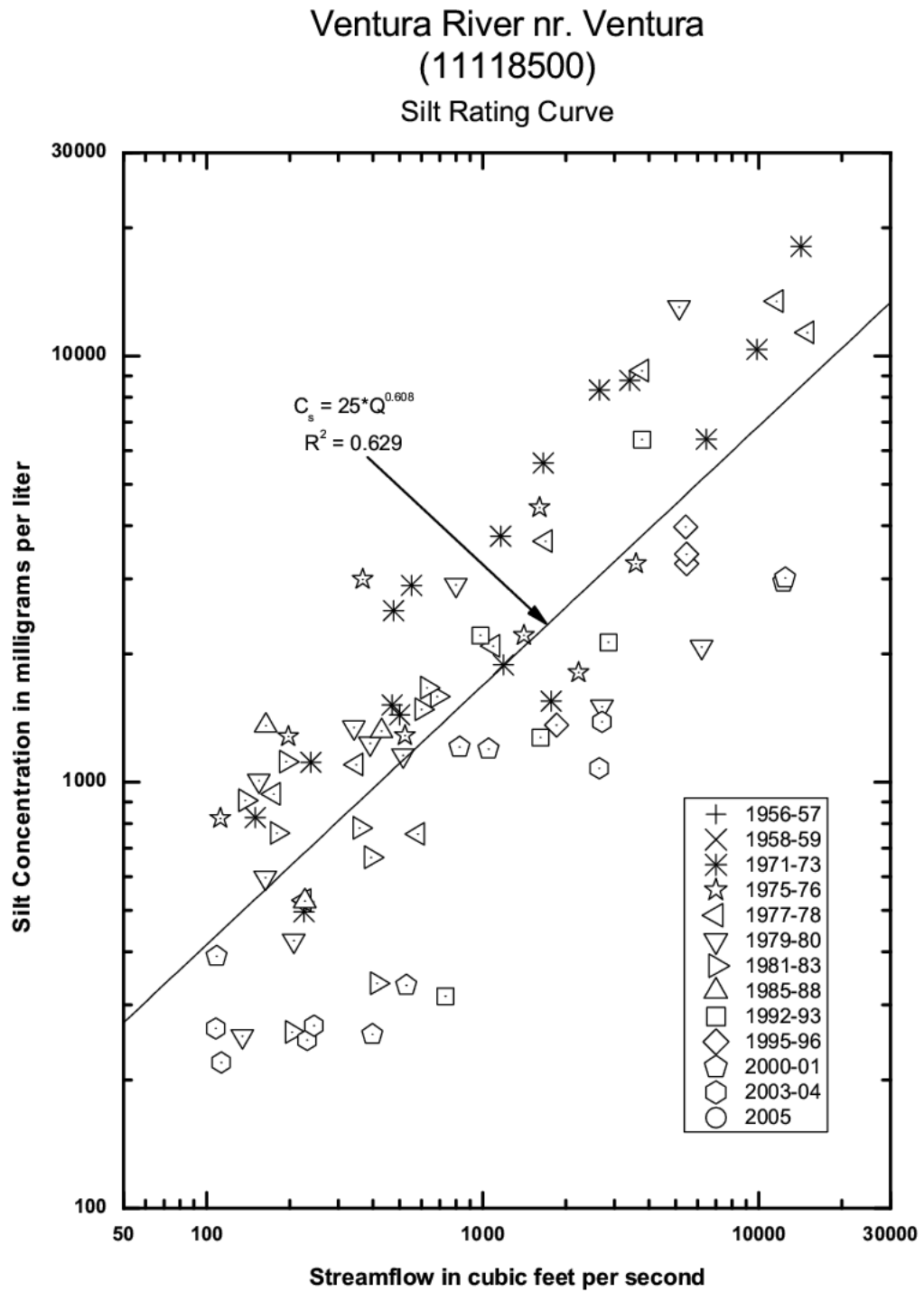
Figure 5.22. Silt Concentration on Ventura River at Foster Park.
