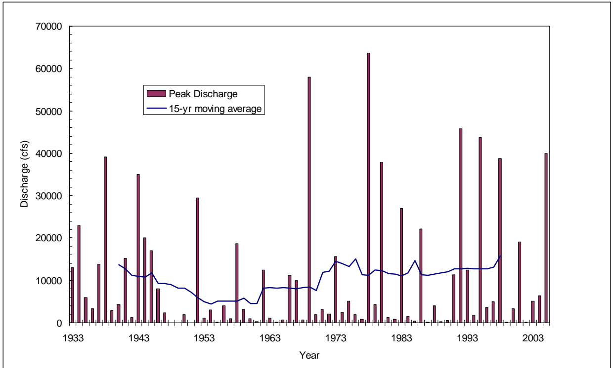
Figure 2.4. Peak Discharge at USGS gage 11118500, near Foster Park on the Ventura River.
