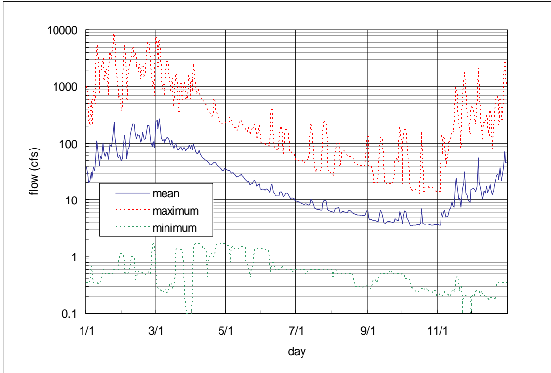
Figure 2.5. Mean, Maximum, and Minimum Daily Average Discharges for Every Day of the Year at USGS gage 11115500, downstream of Matilija Dam.
