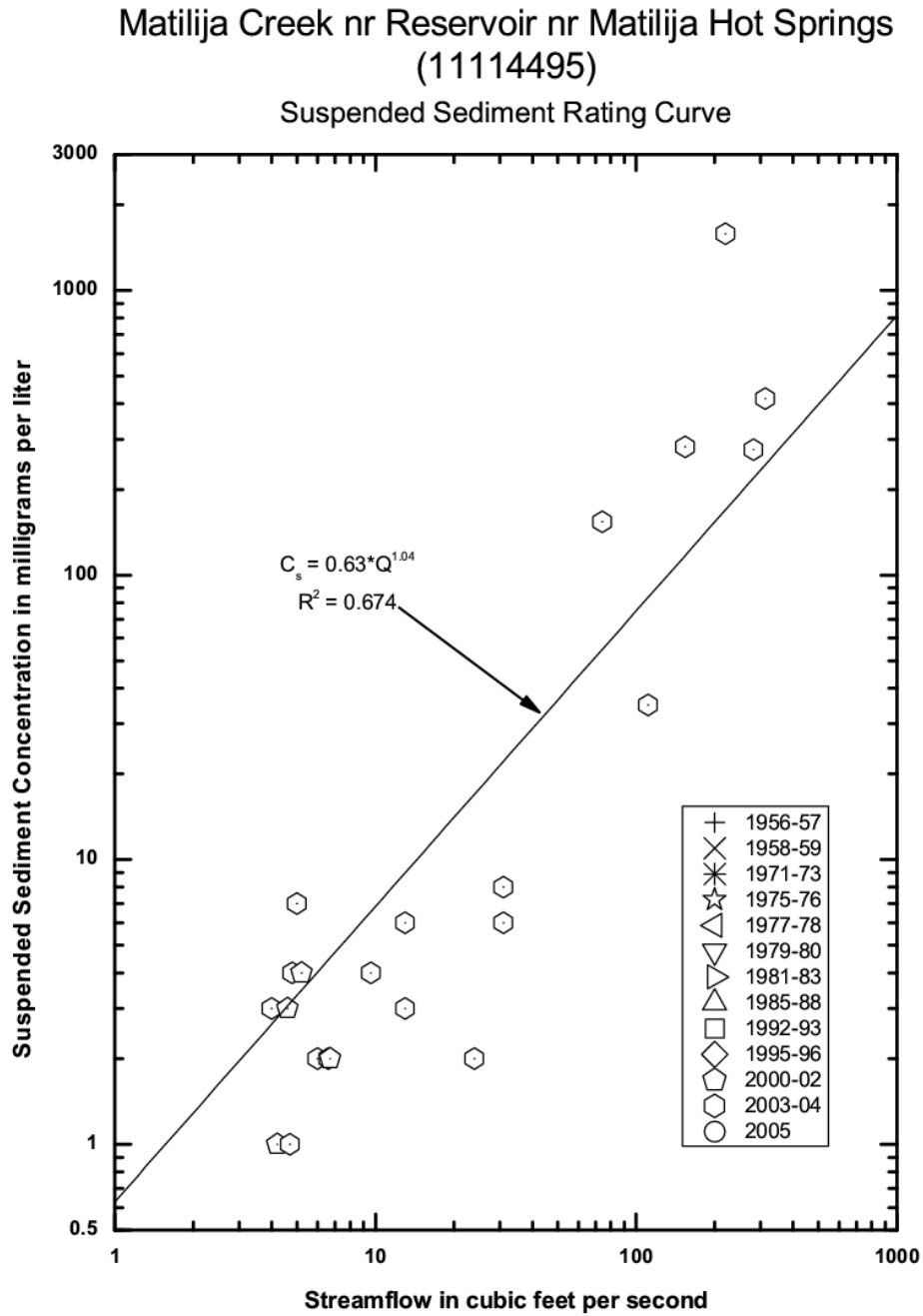
Figure 5.15. Total Suspended Sediment Versus Streamflow On Matilija Creek Upstream of Matilija Dam (USGS Gage #11114495).
