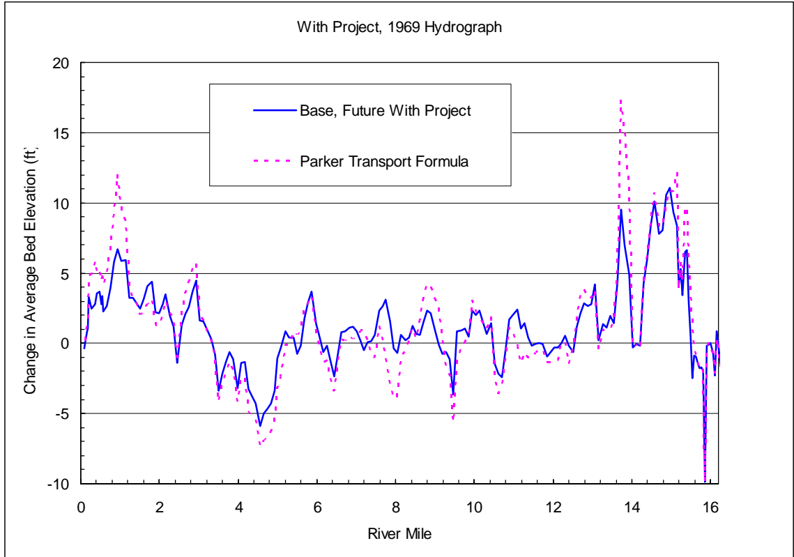
Figure 12.11. Affect of Transport Capacity Formula on Average Bed Elevations for 1969 Hydrograph.
