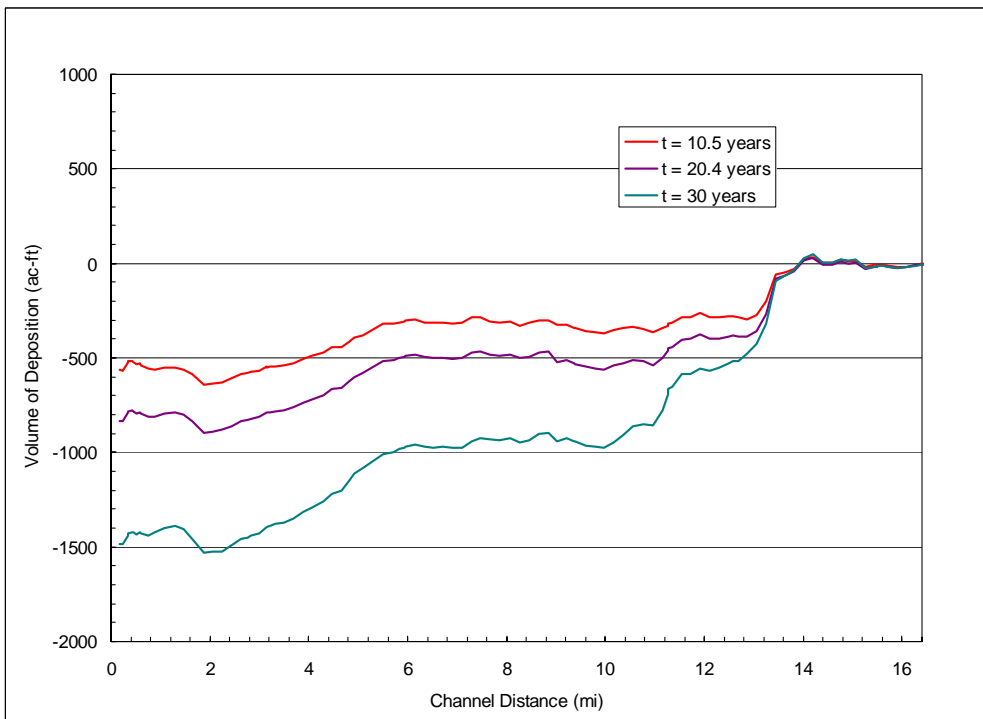
Figure 6.21. Computed Volume of Deposition between 1971 to 2001.
