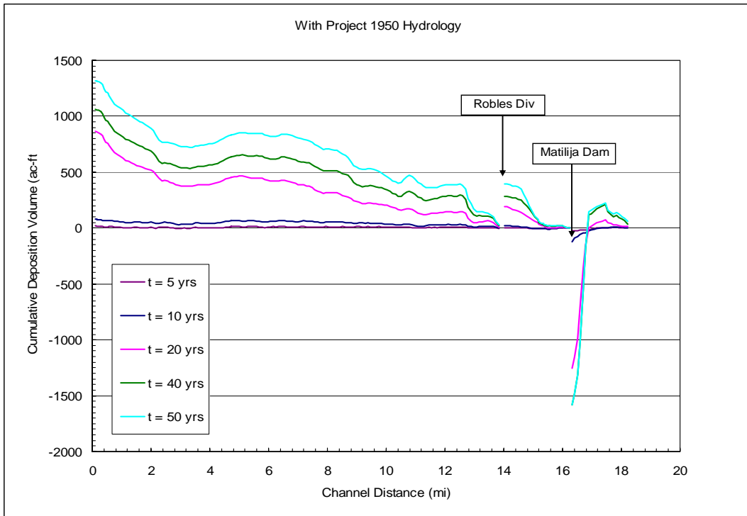
Figure 11.19. Cumulative Deposition for 1950 historical 50-yr hydrograph for With- Project Conditions.
