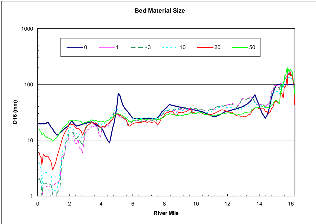
Figure 11.26. Bed Material Size following Dam Removal. D16 is the diameter of which 16% of the bed material is finer.
