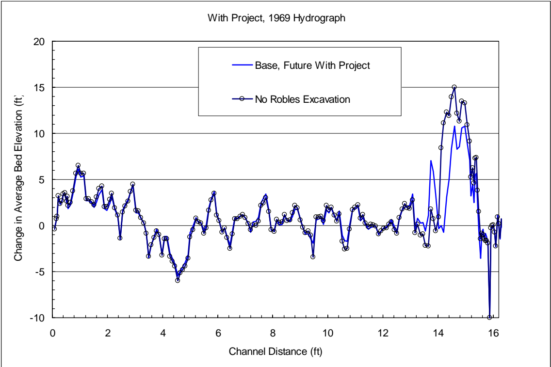
Figure 12.13. Affect of not Excavating Sediment at Robles Diversion.
