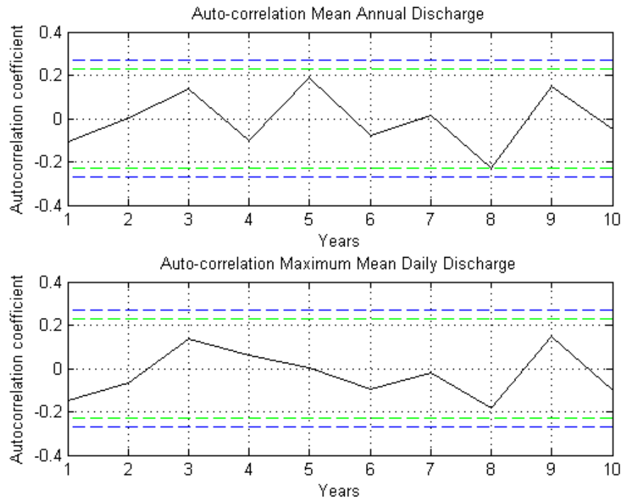
Figure 6.4. Gage 11117500 autocorrelation structure.
