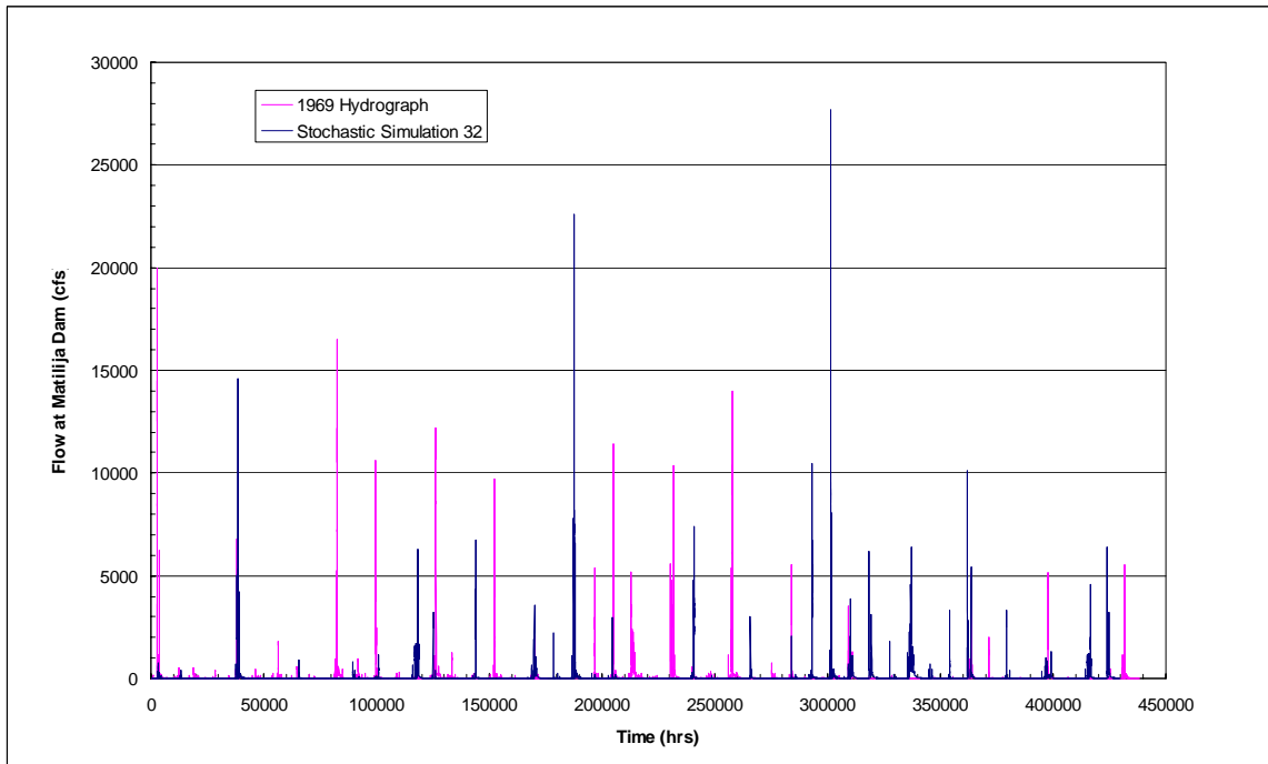
Figure 6.8. Sample Hydrograph Traces as Compared to 1969 Hydrology.
