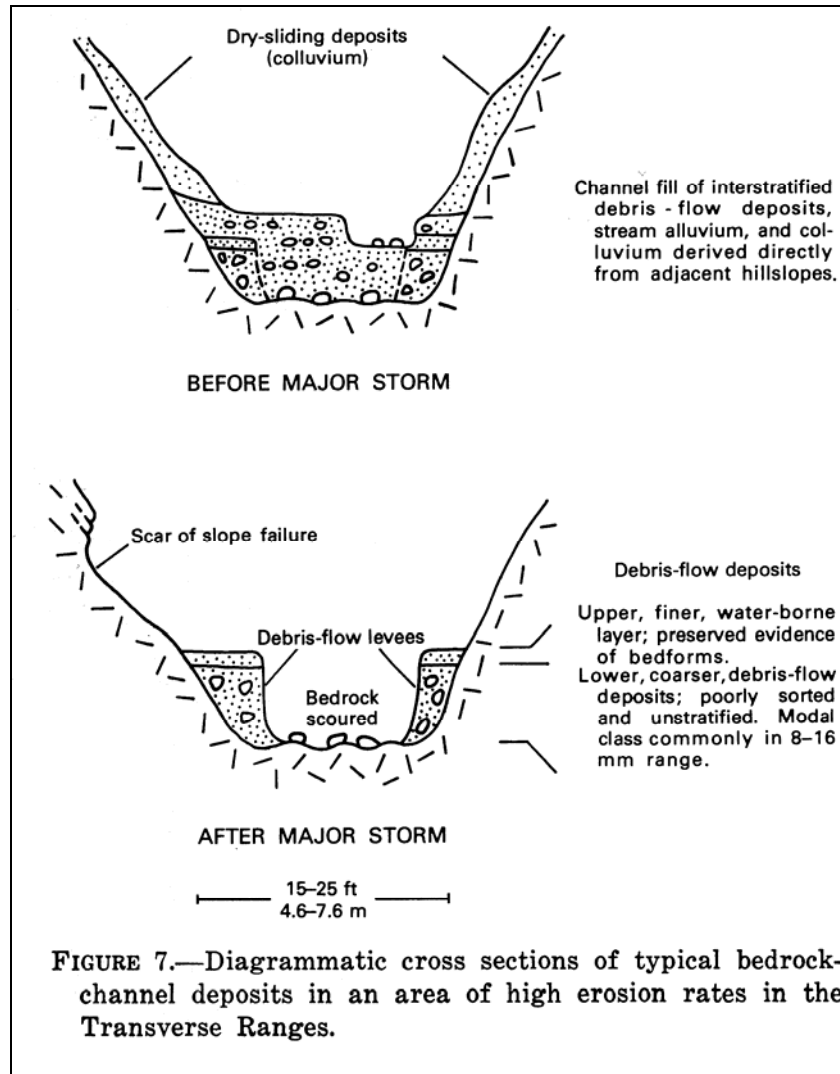
Figure 5.1. Figure 7 from Scott and Williams. The figure shows cause of sediment transport in small watersheds being dependent upon the previous hydrology.
