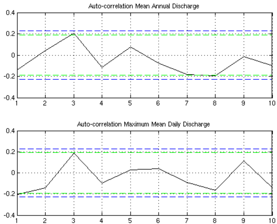
Figure 6.5. Gage 11118500 autocorrelation structure.
