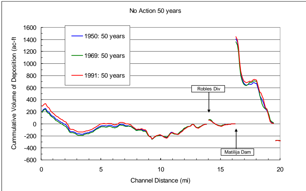
Figure 11.12. Cumulative Deposition in 50 years for Without-Project Conditions for different hydrographs.
