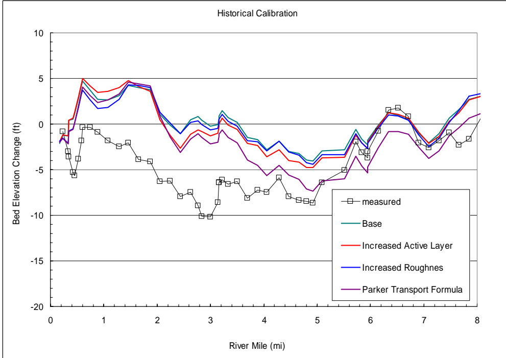
Figure 6.23. Sensitivity of Model Results to Various Model Parameters, RM 8 to 0.
