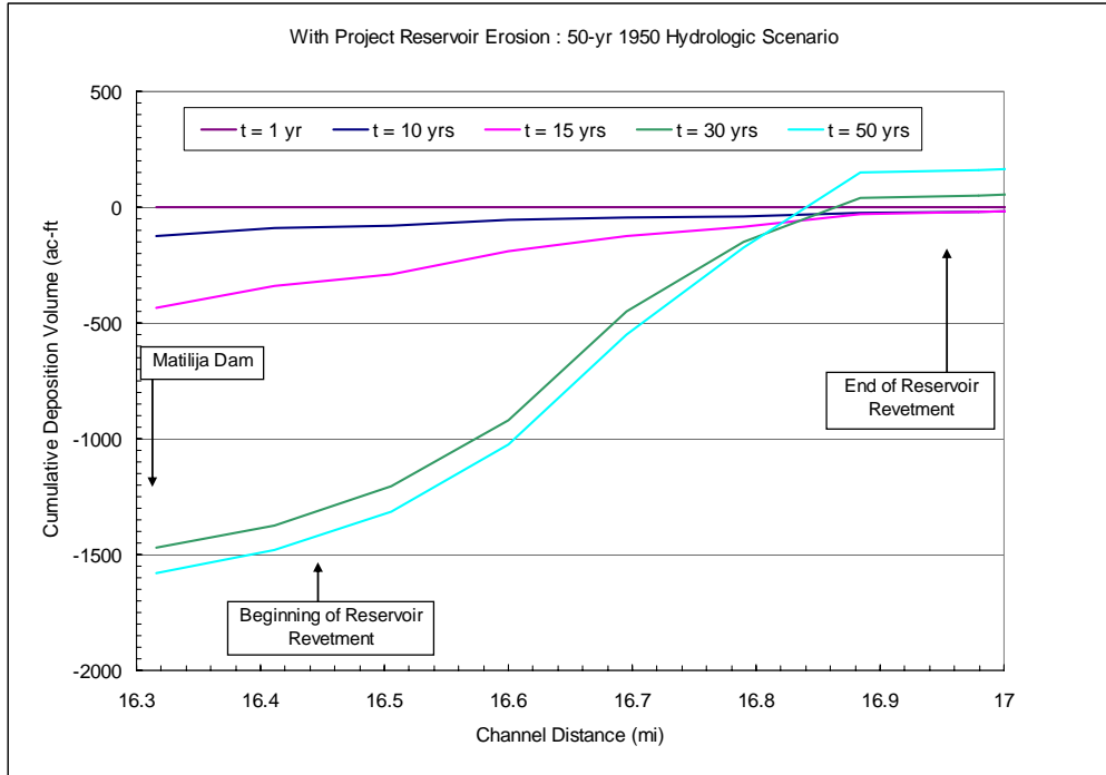
Figure 11.6. Erosion of Sediment from Matilija Reservoir under With-Project Conditions and 50-yr 1950 Hydrologic Scenario.
