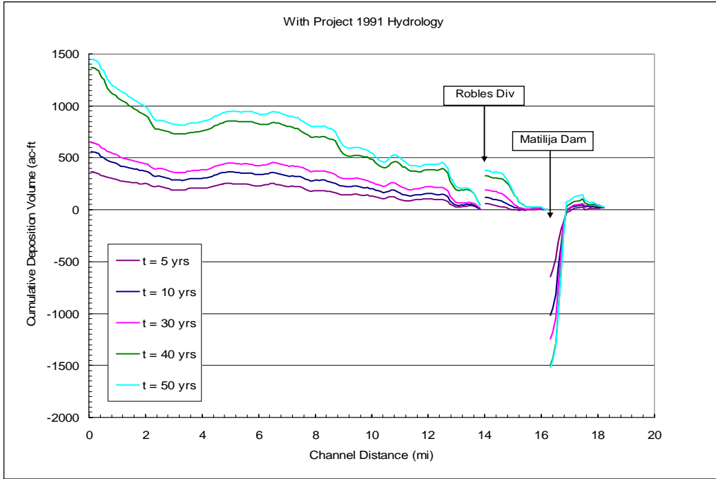
Figure 11.18. Cumulative Deposition for 1991 historical 50-yr hydrograph for With- Project Conditions.
