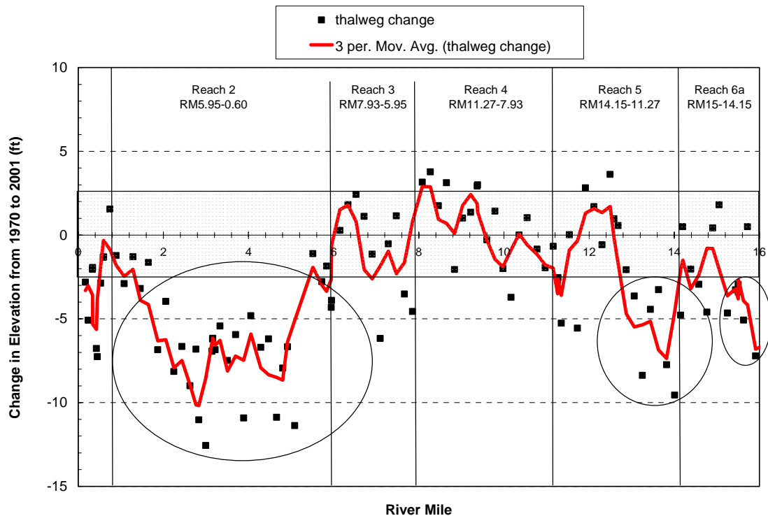
Figure 5.31. Comparison of change in thalweg elevation between 2001 and 1970. Negative changes indicate areas of degradation in the channel bed. Positive changes indicate areas that have aggraded. Areas within 2.5 feet of change are considered to be within the error range of the 1970 data.
