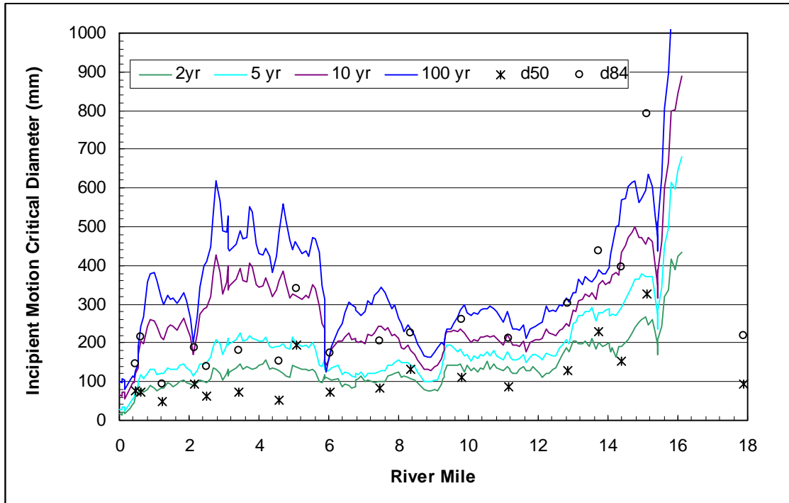
Figure 5.25. Incipient motion critical diameter for the Ventura River and comparison with the d_{50} and d_{84} of the bed material.
