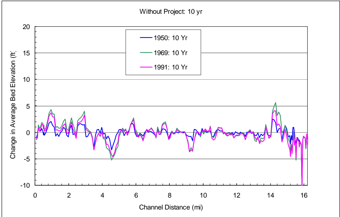
Figure 11.17. Average bed elevation changes at the end of the 10-yr simulations for the 1950, 1969, and 1991 50-yr hydrographs for Without Project Conditions.
