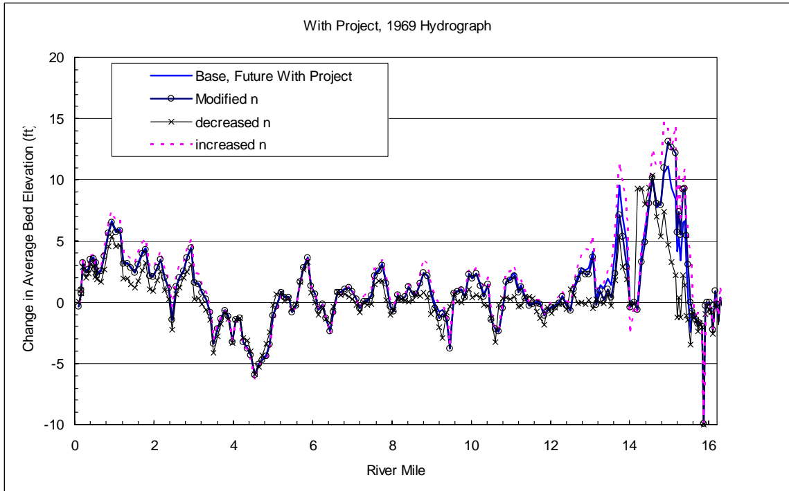
Figure 12.9. Affect of Manning's Roughness Coefficient on Average Bed Elevations for 1969 Hydrograph.
