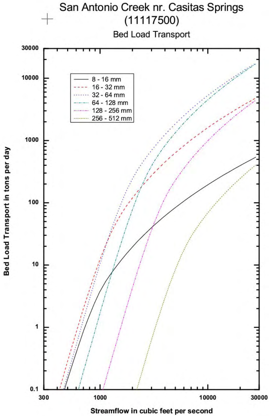
Figure 5.21. Computed Bed Load Transport on San Antonio Creek.
