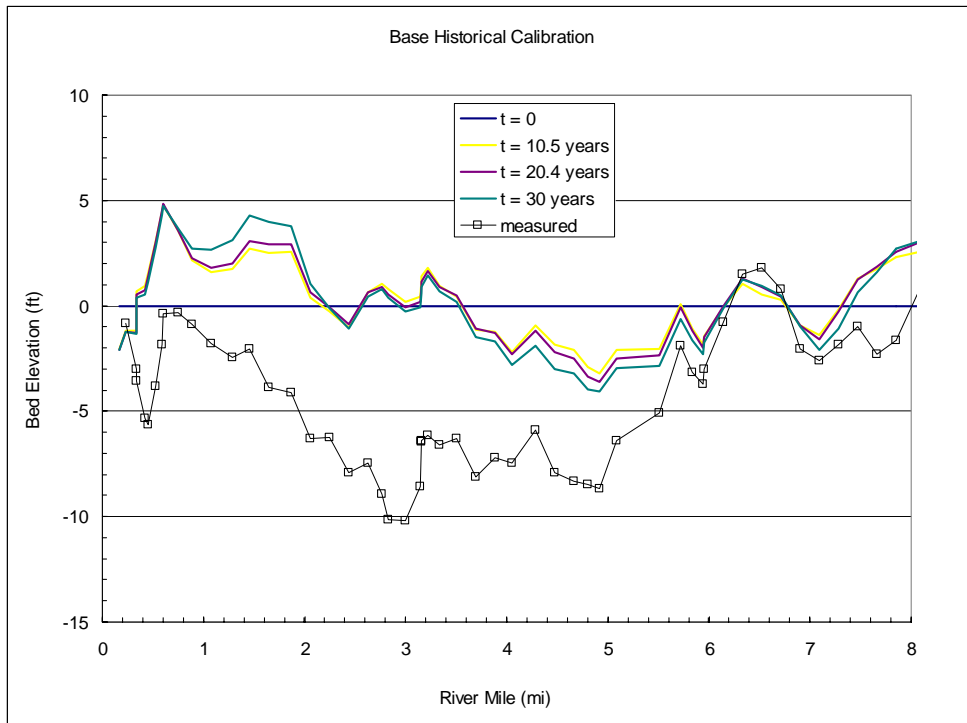
Figure 6.17. Computed Thalweg Elevation Change from 1971 to 2001, RM 0 – 8.
