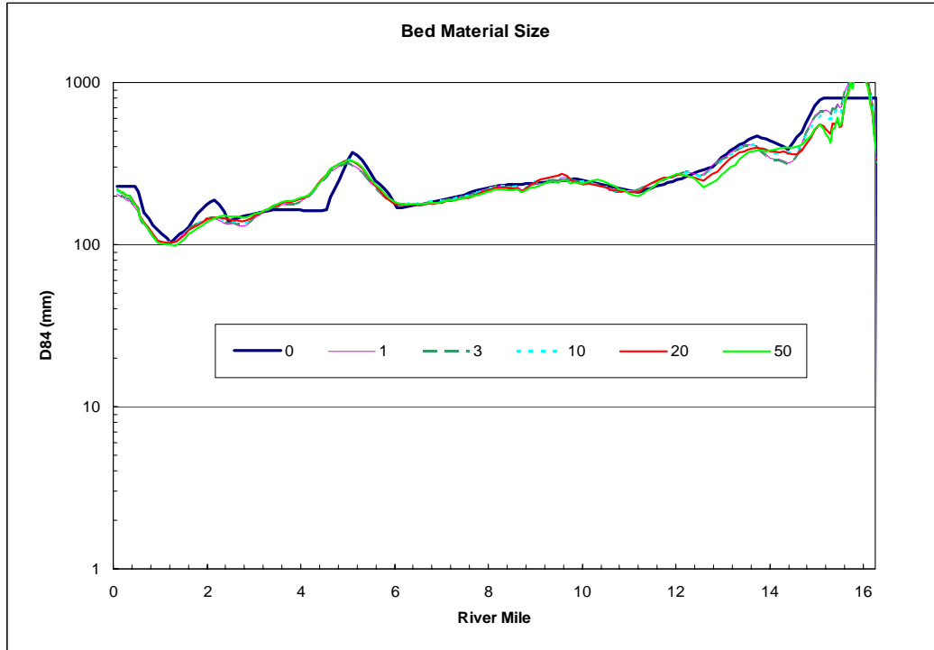
Figure 11.28. Bed Material Size following Dam Removal. D84 is the diameter of which 84% of the bed material is finer.
