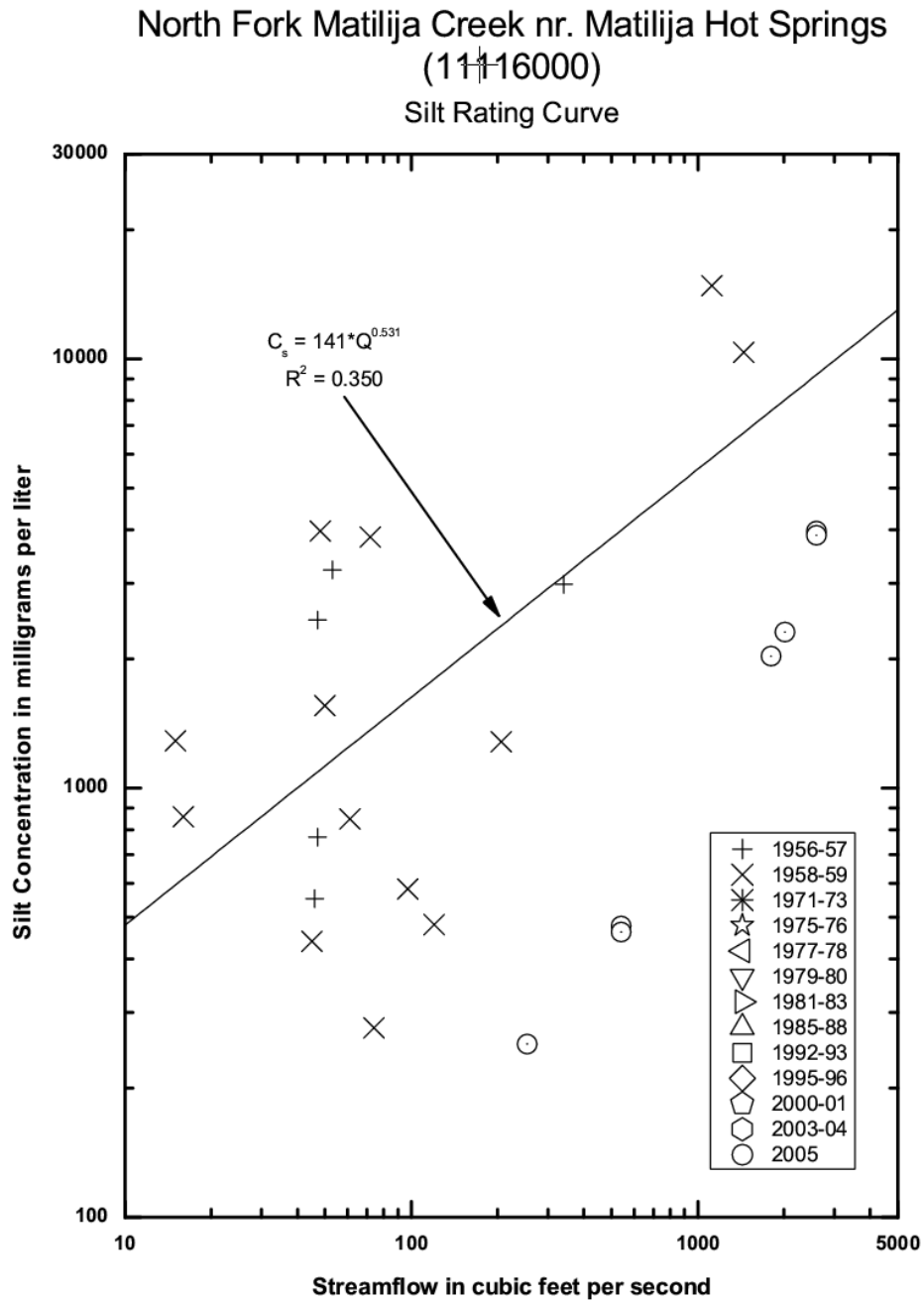
Figure 5.16. Silt Concentration on North Fork Matilija Creek.
