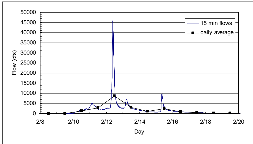
Figure 2.2. Comparison of 15-minute instantaneous hydrographs and daily average hydrographs for the 1992 flood at Foster Park gage on the Ventura River (USGS gage 11118500).
