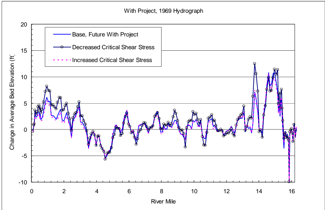
Figure 12.10. Affect of Non-Dimensional Critical Shear Stress on Average Bed Elevations for 1969 Hydrograph.
