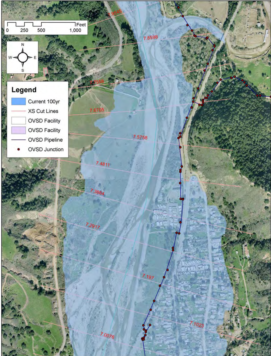
Figure 4.19. 100-yr floodplain from RM 8 to RM 7. Locations of OVSD Pipelines are shown.
