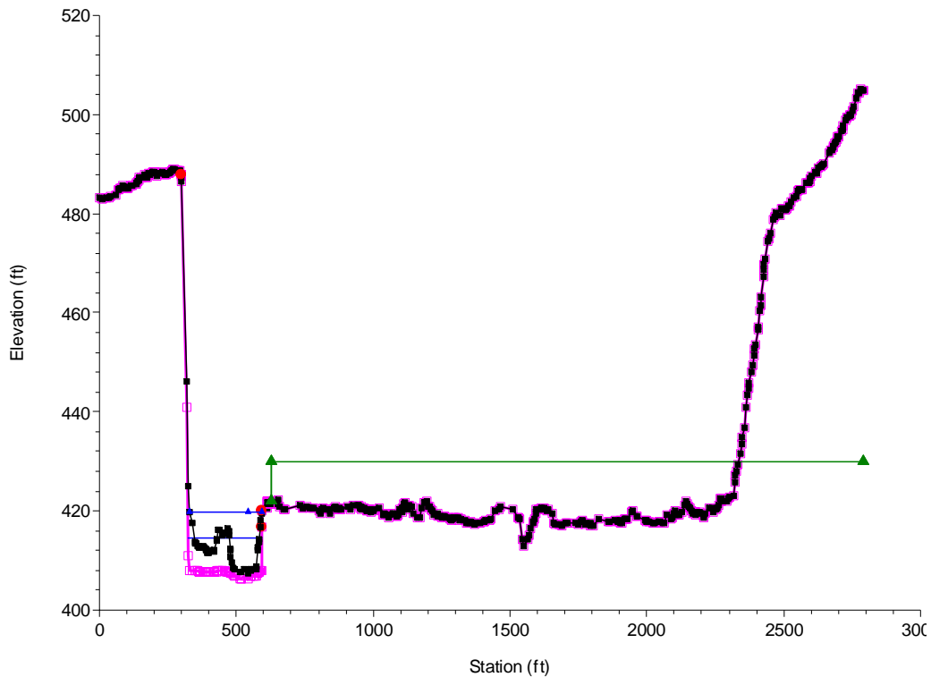
Figure 11.14. Bed Elevation Changes upstream of Santa Ana Bridge under Without-Project Conditions.
