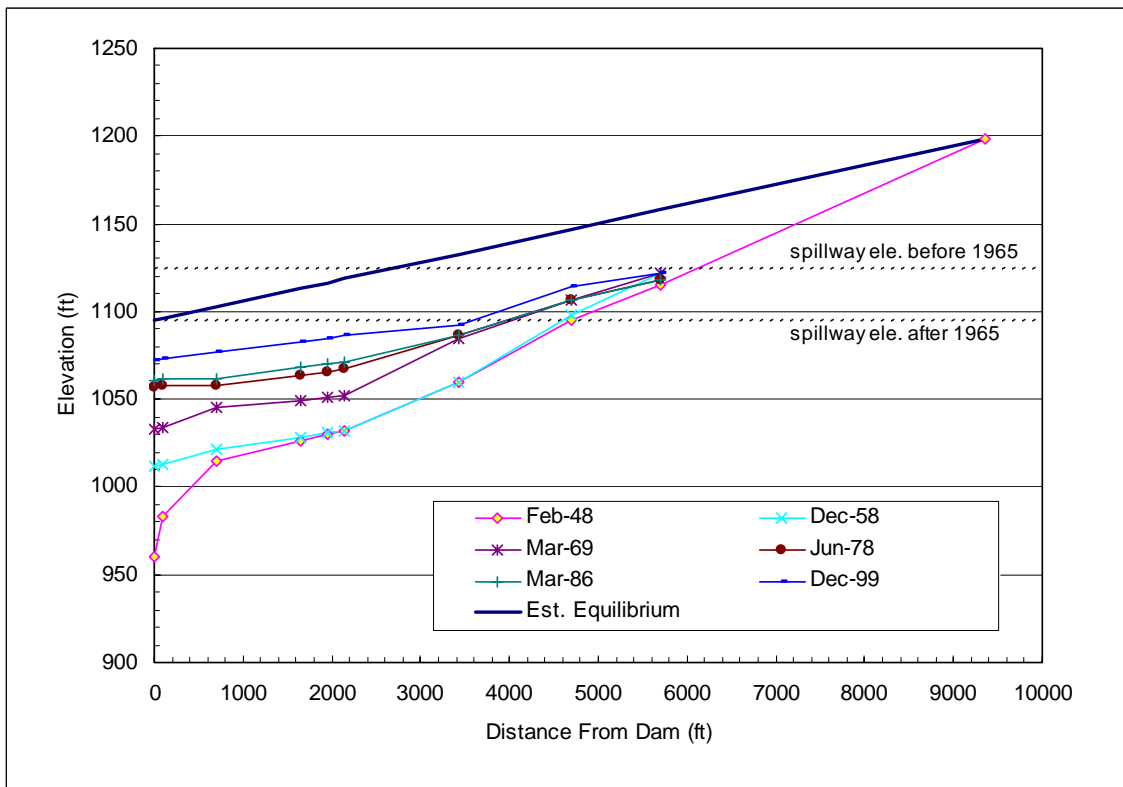
Figure 5.13. Profile plot of depositional history.
