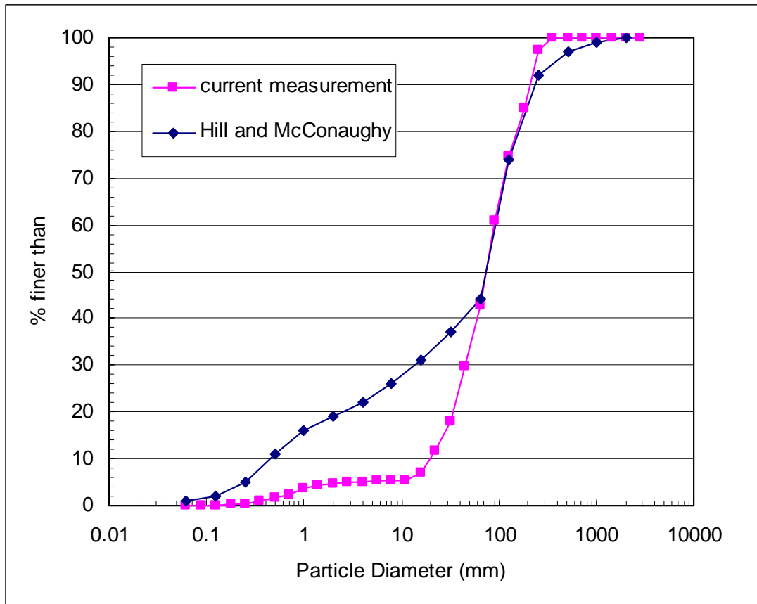
Figure 5.9. Comparison between USGS Composite Sample and Current Measurements of Bed Material near USGS Gage on the Ventura River near Foster Park.
