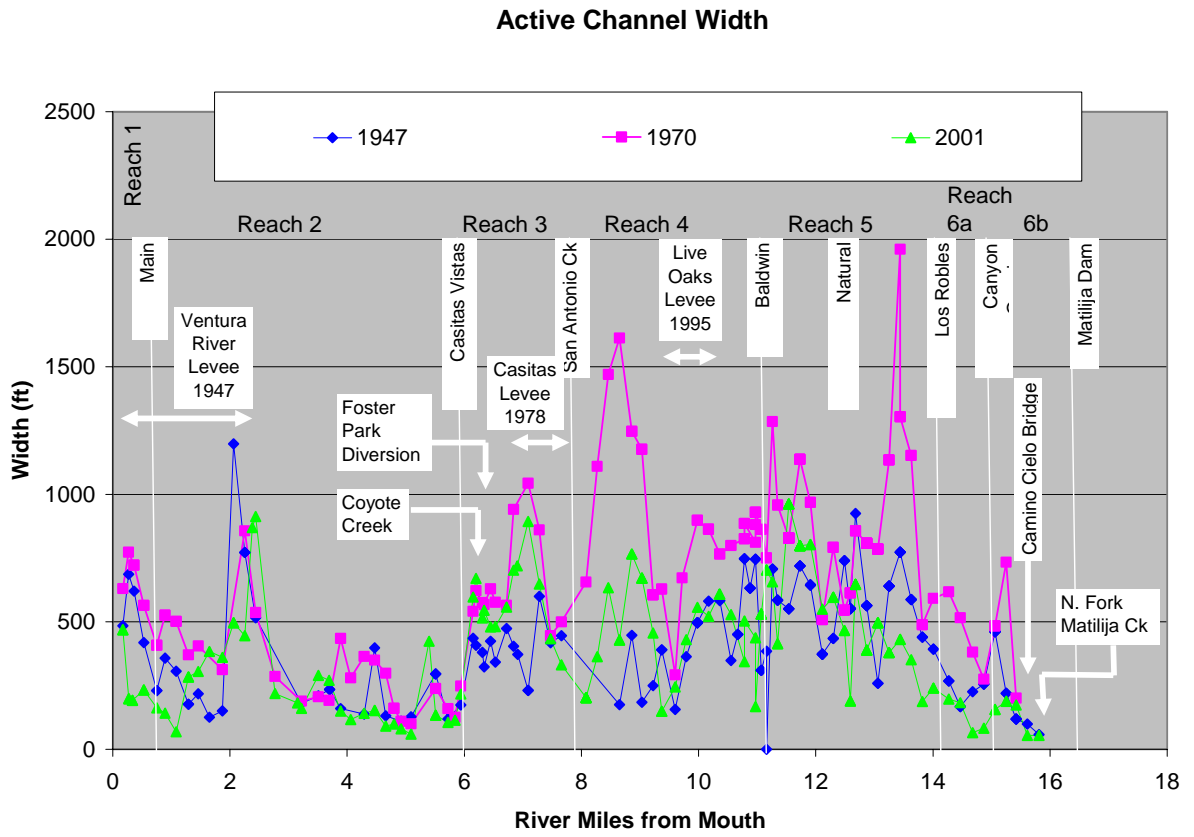
Figure 5.33. Historical Active Channel Widths of the Ventura River in 1947, 1970, and 2001.
