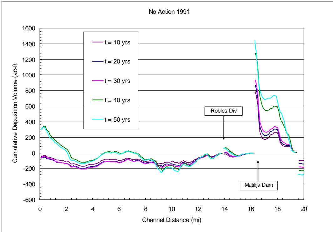
Figure 11.9. Cumulative Deposition for 1991 historical 50-yr hydrograph for Without Project Conditions.
