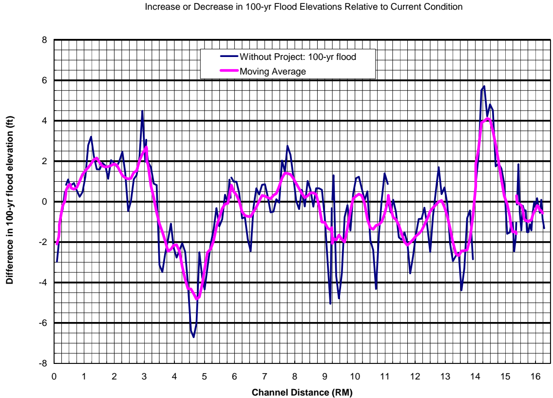
Figure 10.1. Change in 100-yr flood elevations between Current Condition and Future Without-Project Conditions.
