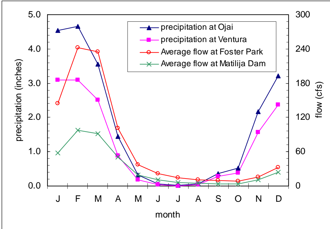
Figure 1.6. Seasonal variation of average rainfall and flow in Ventura River Watershed.
