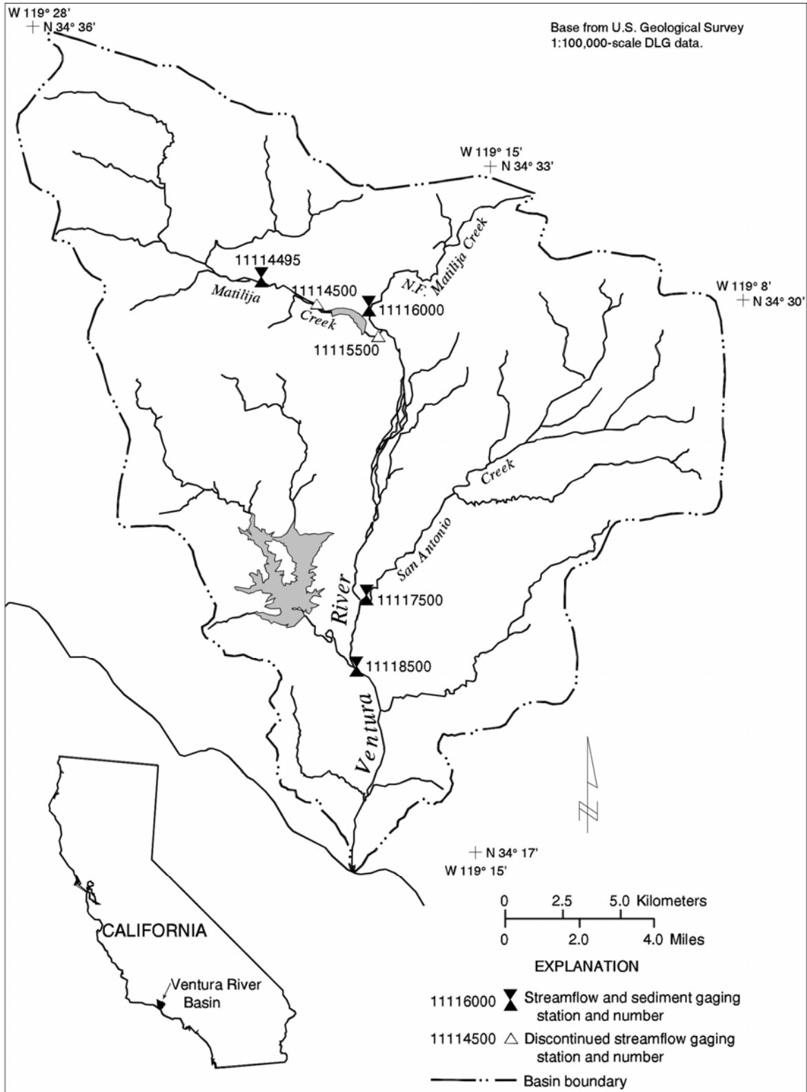
Figure 2.1. Map of Stream Gages in Ventura Watershed.
