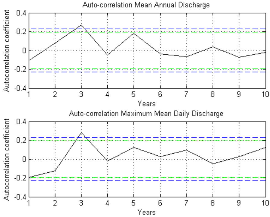
Figure 6.2. Gage 11115500 autocorrelation structure.
