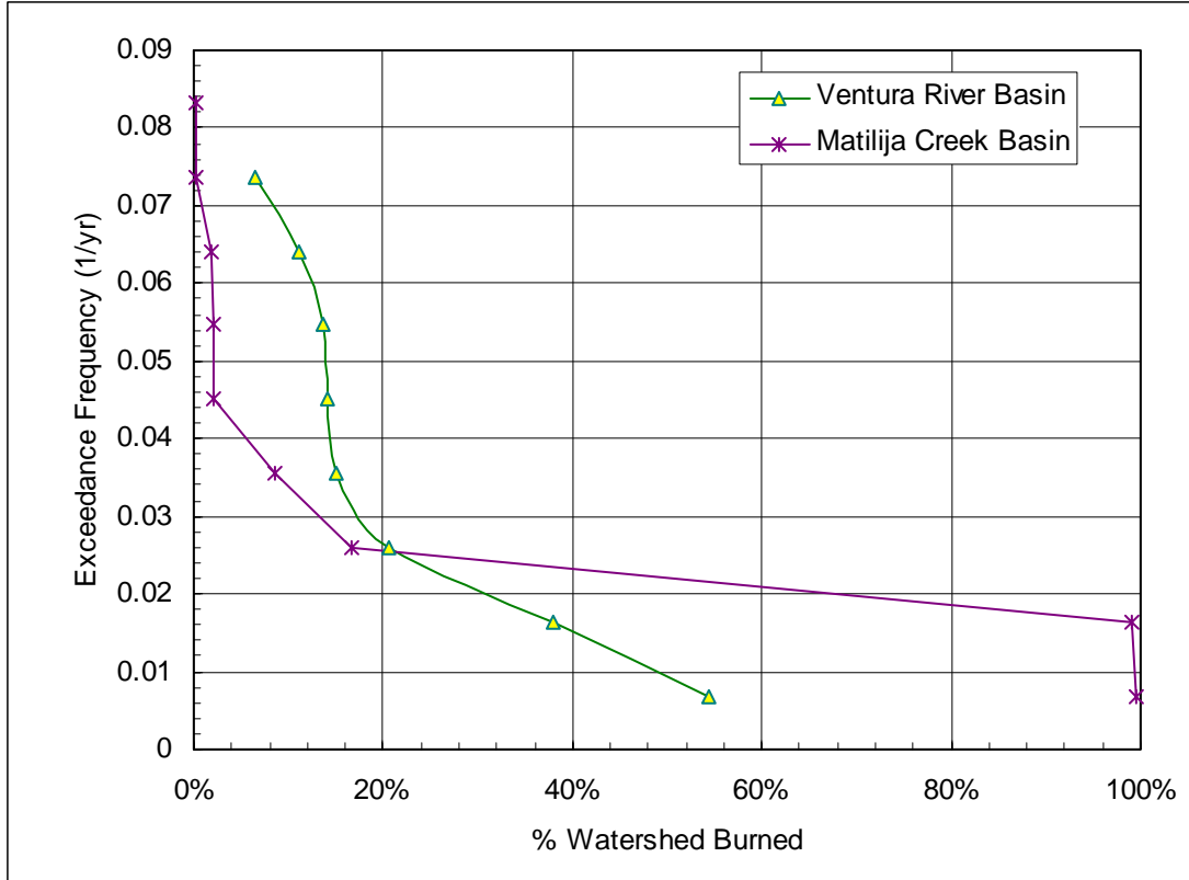
Figure 5.24. Fire frequency in the Matilija Creek and Ventura River Watersheds.
