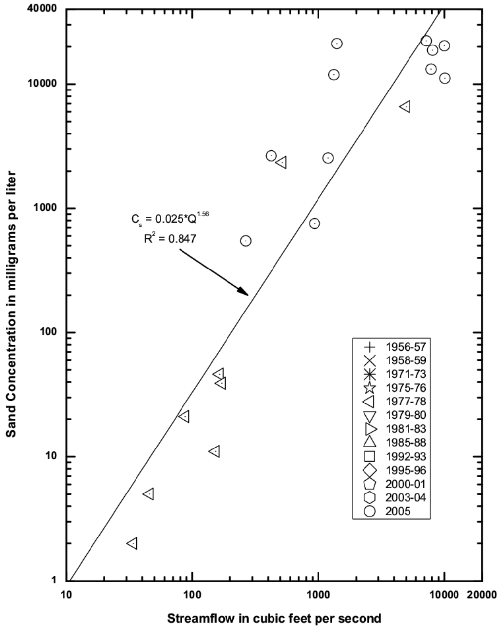
Figure 5.20. Sand Concentration on San Antonio Creek
