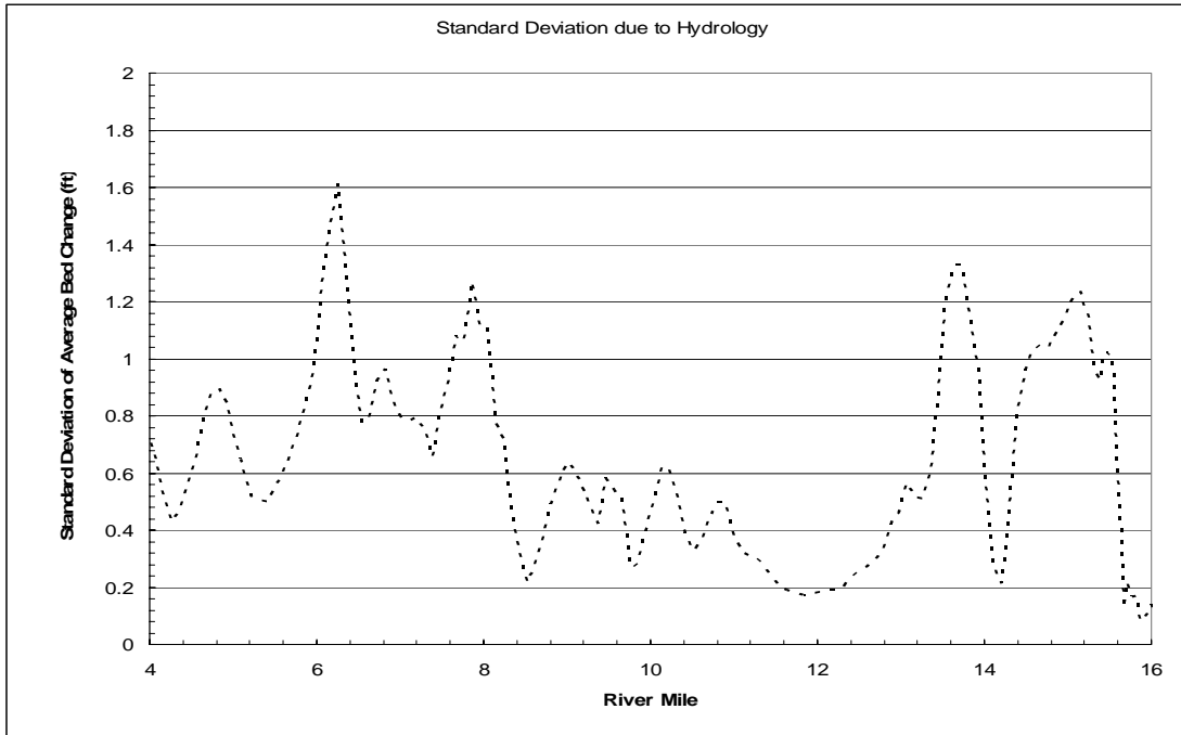
Figure 12.4. Standard Deviation in the Average Bed Elevation Changes due to Hydrologic Variability.
