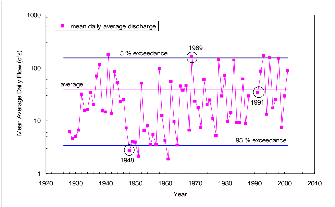
Figure 2.9. Analysis of mean daily average flows at USGS gage 11115500, downstream of Matilija Dam on Matilija Creek.
