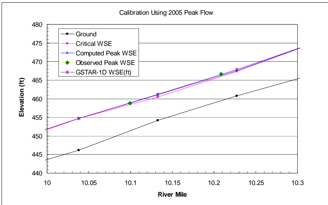
Figure 4.4. Plot of observed and computed peak water surface elevations at the Levee near Live Oak.
