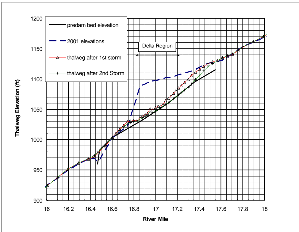
Figure 6.14. Thalweg elevations through reservoir region for Alternative 2a after the simulation of the 1998 flood twice in succession.
