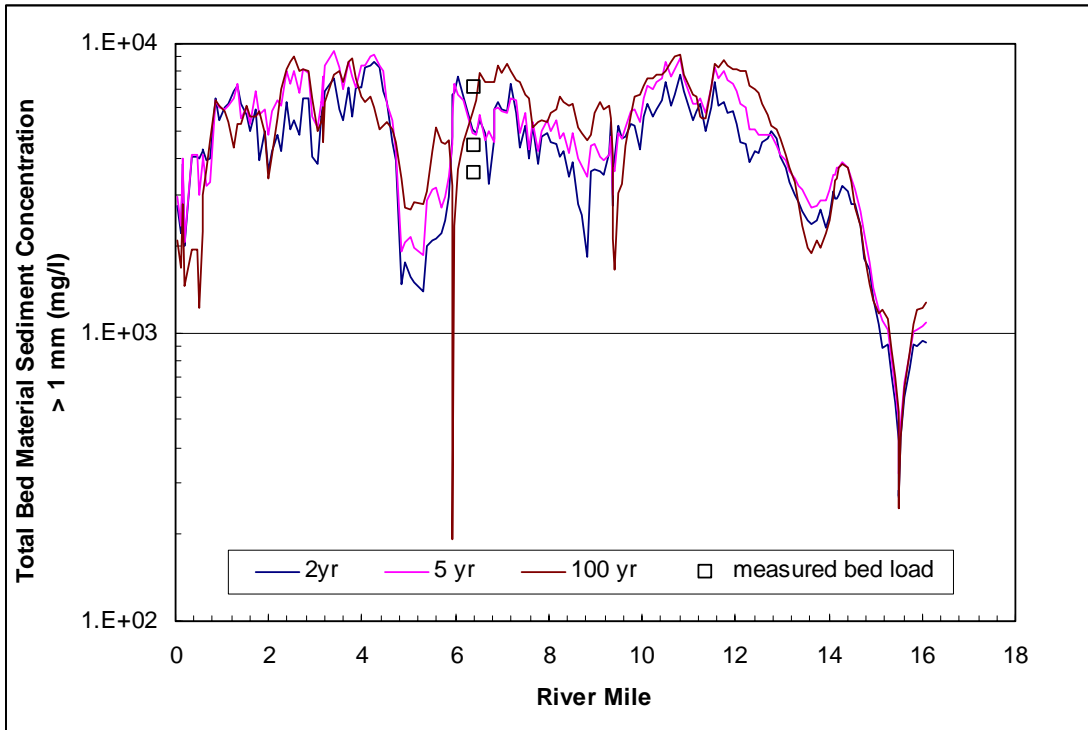
Figure 5.29. Bed material sediment capacity concentration of sediment sizes greater than 1 mm, for the Ventura River using Meyer-Peter-Müller sediment transport equation.
