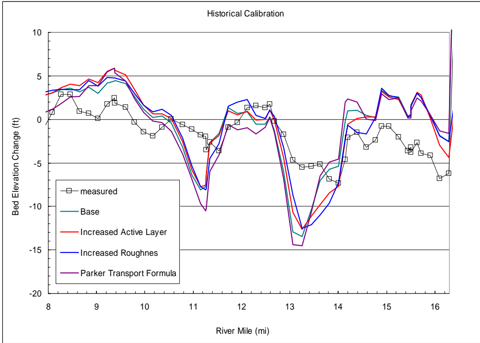
Figure 6.22. Sensitivity of Model Results to Various Model Parameters, RM 16 to 8.
