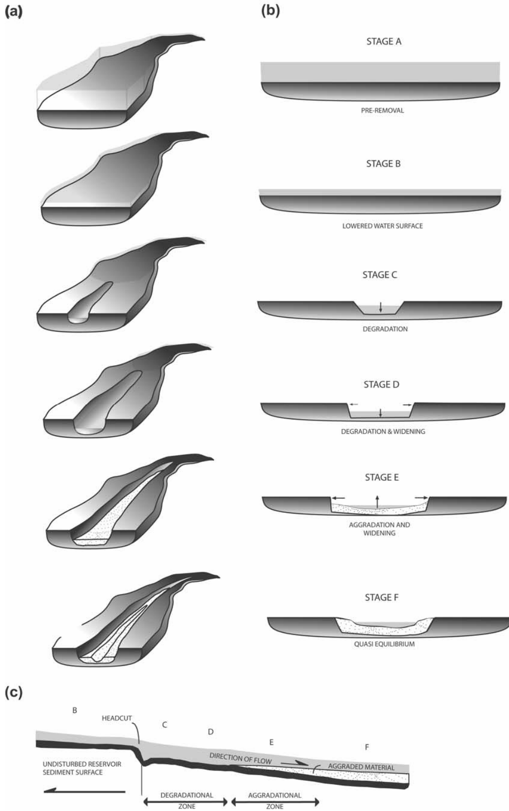
Figure 6.13. Schematic description of reservoir erosion process through delta deposits, from Doyle et al. (2003). (a) oblique view, (b) cross section view, (c) profile view.
