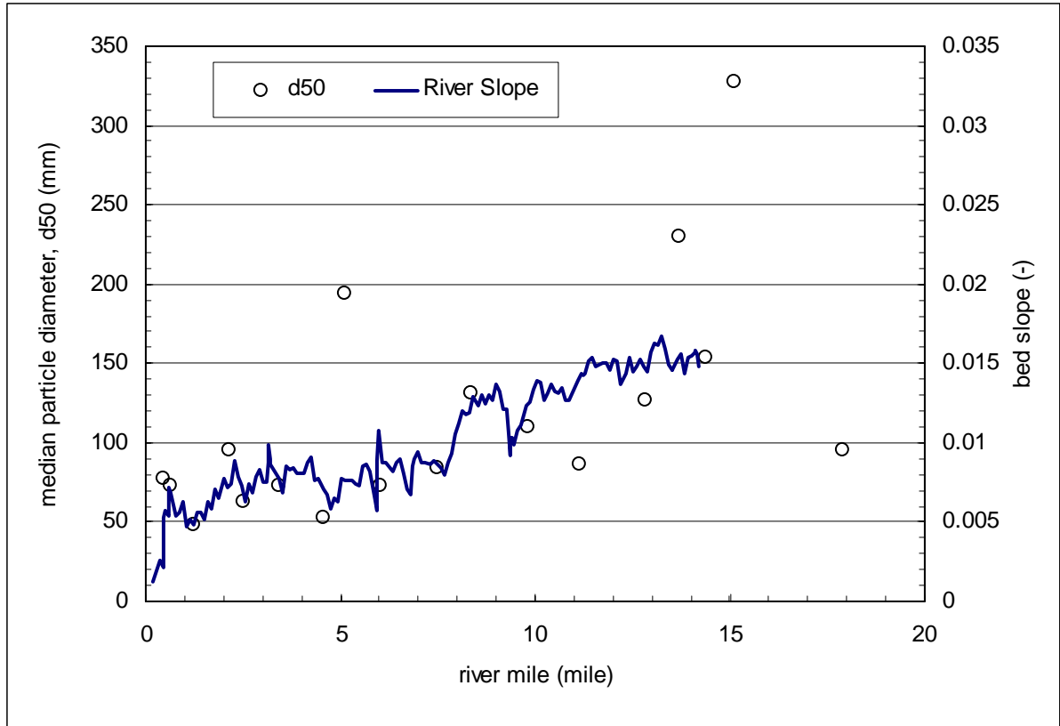
Figure 5.7. Average Bed Slope and d_{50} of Bed Material Samples.
