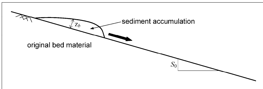
Figure 12.1. Schematic of idealized representation of the movement of a sediment accumulation, from Greimann et al. (2006).
