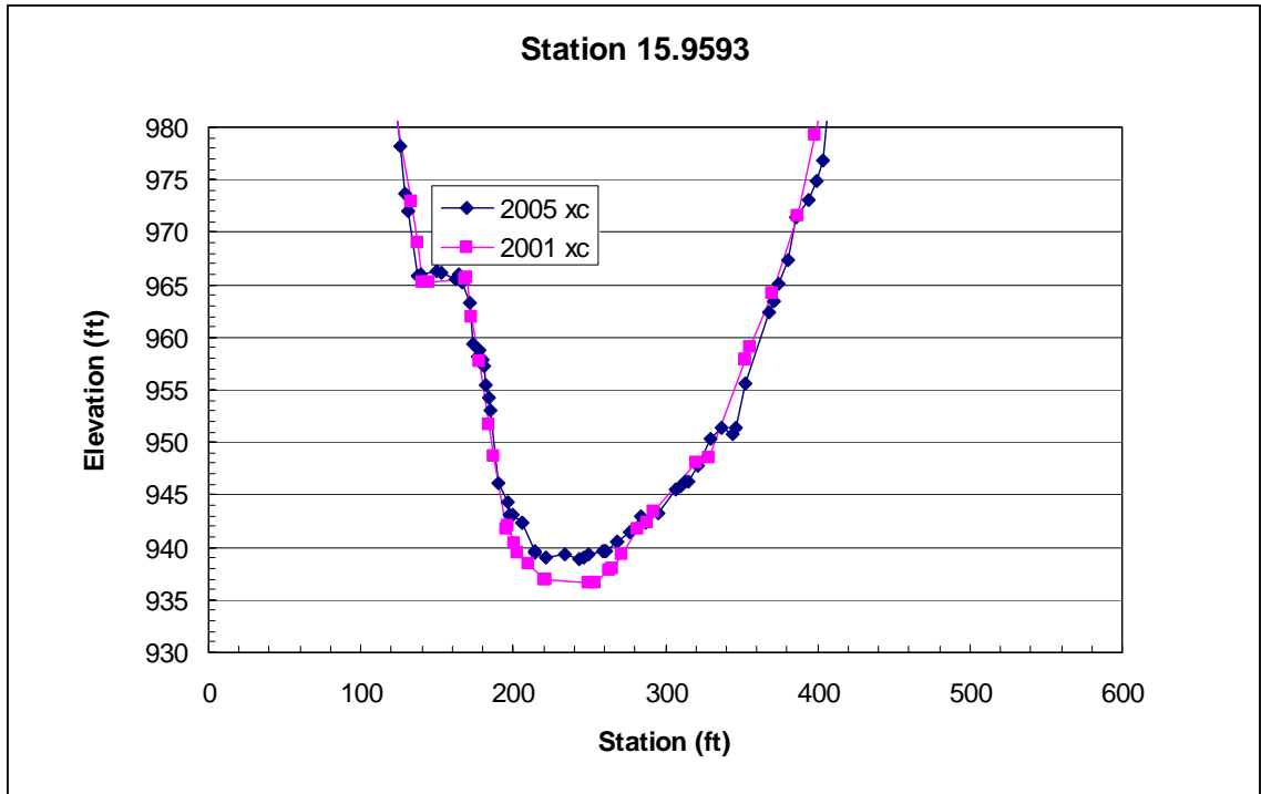
Figure 4.1. Comparison between 2001 and 2005 aerial surveys at Station 15.9593.
