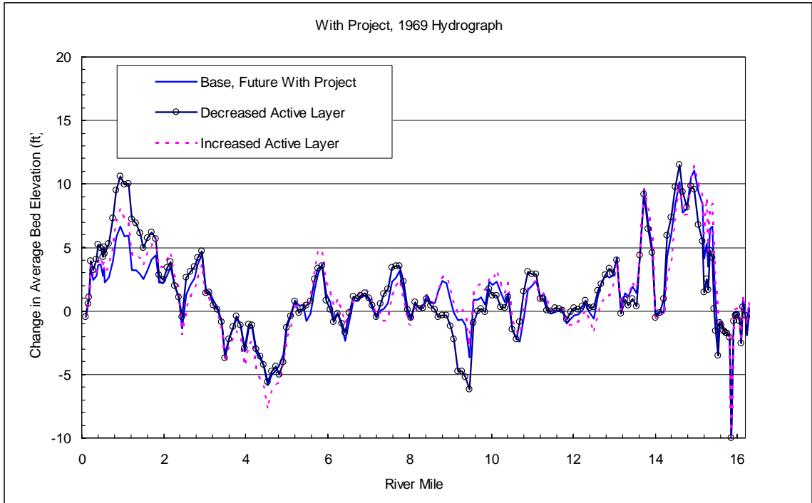
Figure 12.8. Affect of Active Layer on Average Bed Elevations for 1969 Hydrograph.
