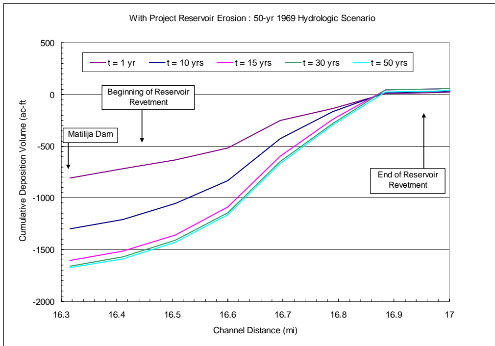
Figure 11.7. Erosion of Sediment from Matilija Reservoir under With-Project Conditions and 50-yr 1969 Hydrologic Scenario.
