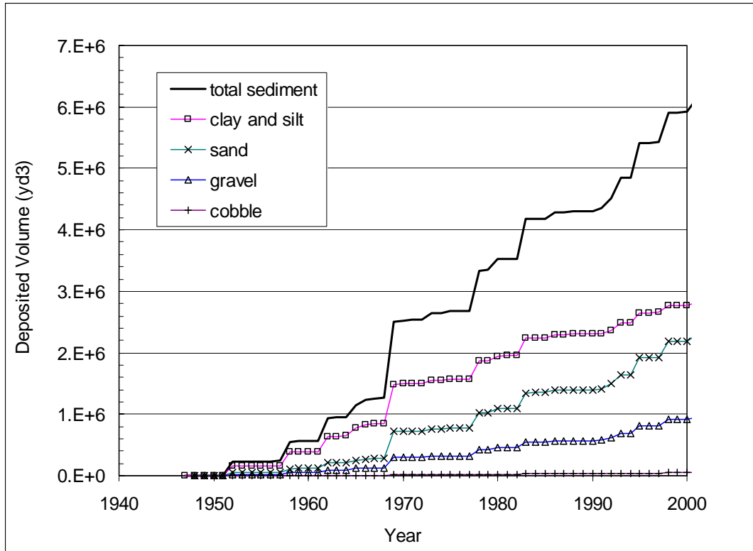
Figure 6.9. Simulated deposition in Matilija Reservoir using sediment rating curve for Matilija Creek.
