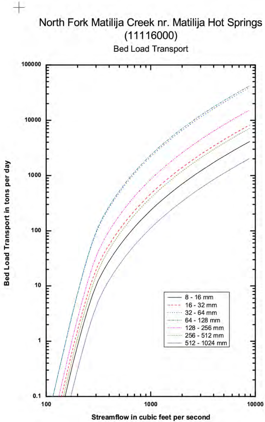
Figure 5.18. Computed Bed Load Transport on North Fork Matilija Creek.
