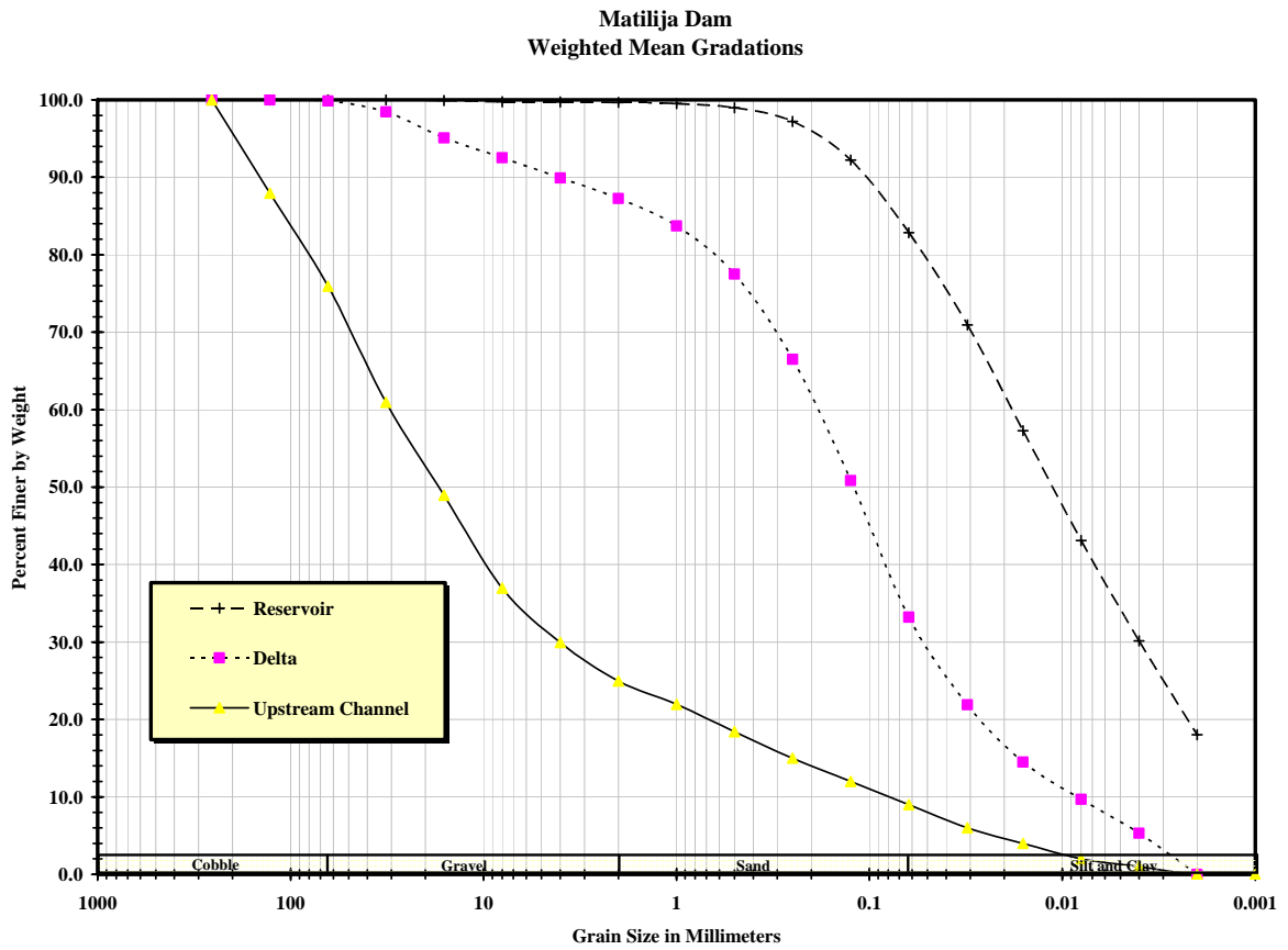
Figure 5.14. Average size gradations of reservoir deposits.
