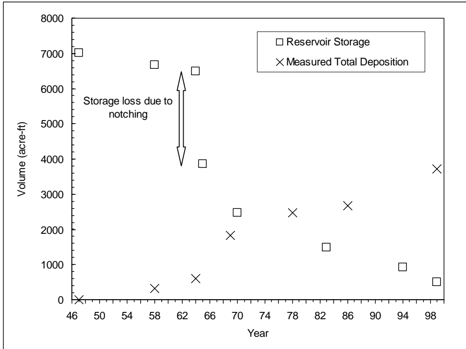
Figure 5.12. Plot of Matilija reservoir storage and deposition.
