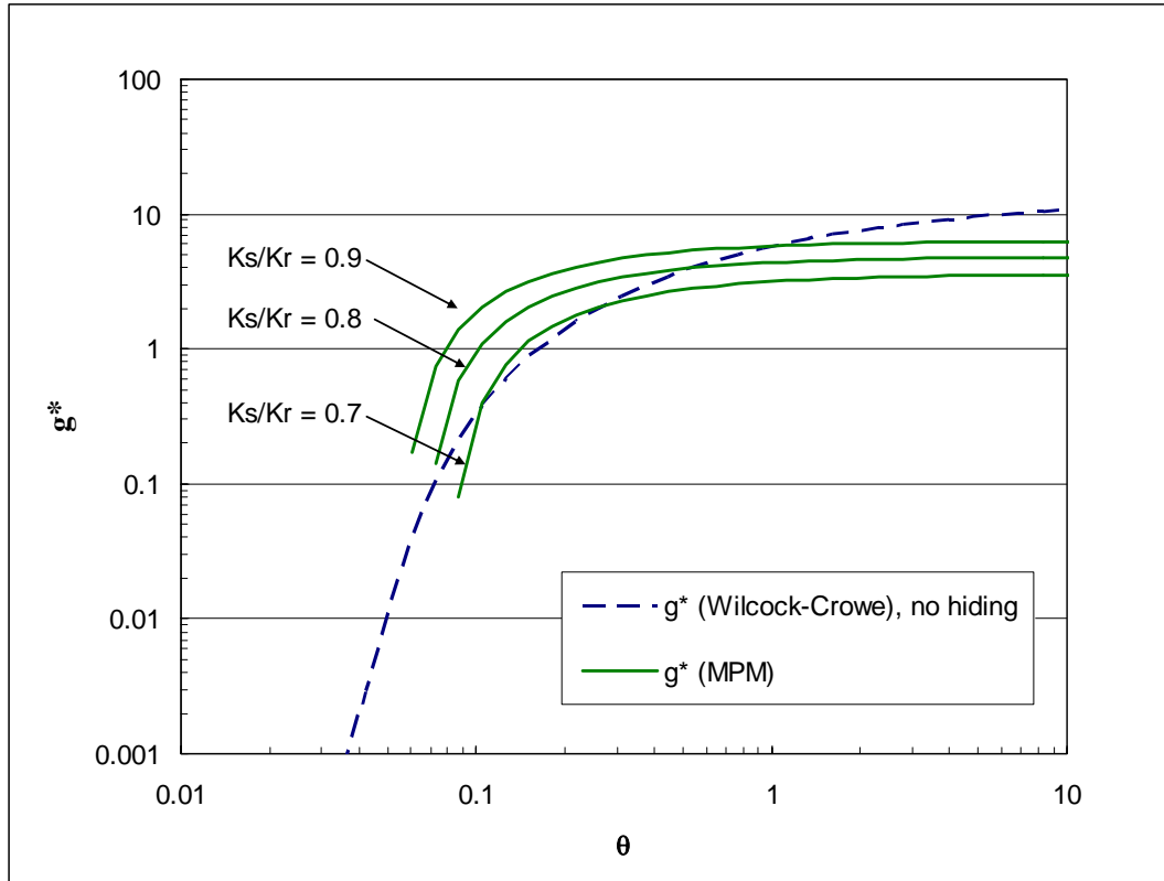
Figure 6.12. Comparison between the Wilcock and Crowe method and the Meyer-Peter-Muller Method (MPM).
