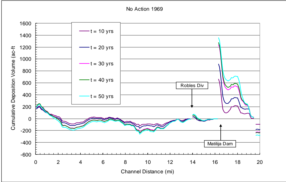
Figure 11.11. Cumulative Deposition for 1969 historical 50-yr hydrograph for Without Project Conditions.
