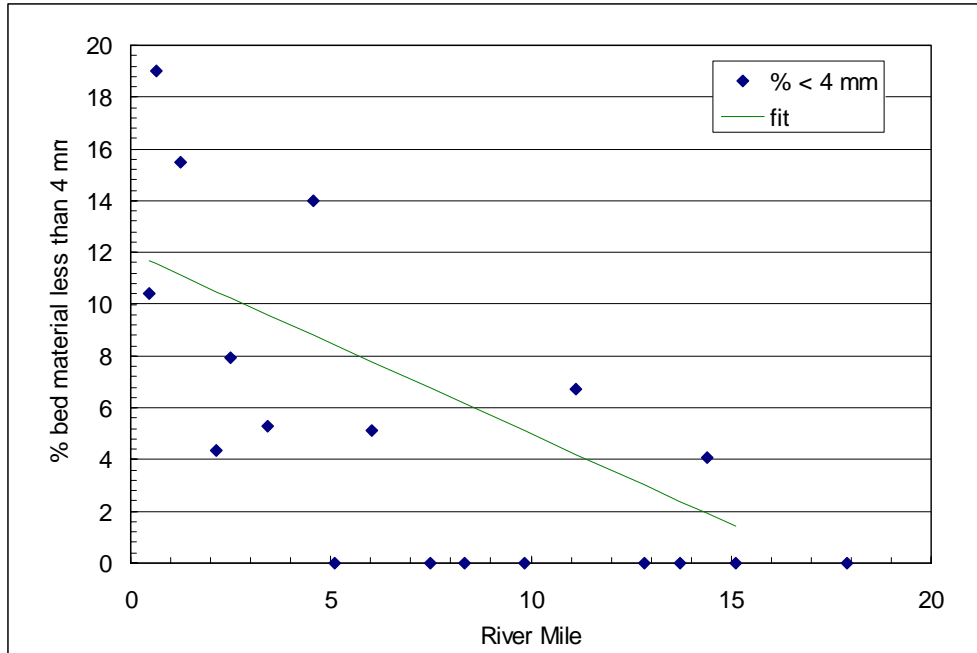
Figure 5.8. Fraction of Bed Material Less than 4 mm.
