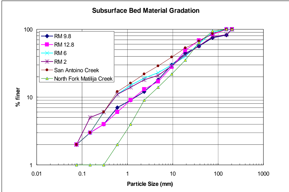
Figure 5.10. Sediment Gradation of Sub-Surface Material in Ventura River.
