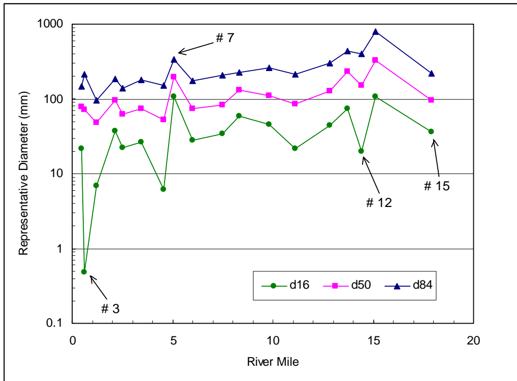
Figure 5.4. Measured representative diameters of surface bed material samples.
