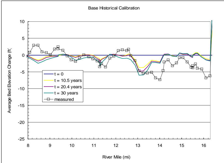
Figure 6.20. Computed Average Bed Elevation Change from 1971 to 2001, RM 8 – 16.
