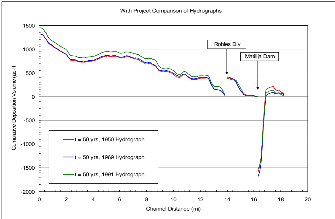
Figure 11.21. Cumulative Deposition in 50 years for With-Project Conditions for different hydrographs.
