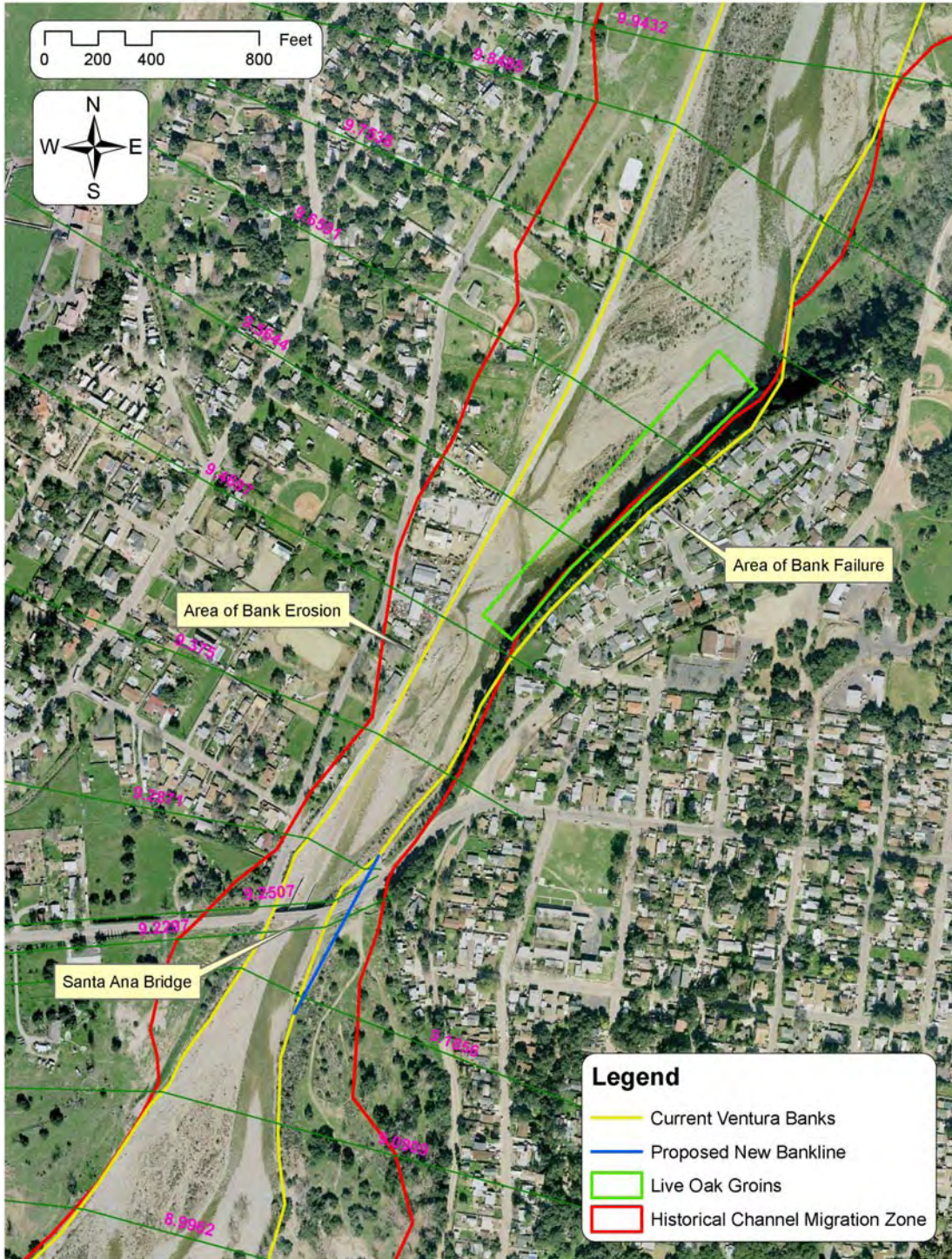
Figure 11.23. Proposed New Bank Link in Vicinity of Santa Ana Bridge. Groins Constructed in 2005 are also Shown.
