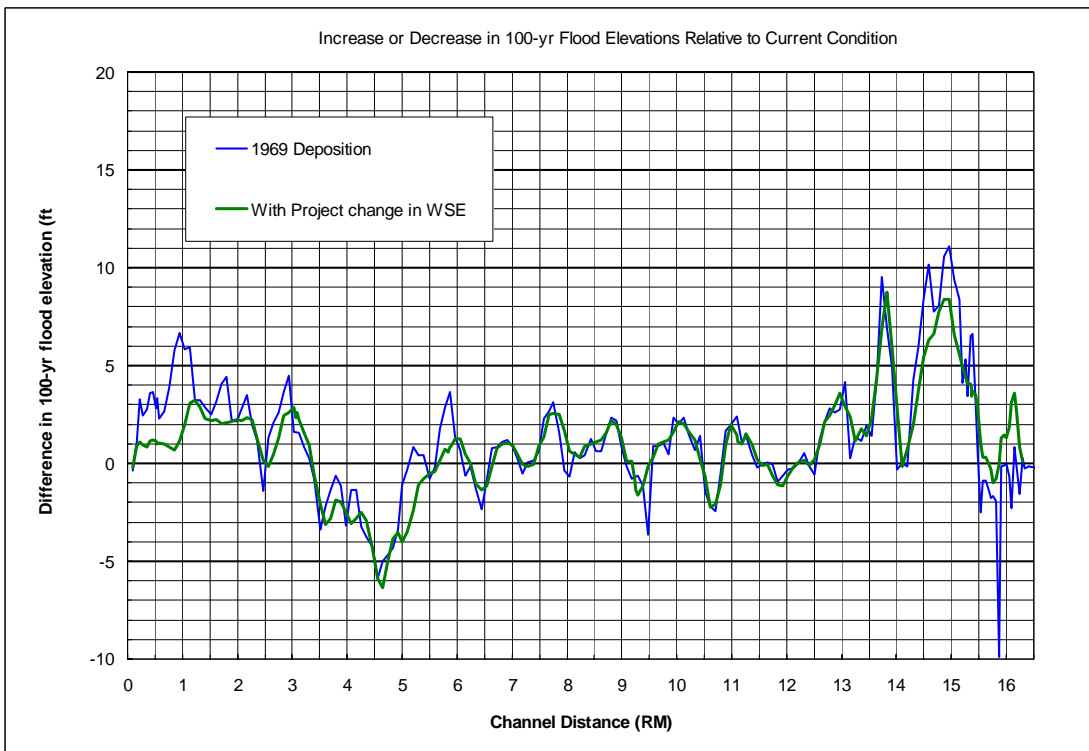
Figure 12.5. Comparison between Average Bed Elevation Change and Change to the 100-yr Water Surface Elevation Change.
