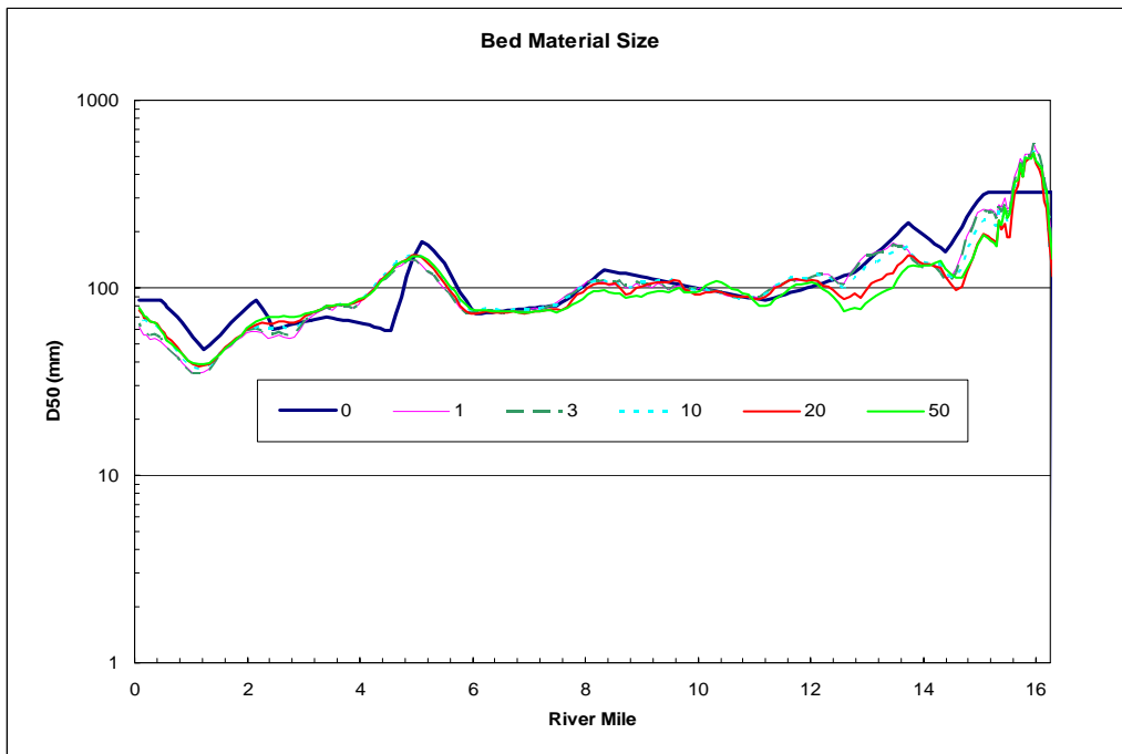
Figure 11.27. Bed Material Size following Dam Removal. D50 is the diameter of which 50% of the bed material is finer.
