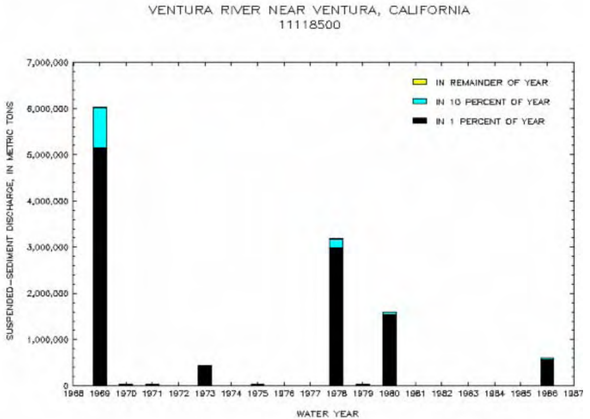
Figure 5.2. Suspended Sediment Loads in Ventura River. There was no data recorded from 10/1/73 to 9/30/74 and from 10/1/82 to 9/30/85 (figure from USGS http://webserver.cr.usgs.gov/sediment/ ). The year 1983 had substantial flow and sediment transport.
