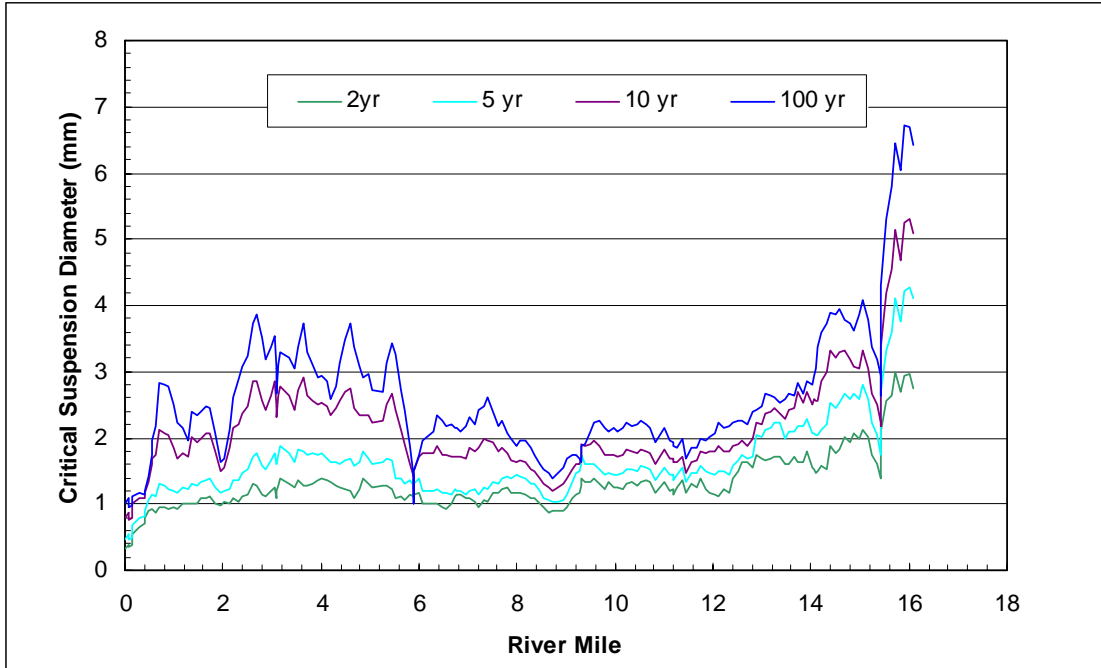
Figure 5.28. Critical suspended diameter along Ventura River for selected floods.
