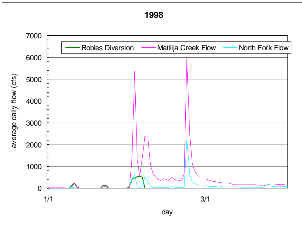
Figure 2.14. Daily average flows at Matilija Creek, North Fork Matilija Creek, and Robles Diversion for the period 1991 to 1998.
