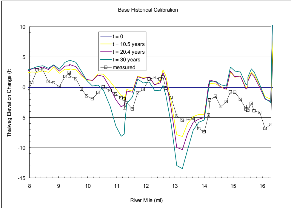
Figure 6.18. Computed Thalweg Elevation Change from 1971 to 2001, RM 8 – 16.
