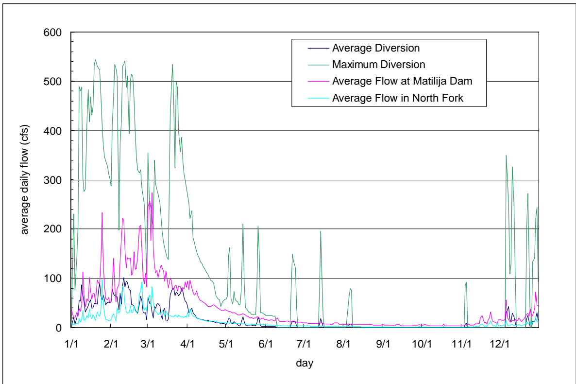
Figure 2.12. Average flow in Matilija Creek, North Fork Matilija Creek, and Robles Diversion.
