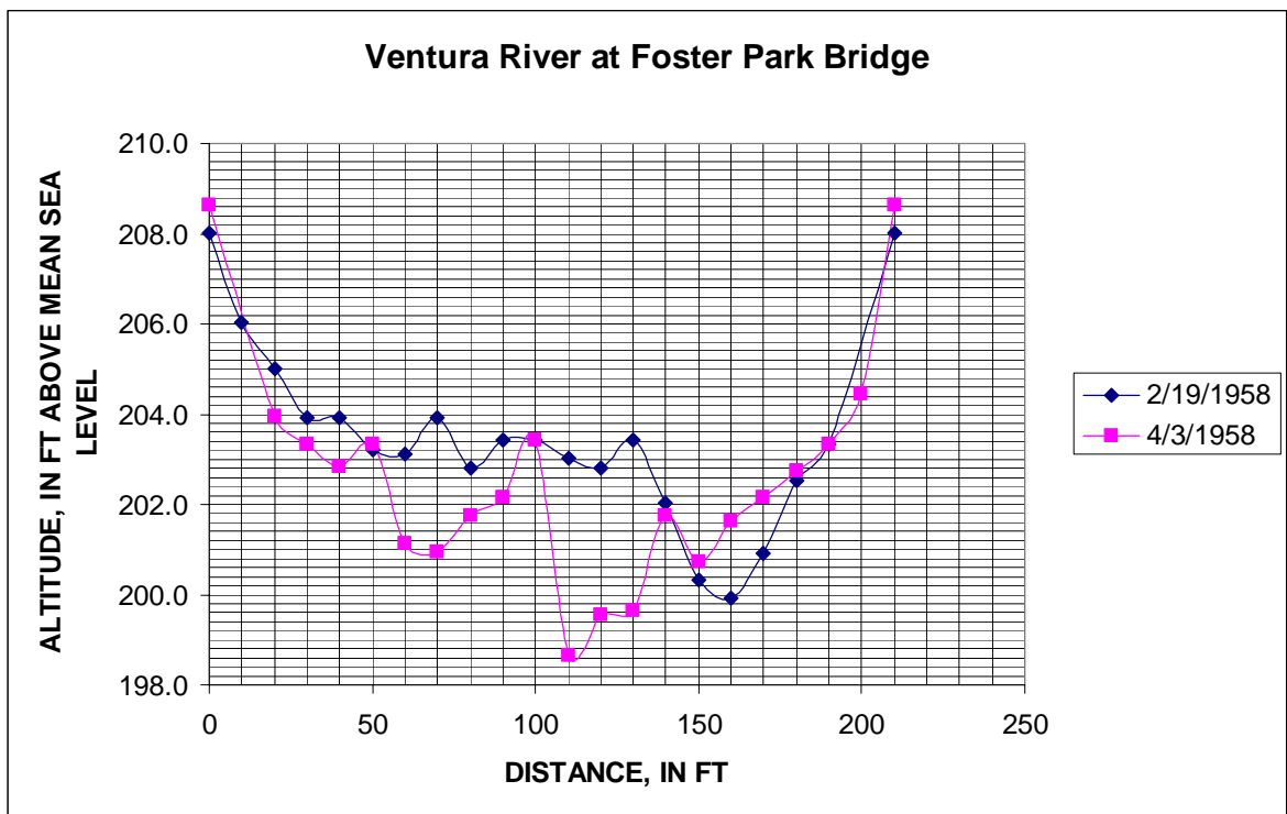
Figure 5.30. Change of Cross Section at Foster Park Bridge due to 1958 flood.
