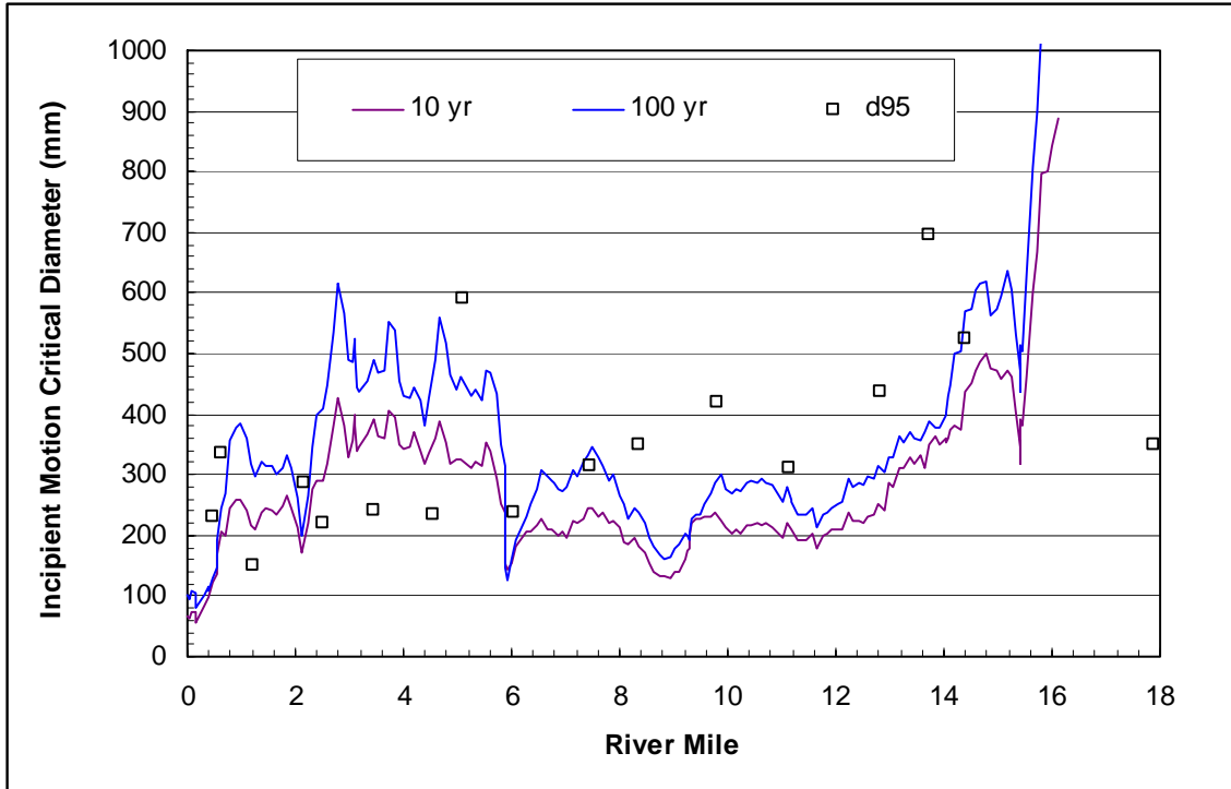
Figure 5.26. Incipient Motion Critical Diameter for 10- and 100-yr Floods, Plotted with d_{95} .
