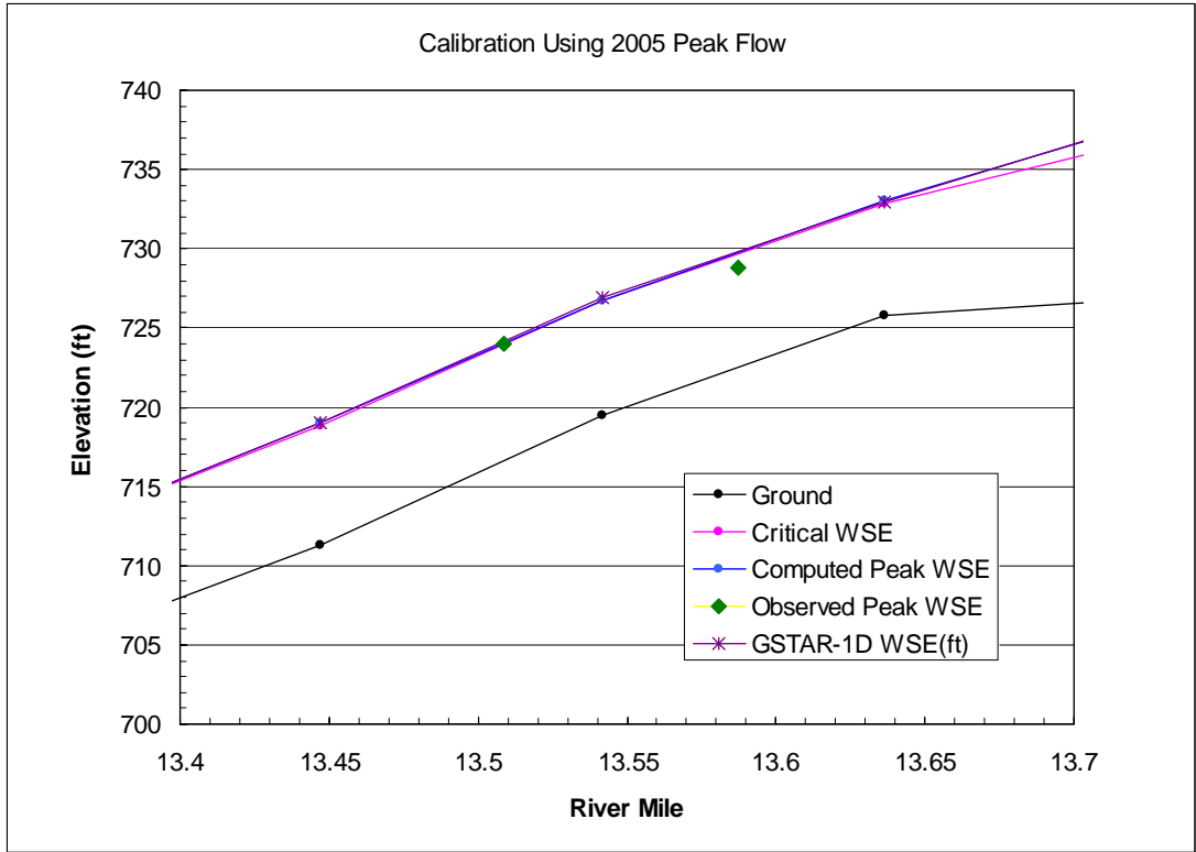
Figure 4.5. Plot of observed and computed peak water surface elevations just downstream of Robles Diversion.
