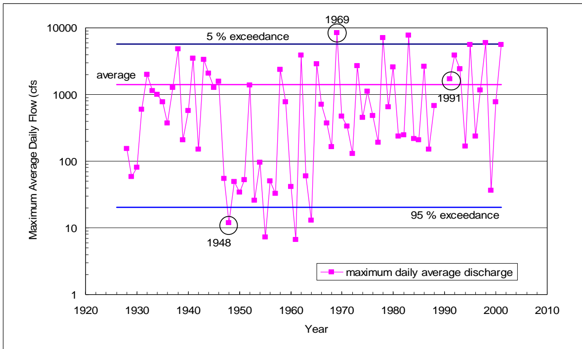
Figure 2.10. Analysis of maximum daily average flows at USGS gage 11115500, downstream of Matilija Dam on Matilija Creek.
