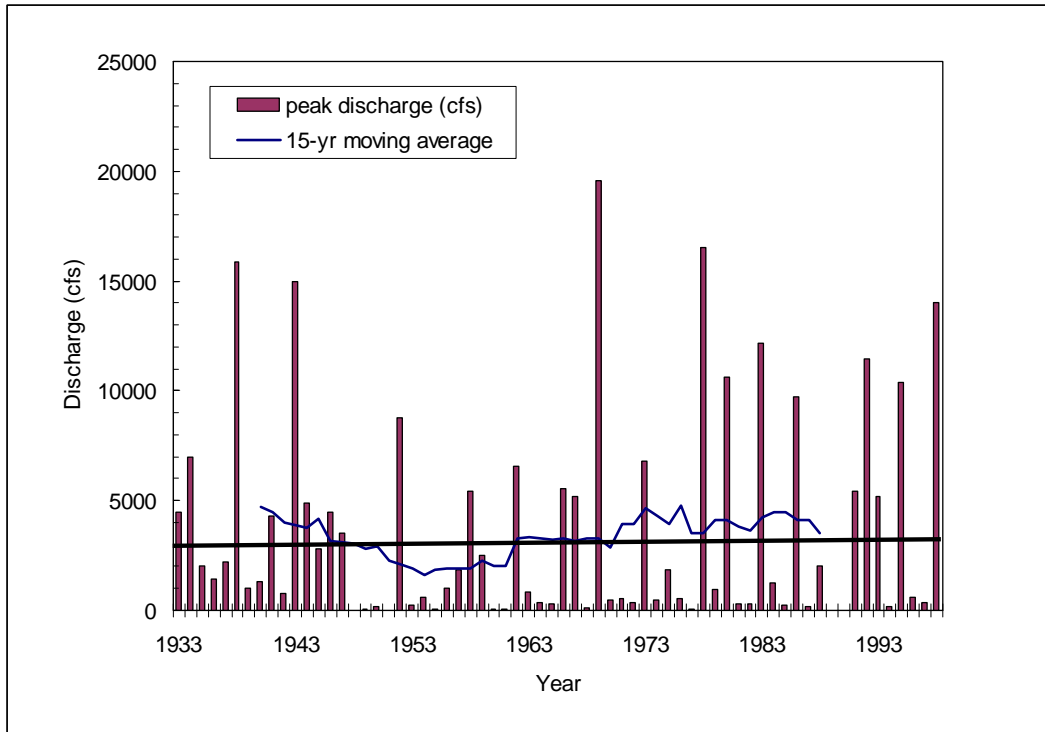
Figure 2.3. Peak Discharge at USGS gage 11115500, downstream of Matilija Dam on Matilija Creek. Flows between Oct 1 1988 and Sept 30 1990 were not available at this gage
