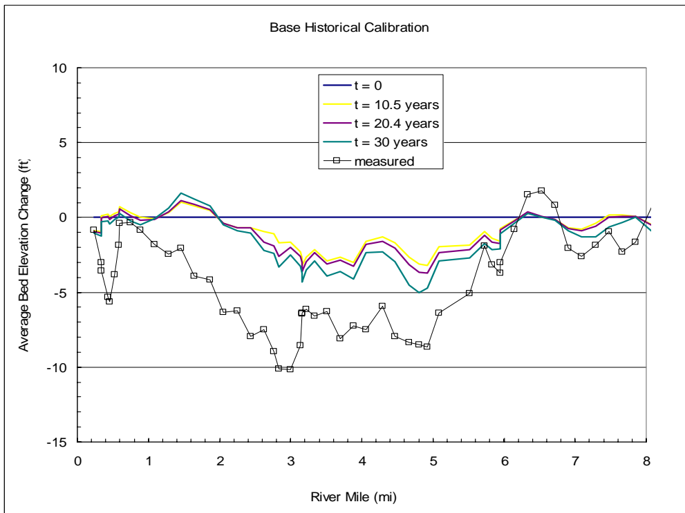
Figure 6.19. Computed Average Bed Elevation Change from 1971 to 2001, RM 0 – 8.
