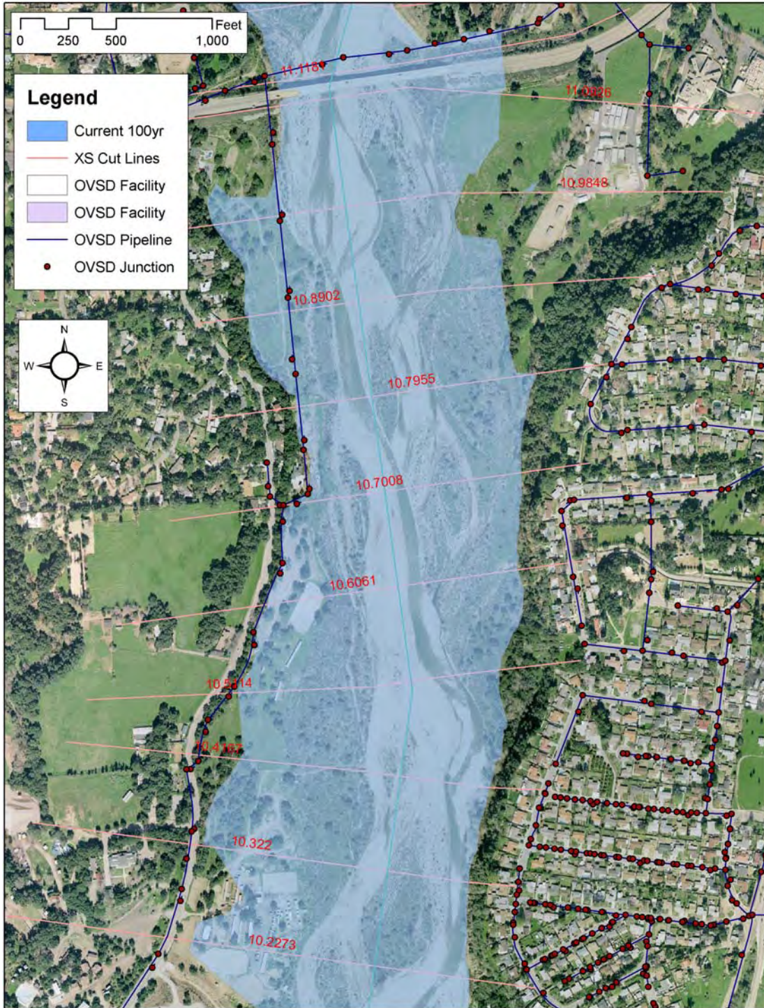
Figure 4.10. 100-yr floodplain from RM 11 to RM 10 Showing location of OVSD pipelines.
