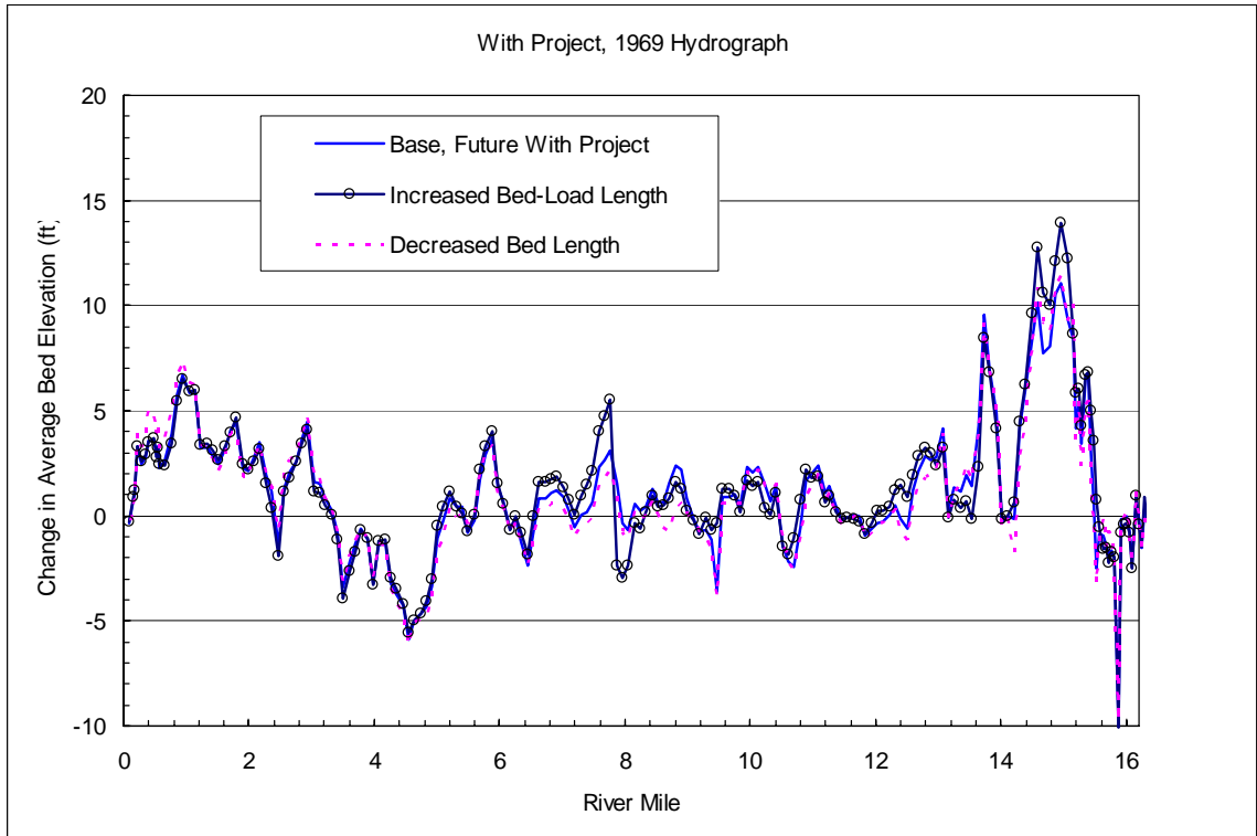
Figure 12.12. Affect of Bed Load Adaptation Length on Average Bed Elevations for 1969 Hydrograph.
