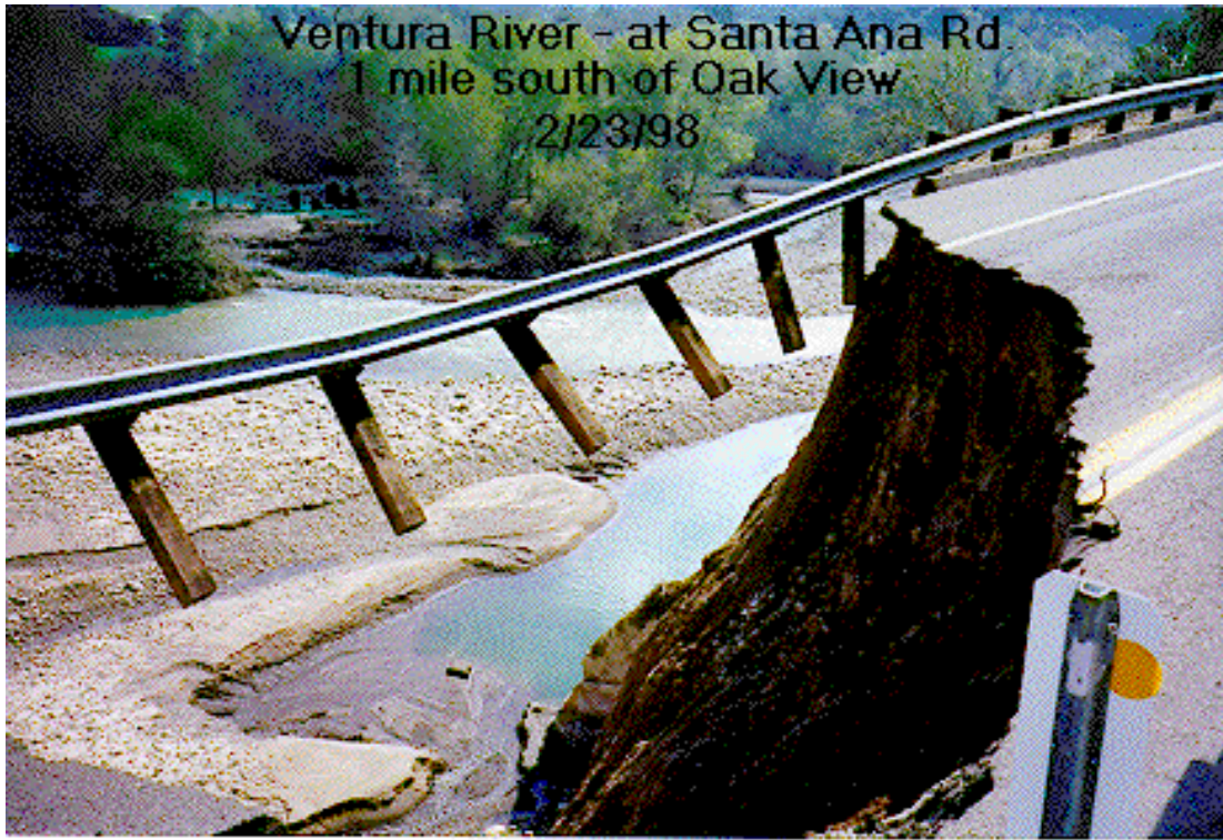
Figure 4.16. Picture of the looking downstream at the Ventura River from the East Abutment of Santa Ana Bridge. Picture was taken after the 1998 flood on 2-23-1998.
