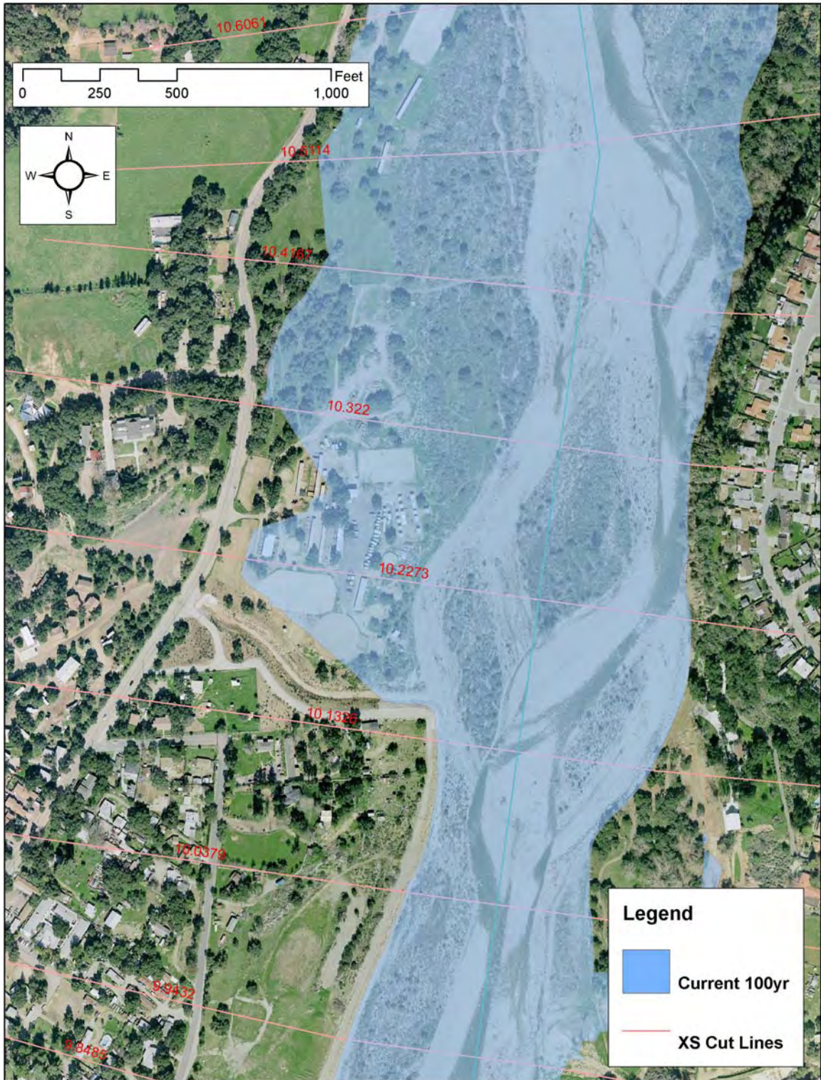
Figure 4.11. 100-yr Floodplain in Vicinity of Live Oak Drain.
