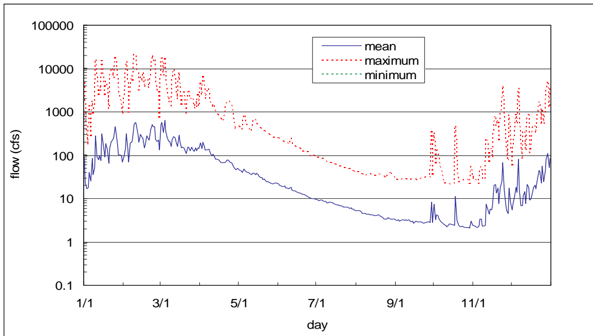
Figure 2.6. Mean, Maximum, and Minimum Daily Average Discharges for Every Day of the Year at USGS gage 11118500, Ventura River at Foster Park.
