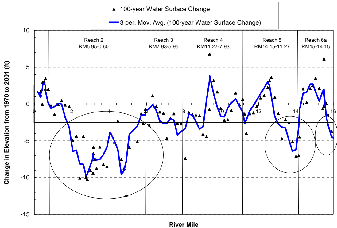
Figure 5.32. Comparison of change in 100-year flood stage between 2001 and 1970. Negative changes indicate areas where the flood stage has lowered. Positive changes indicate areas where the flood stage has increased. Areas within 2.5 feet of change are considered to be within the error range of the 1970 data.
