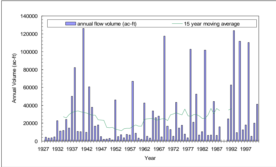
Figure 2.7. Annual flow volume at USGS gage 11115500, downstream of Matilija Dam on Matilija Creek.
