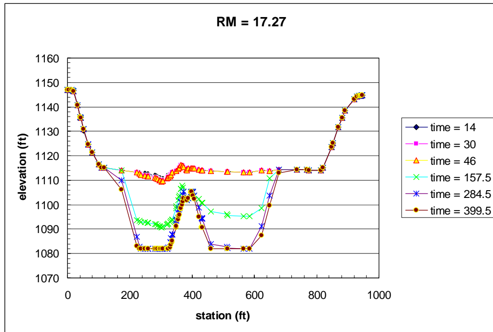
Figure 6.16. Example of Cross Section in Upstream Delta for Alternative 2a for Two 100-yr Floods in Succession.
