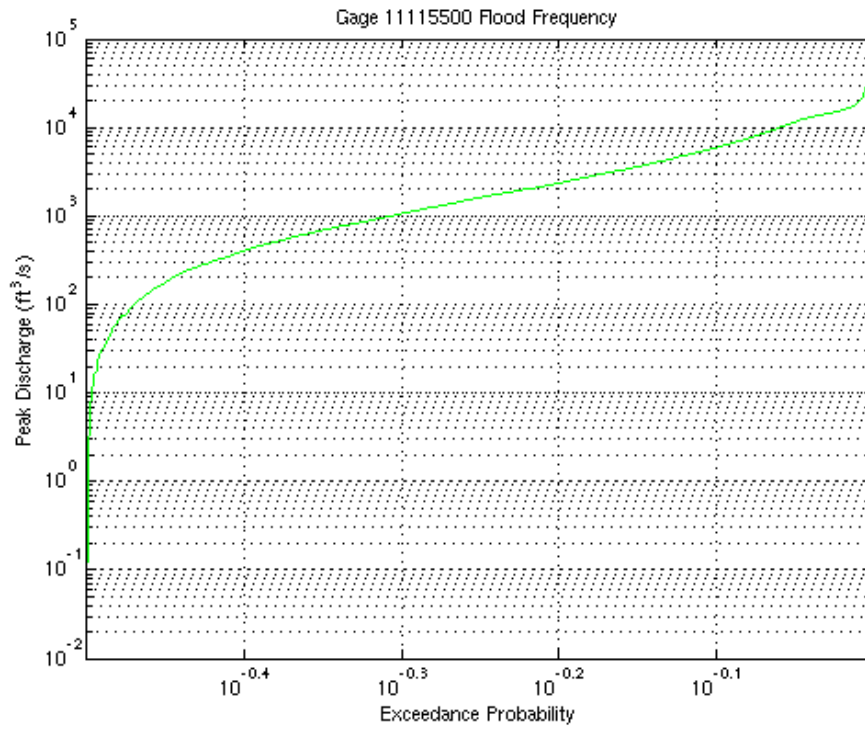
Figure 6.6. Flood Frequency curve for gage 11115500 used in stochastic simulations.
