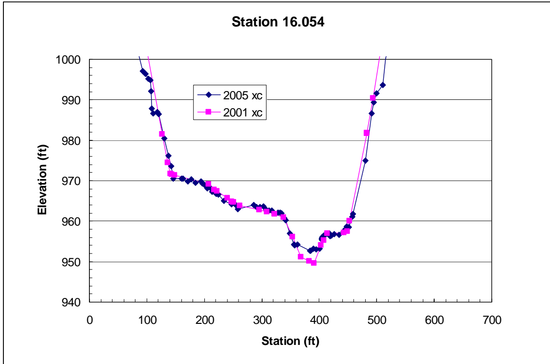
Figure 4.2. Comparison between 2001 and 2005 aerial surveys at Station 16.054.
