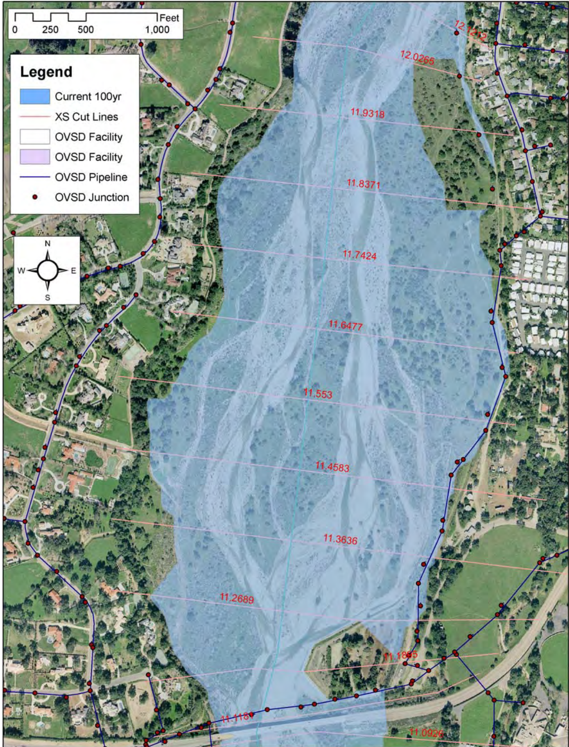
Figure 4.8. 100-yr floodplain from RM 12 to RM 11. Showing location of OVSD pipelines
