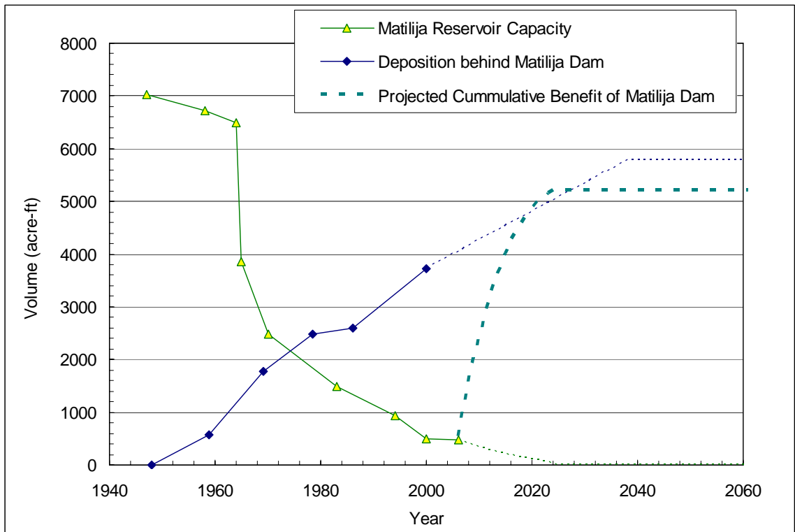
Figure 8.1. Storage Capacity of Matilija Reservoir and Projected Benefit of Matilija Dam to the Amount of Water Diverted at Robles.
