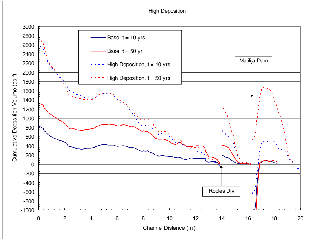
Figure 12.6. Sensitivity of Volume of Sediment Deposition to Incoming Sediment Loads.
