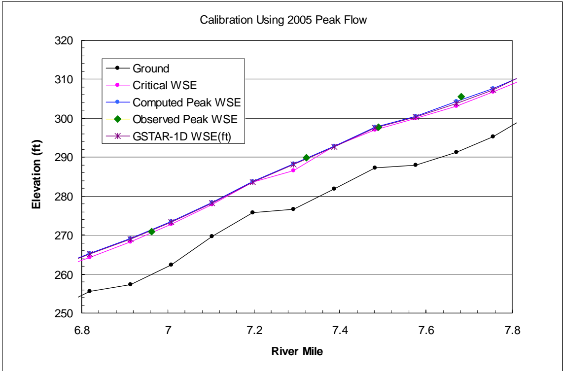
Figure 4.3. Plot of observed and computed peak water surface elevations at the Levee near Casitas Springs.
