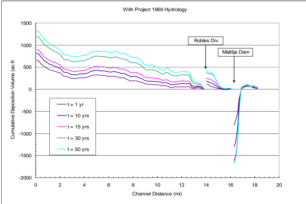
Figure 11.20. Cumulative Deposition for 1969 historical 50-yr hydrograph for With- Project Conditions.
