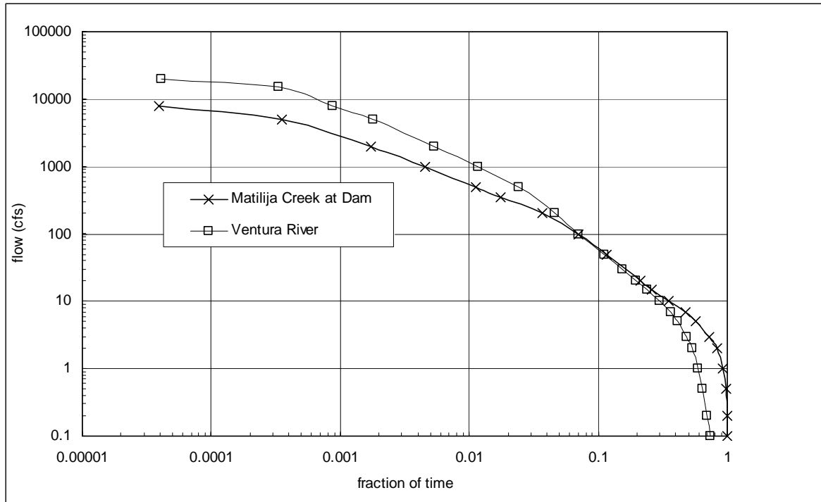
Figure 2.11. Plot of flow duration curves for USGS gage 11115500 at Matilija Dam and USGS gage 11118500, near Foster Park on the Ventura River.
