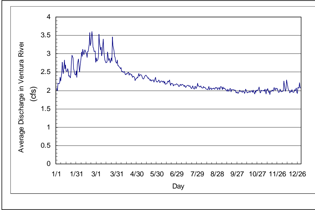
Figure 1.14. Average Discharge of the OVSD Wastewater Treatment Plant for Each Day of the Year.
