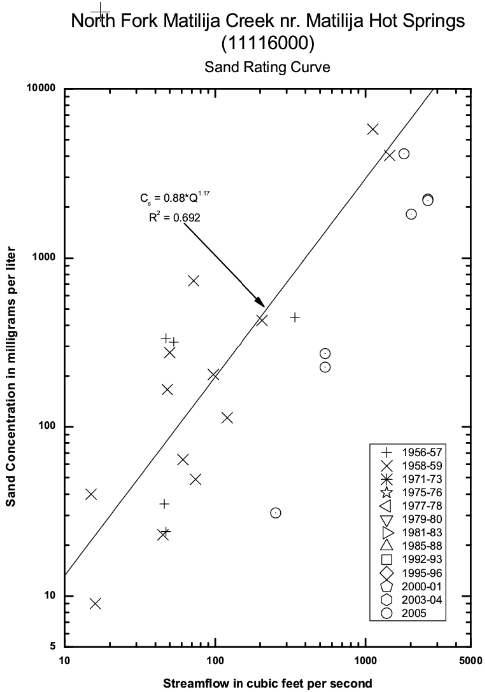
Figure 5.17. Sand Concentration on North Fork Matilija Creek.
