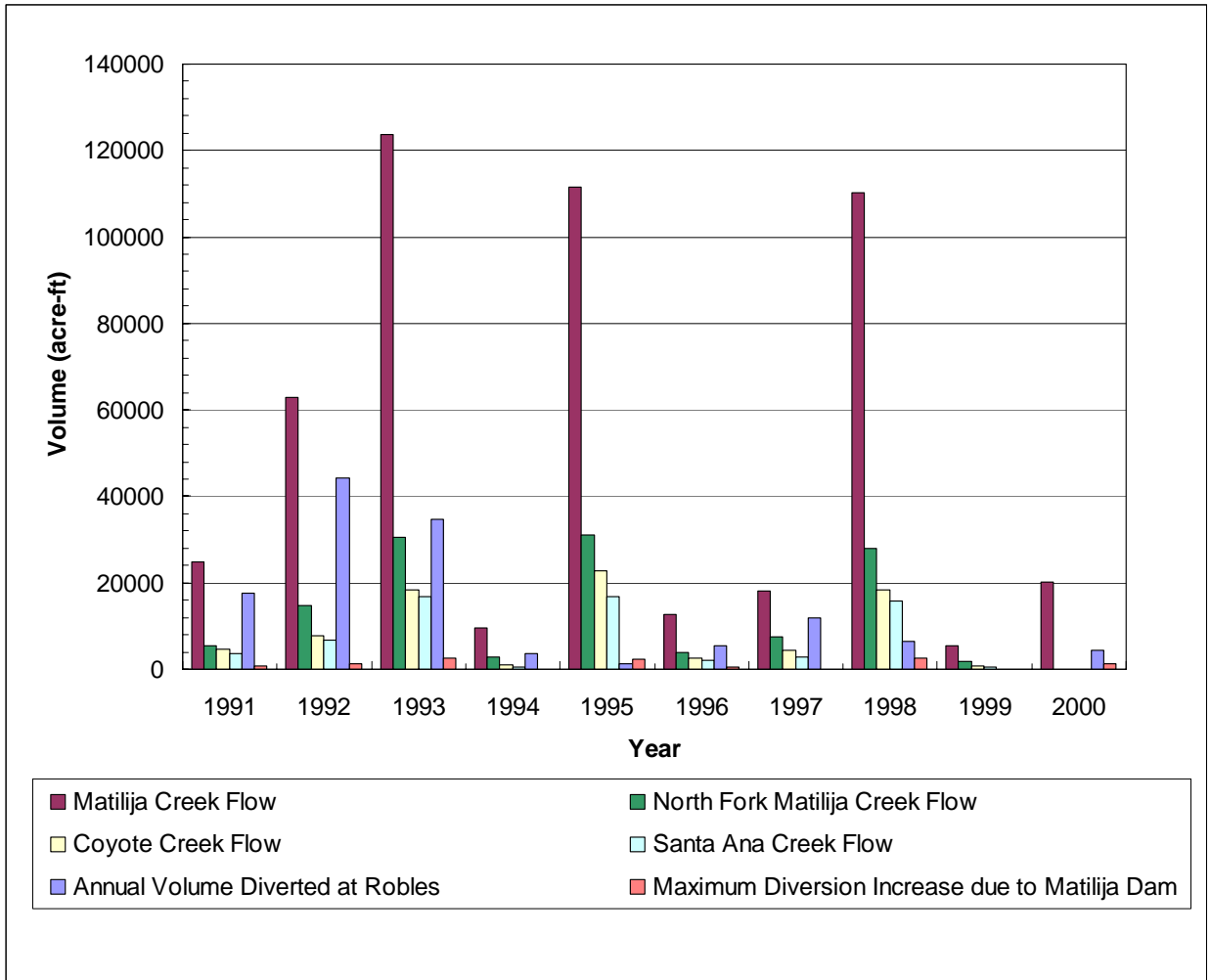
Figure 2.13. Annual Flow and Diversion Volumes for Period 1991 to 2000.
