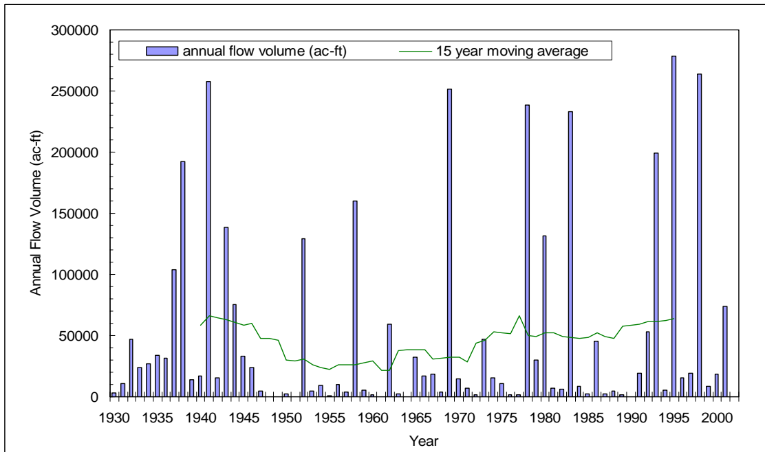
Figure 2.8. Annual flow volume at USGS gage 11118500, near Foster Park on the Ventura River.
