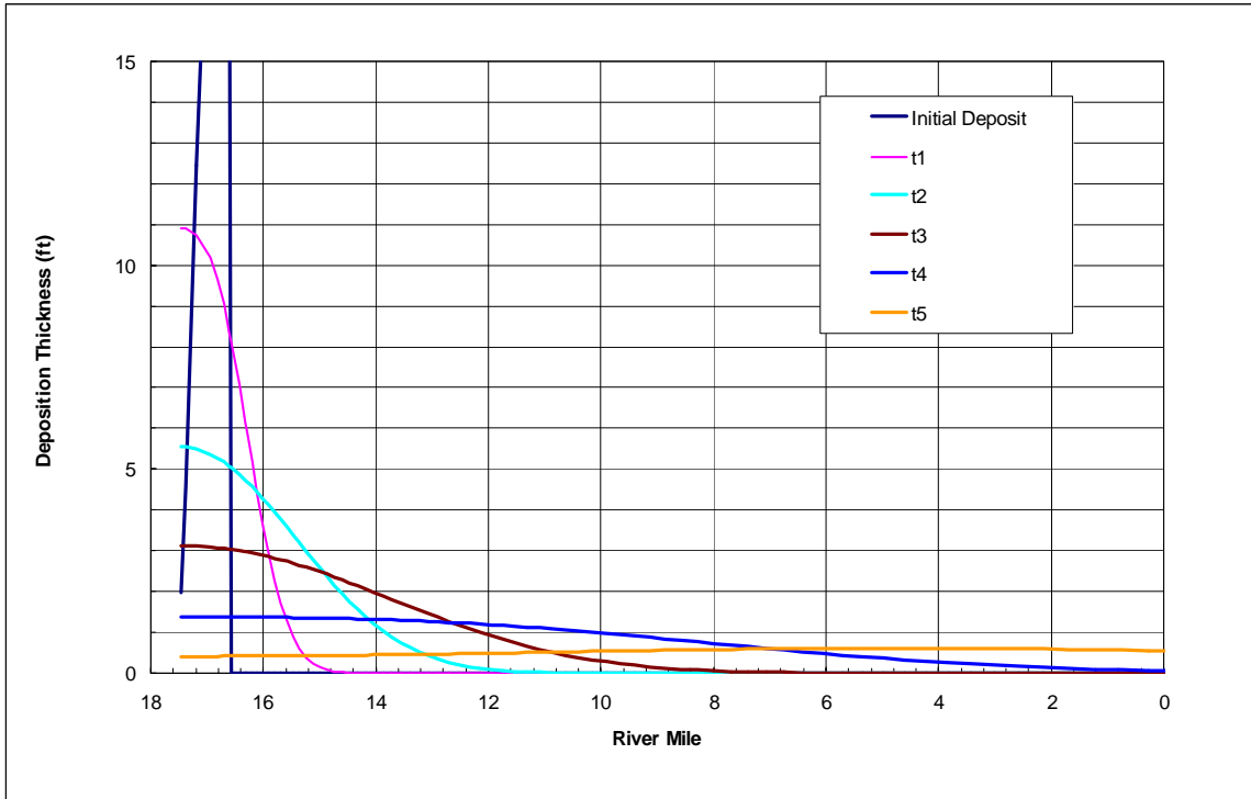
Figure 12.2. Simulation of Deposition Thickness using Sediment Wave Model.
