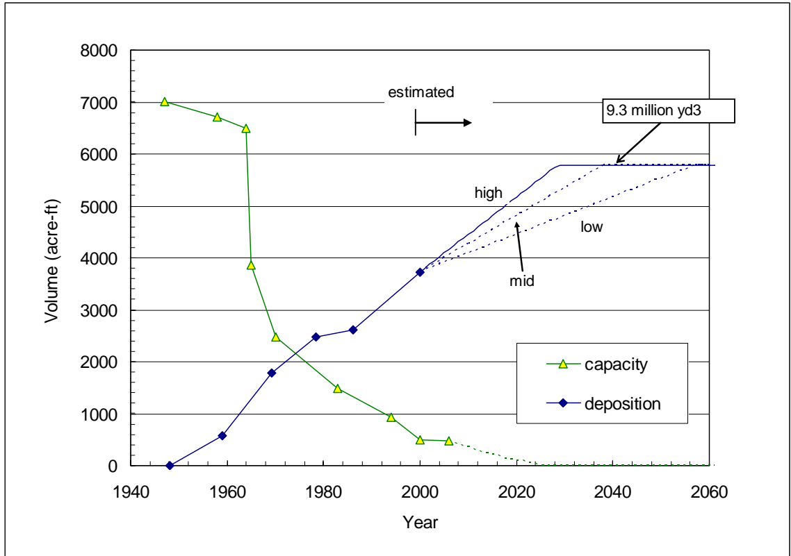
Figure 11.1. Historical and projected future deposition in Matilija reservoir.
