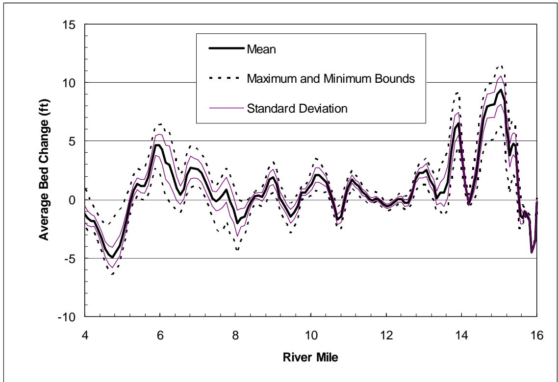
Figure 12.3. Average Bed Deposition for the Range of Stochastic 50-yr Hydrographs under With-Project Conditions
