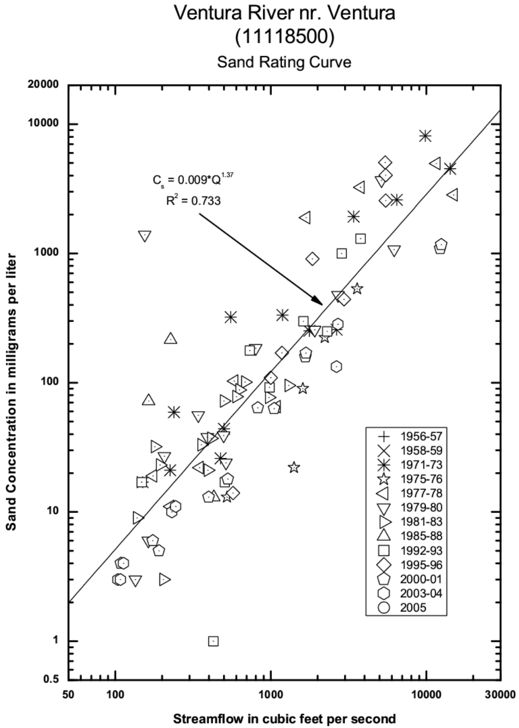
Figure 5.23. Sand Concentration on Ventura River at Foster Park.
