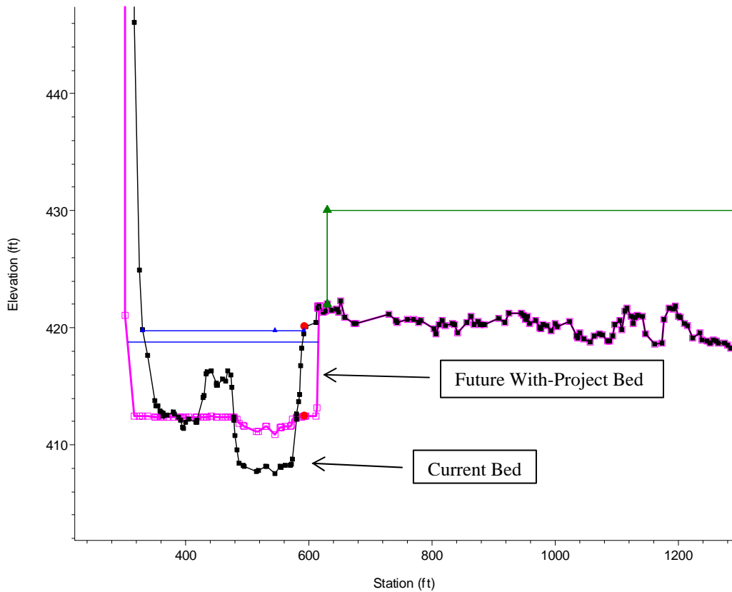
Figure 11.22. Bed Elevation Changes upstream of Santa Ana Bridge under With-Project Conditions.
