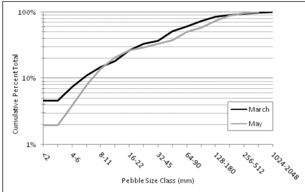
Figure 15. The results of two pebble counts on the channel bed of the Conococheague Creek ( Bravo reach) are graphed in a logarithmic format. The bed material of the Bravo reach was quantified based on a pebble count (Wolman 1954).
