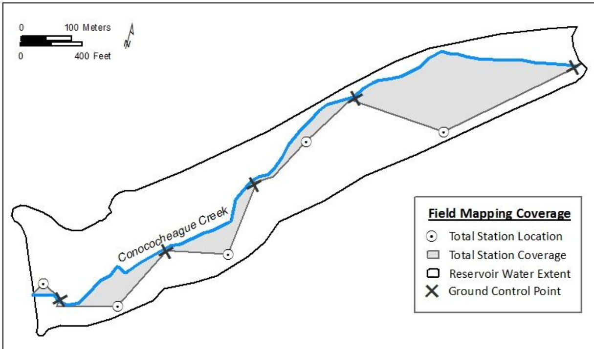
Figure 5. A graphic display of the methods employed to map the planform of the Conococheague Creek. Total station locations were mapped first with a GPS receiver then from the next nearest total station location. The ground control points were distributed to provide overlap between total station locations in an effort to minimize error.
