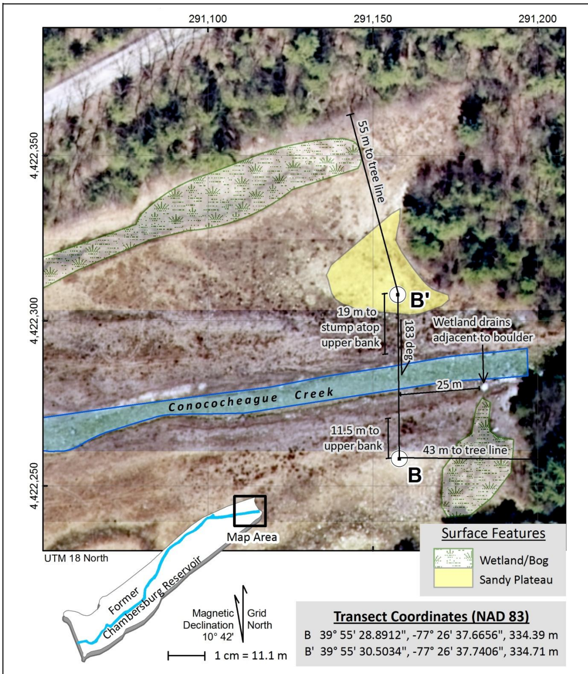
Figure 4a. The location of the Bravo transect is identifiable based on its spatial relationship with the relict shorelines of the former Chambersburg Reservoir and the Conococheague Creek. Map features are projected and the grid is displayed with the Universal Transverse Mercator (UTM) system, 18 North.
