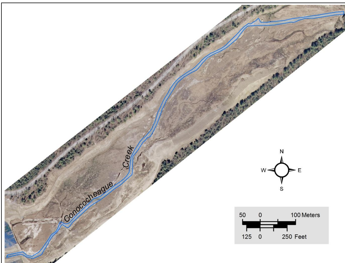
Figure 8. Stream planform of the Conococheague Creek through the former impoundment behind Birch Run Dam. Channel boundaries were mapped in the fall of 2008. There is no change to the channel planform compared to an aerial image taken in 2005 (PA DCNR 2008).
