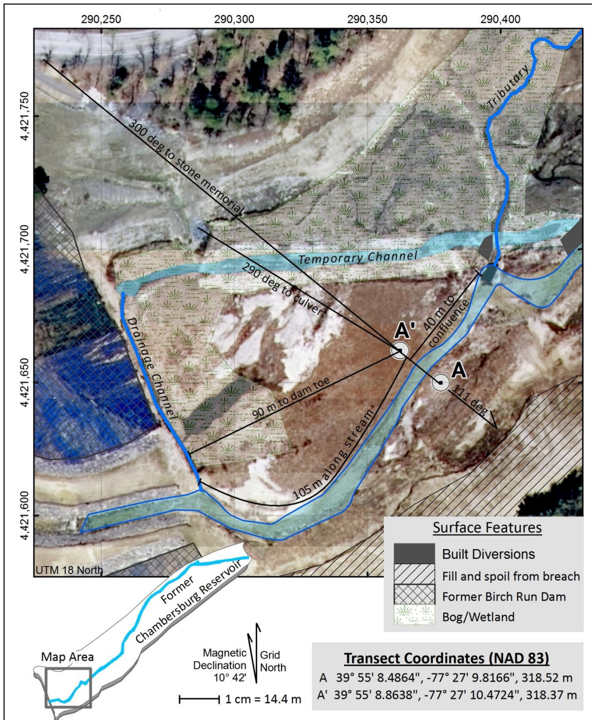
Figure 3a. The location of the Alpha study reach as relates to the former Birch Run Dam and other physical features. Map features are projected and the grid is displayed with the Universal Transverse Mercator (UTM) system, 18 North.
