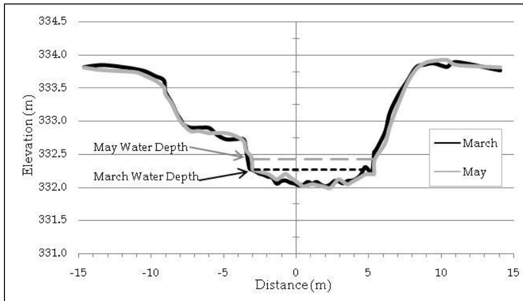
Figure 12. Comparison of the Bravo channel cross-sections observed during two field visits (March and May 2009) to the Conococheague Creek.
