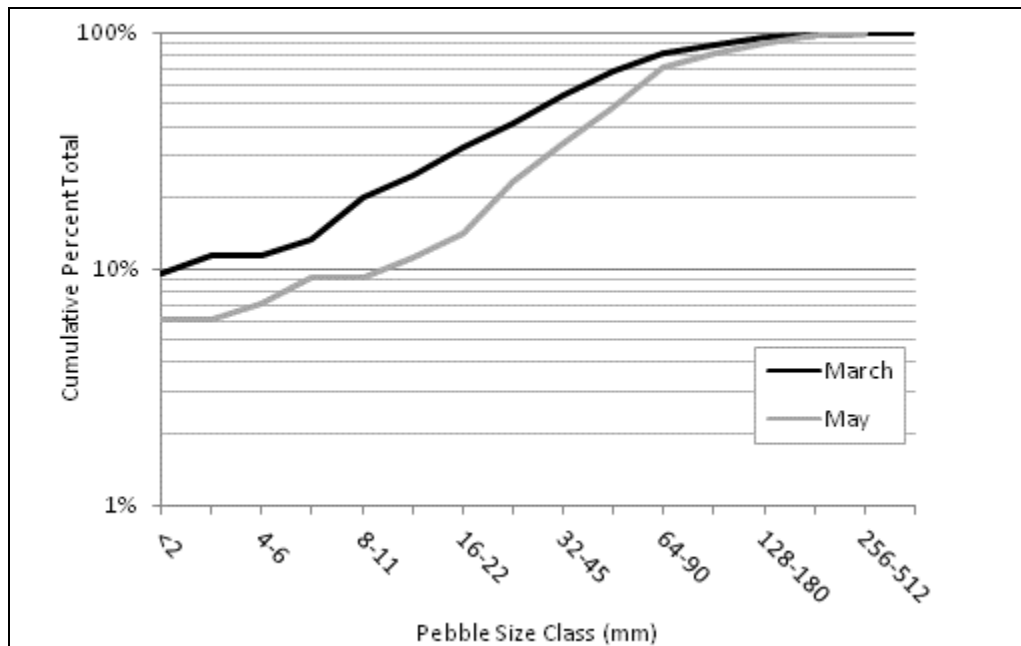
Figure 11. The results of two pebble counts on the channel bed of the Conococheague Creek ( Alpha reach) are graphed in a logarithmic format. The bed material of the Alpha reach was quantified based on a pebble count (Wolman 1954).
