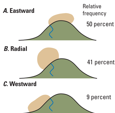
Figure 9.6. Schematic diagrams showing the behavior of the buoyant coastal plume of the Elwha River, Washington. (After Warrick and Stevens, 2011). The plume is bent toward the east (A) and west (C) during strong tidal currents, and is radial (B) during weak currents. Oceanographic observations suggest that the plume is bent toward the east more frequently than toward the west.
