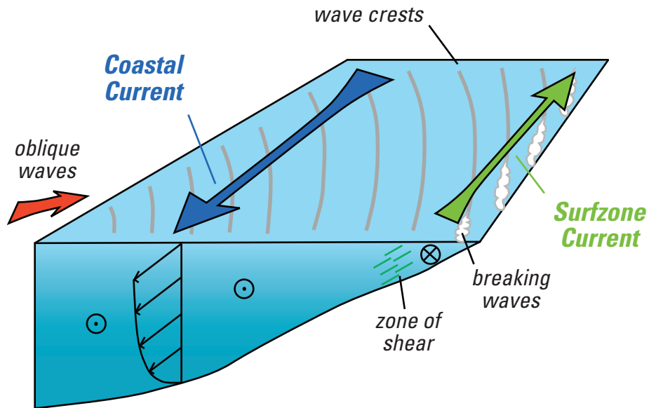
Figure 5.2. Schematic diagram showing alongshore currents of nearshore waters. Surfzone currents (green arrow) are caused by breaking waves when they have oblique approach angles. The coastal currents (blue arrow) offshore of the surfzone are influenced by tidal, wind-driven, or other regional currents and may or may not be in the same direction as the surfzone currents.
