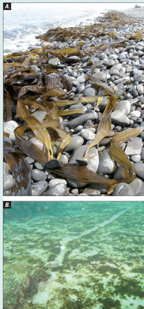
Figure S5.3. Examples of kelp-mediated clast movement from the Elwha River delta, Washington, coastal zone. (A) Numerous kelp-attached clasts litter the beach on June 21, 2009, about 250 meters east of the river mouth. Water level in this photograph is estimated to be 1.0 meter above Mean Lower Low Water (MLLW). The dominant kelp in these windrows is Cymathere triplicata , a common kelp at depths between -3.0 and -8.0 meters offshore of the delta. The two kelp-attached clasts in the near-field are estimated to be 5 centimeters along their long axes. (B) Active movement of an unidentified kelp attached to a cobble through algal debris at about -5.0 m MLLW depth offshore of the base of Ediz Hook on August 11, 2008. The clast under motion in this photograph is estimated to be 15 centimeters along the long axis. (Photographs taken by Ian Miller, University of California, Santa Cruz.)
