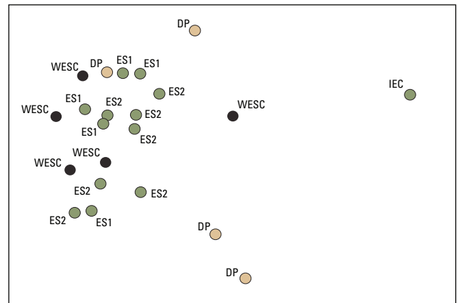
B. July nMDS (stress = 0.13)
