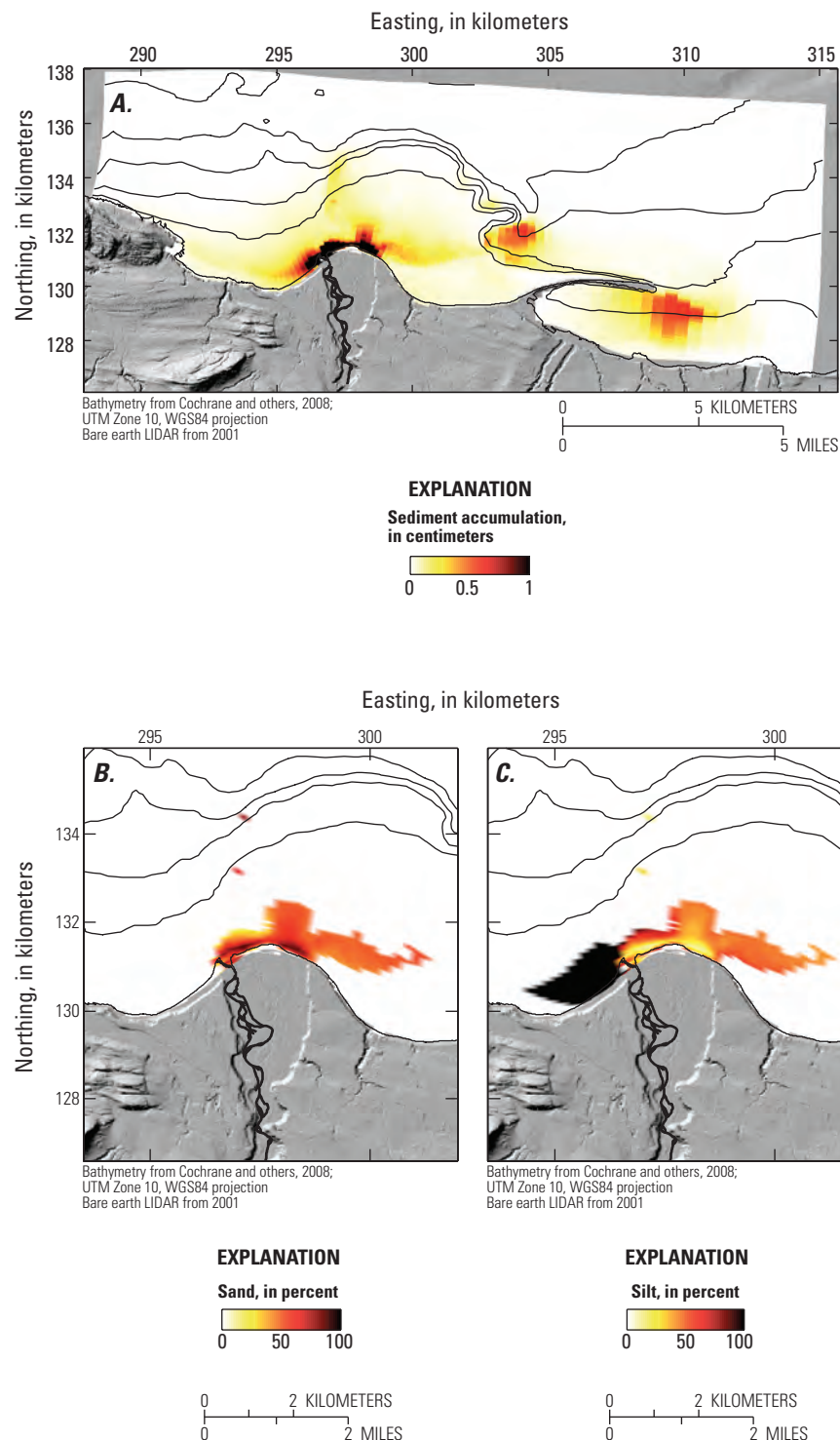
Figure 9.7. (A) simulated sediment accumulation offshore of the Elwha River mouth, Washington, after flood event from the river. (After Gelfenbaum and others, 2009). Results derived from a three-dimensional hydrodynamic model of water and two classes of sediment, sand, and silt. The sand (B) preferentially accumulates east of the river mouth, and the silt (C) accumulates on both sides of the river mouth.
