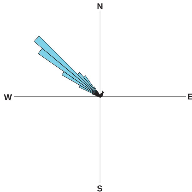
Figure 5.5. Rose diagram showing dominant wave direction from observations at the western side (site W) of the Elwha River delta, Washington. More than 90 percent of the observations were dominated by waves from the northwest, which is the direction of approach for waves generated in either the Pacific Ocean or the western Strait of Juan de Fuca.
