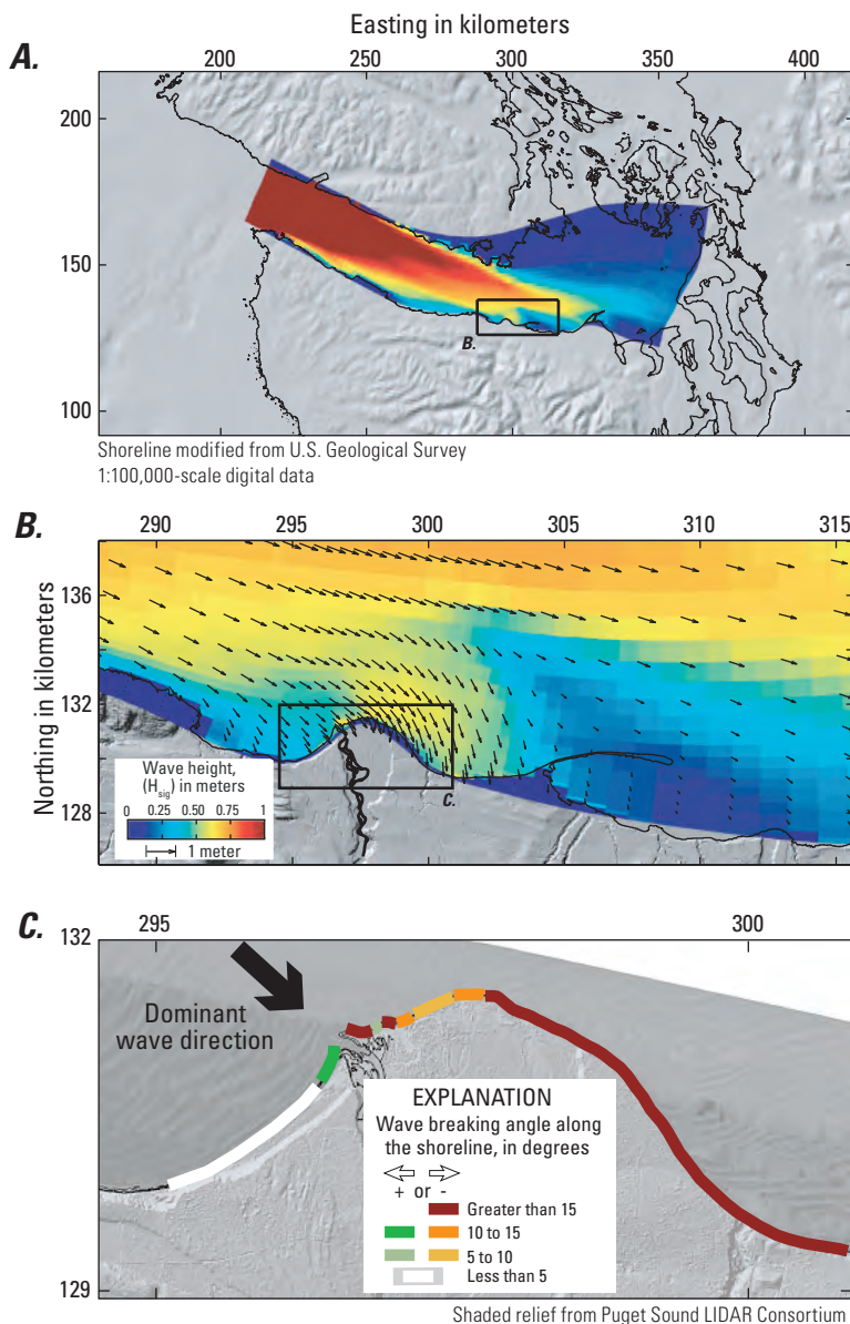
Figure 5.6. Wave patterns for the Strait of Juan de Fuca and Elwha River delta, Washington, from measurements and model simulation results. (A–B) The transformation of wave heights and directions in the Strait from 6 meter Pacific Ocean swell as predicted by the SWAN numerical model (after Gelfenbaum and others, 2009). Arrows in (B) show modeled wave directions. (C) Measurements of the angle of breaking waves along the Elwha River delta shoreline during northwest swell (black arrow) from lidar and aerial photographs (after Warrick and others, 2009).
