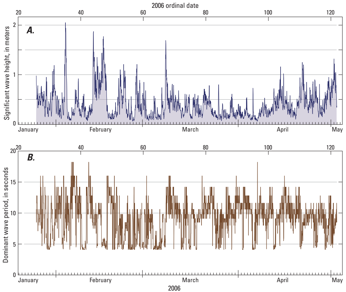
Figure 5.3. Wave height and wave period measurements from the western side (site W) of the Elwha River delta, Washington, during 2006.
