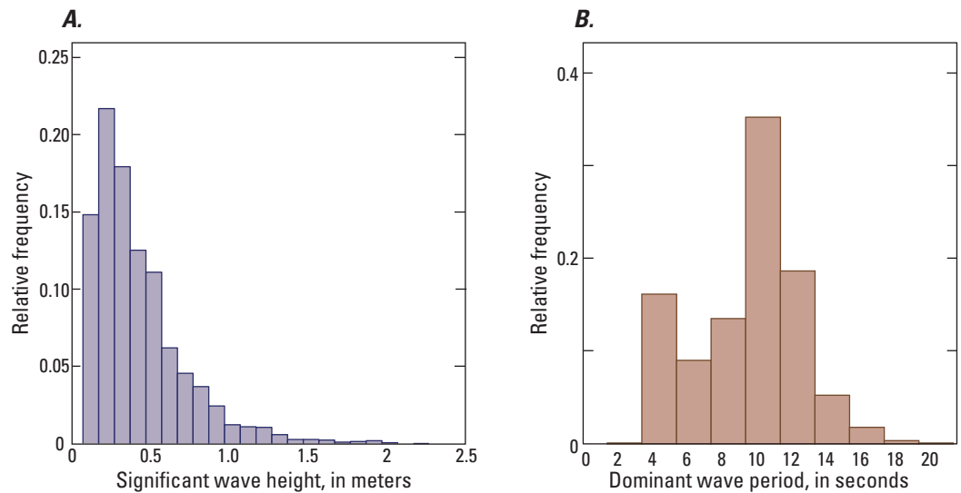
Figure 5.4. Histograms of significant wave height and dominant wave period from observations at the western side (site W) of the Elwha River delta, Washington. Waves generally are less than 1 meter with periods greater than 8 seconds, indicating Pacific Ocean origins. Location of site is shown in figure 5.1.
