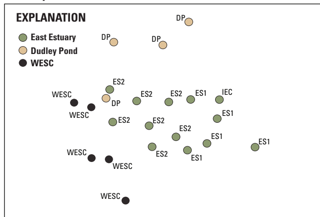
C. September nMDS (stress = 0.12)
