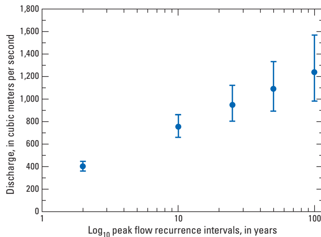
Figure 1.17. Weighted recurrence-interval peak flows calculated for the Elwha River at U.S. Geological Survey streamflow-gaging station 12045500, Elwha River at McDonald Bridge near Port Angeles, Washington, with the upper and lower 95 percent confidence intervals.
