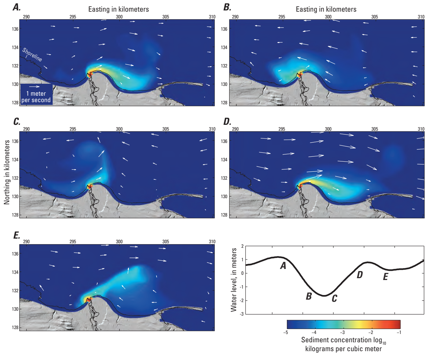
Figure 5.13. Evolution of coastal turbidity from the discharge of suspended sediment from the Elwha River, Washington, as determined by model simulation results (after Gelfenbaum and others, 2009). Arrows indicate depth-averaged flow direction and magnitude.
