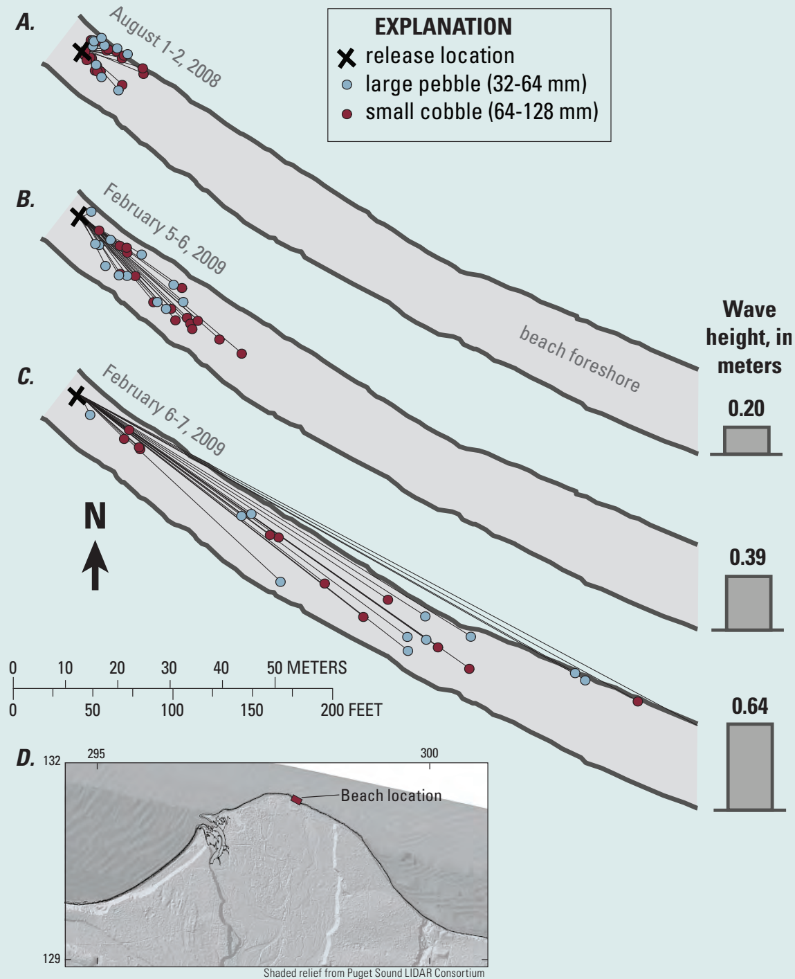
Figure S5.2. Diagrams and map showing examples of three 24-hour releases of the Radio Frequency Identifier tracers over a range of wave conditions, Elwha River delta, Washington. (A) August 1–2, 2008; (B) February 5–6, 2009; (C) February 6–7, 2009, (D) location of active foreshore and release site. Wave heights from visual estimates on August 1–2, 2008, and a pressure transducer located offshore of this site during the February 2009 measurements.
