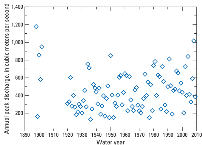
Figure 1.16. Annual peak discharges measured at U.S. Geological Survey streamflow-gaging station 12045500, Elwha River at McDonald Bridge near Port Angeles, Washington.
