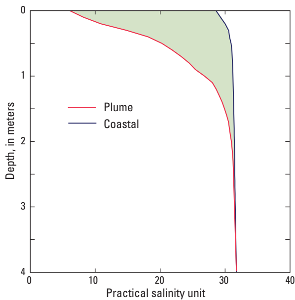
Figure 5.12. Salinity inside the buoyant plume (plume) and in coastal waters directly outside the plume (coastal), Elwha River, Washington. Measurements were taken at 1800 Pacific Standard Time on June 9, 2007, at about 0.5 kilometers offshore of the river mouth. The freshening of the upper 1.5 meters of water from the river water is shaded green. (After Warrick and Stevens, 2011.)
