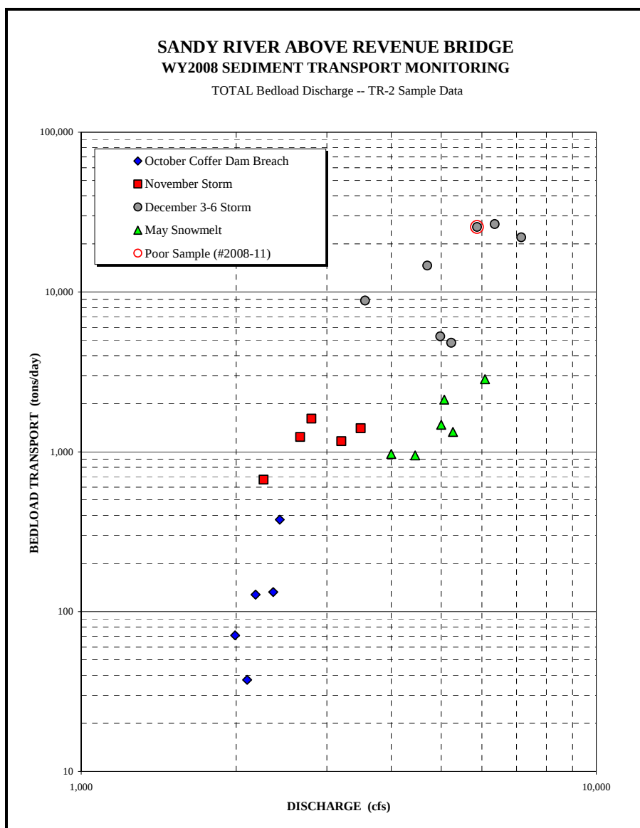
Figure 3-22. Composited bedload samples presented by sampling period.
