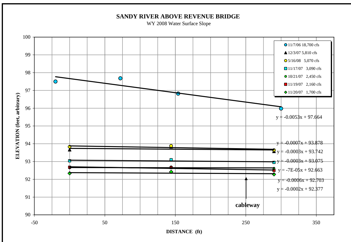
Figure 3-5. Water surface slope through the sampling section.
