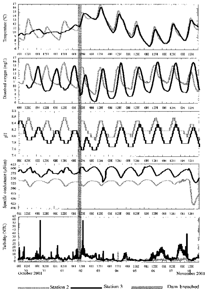
Figure 8.6 Continual measurements (15-minute intervals) of selected water quality constituents (partial record) at Stations 2 and 3. Note: mg/L = milligrams per liter; \mu\text{S}/\text{cm} = microsiemens per centimeter; NTU = Nephelometric Turbidity Units.
