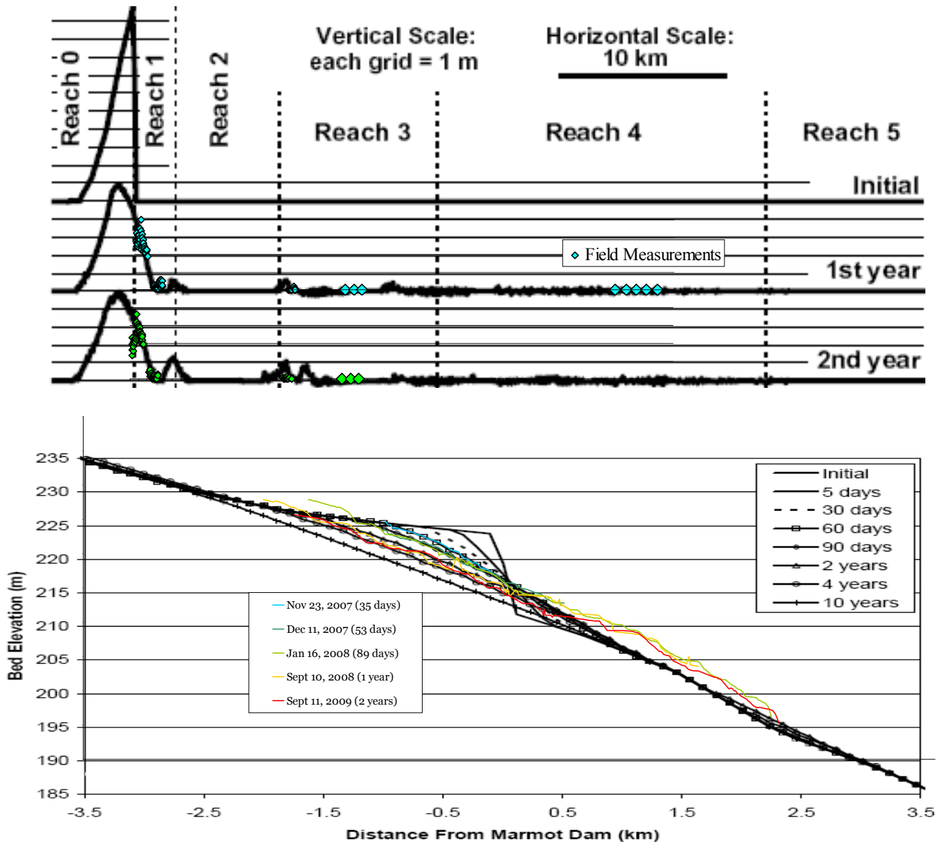
Figure 6 Results of numerical modeling from Cui and Wilcox (2008). Longitudinal profiles [averaged at a cross section] for a) annual change in bed elevation, and b) bed elevation
