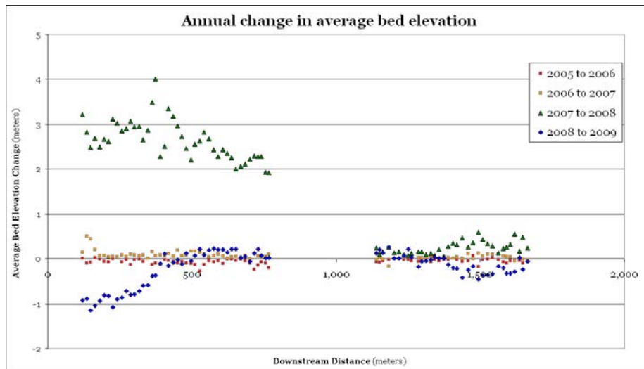
Figure 4 Longitudinal profiles [averaged at a cross section] for annual change in bed elevation
