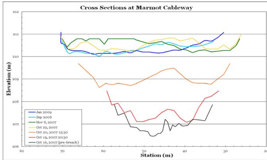
Figure 3 Repeat cross sections at the Marmot cableway. The aggrading channel bed is evident in this series. Note some erosion between September 2008 and January 2009.
