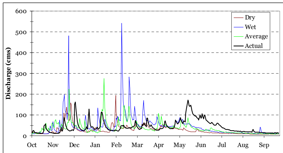
Figure 5 Hydrographs for discharge at the dam site - dry, wet, and average conditions used for the model inputs, as well as the actual daily discharge at USGS station 14136500.
