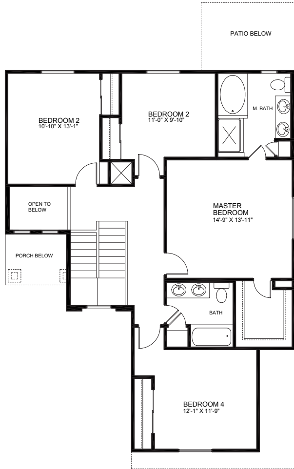
SECOND FLOOR PLAN 1053 S.F.
