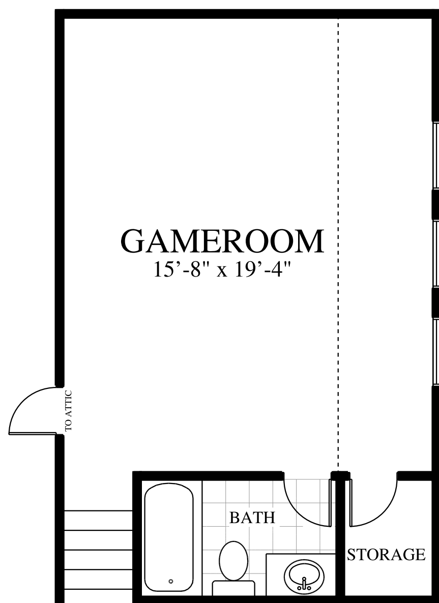
SECOND FLOOR GAMEROOM 400 S.F.
